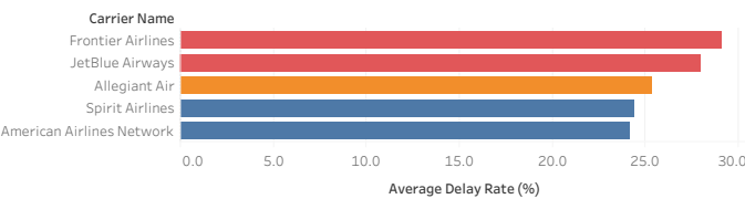
Top-5 Carriers by Delay Rate
