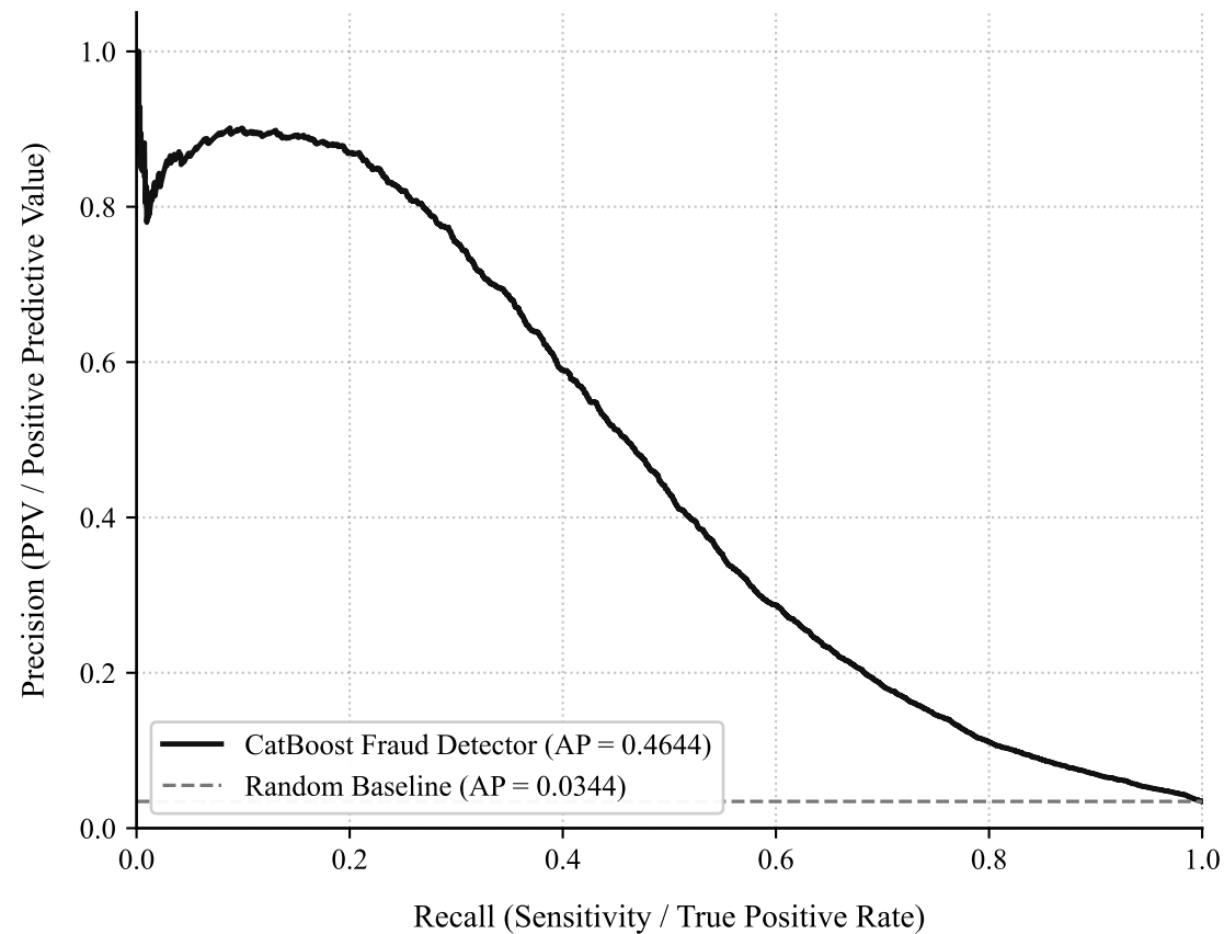
Sentinel AI: Precision-Recall (PR) Curve
