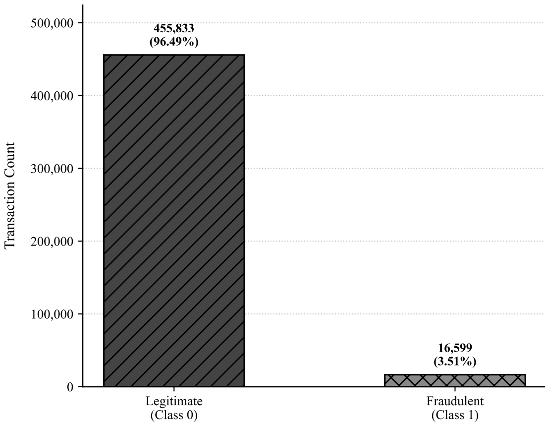
IEEE-CIS Dataset: Class Distribution & Imbalance
