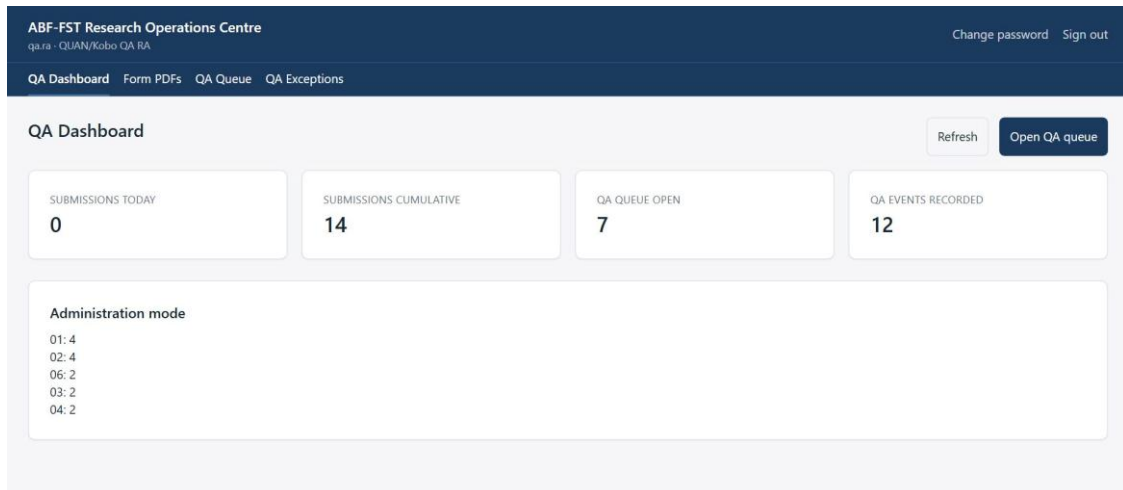
Figure 4. QA Dashboard.
