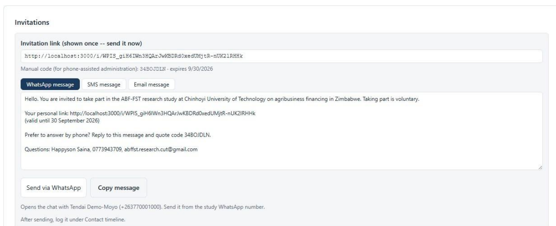
Figure 19. The link, manual code and ready-written messages are shown once, with a send button for each channel.
