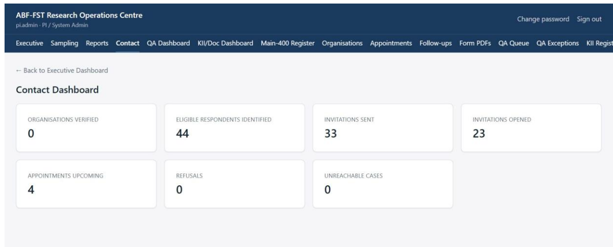
Figure 6. Contact Dashboard.
