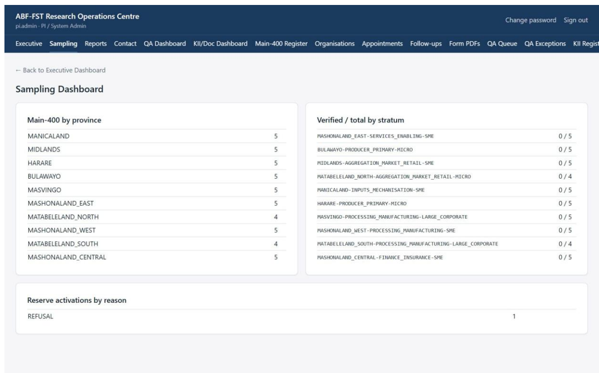
Figure 5. Sampling Dashboard.
