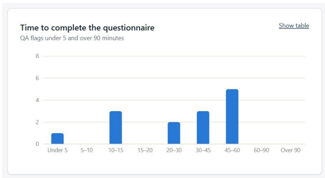
Figure 21. Completion-time distribution.
