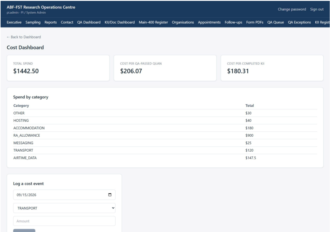
Figure 32. Cost Dashboard and the Log a cost event form.
