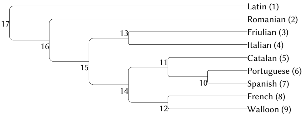
Fig 1. An example tree showing the relationships of N = 9 languages.
