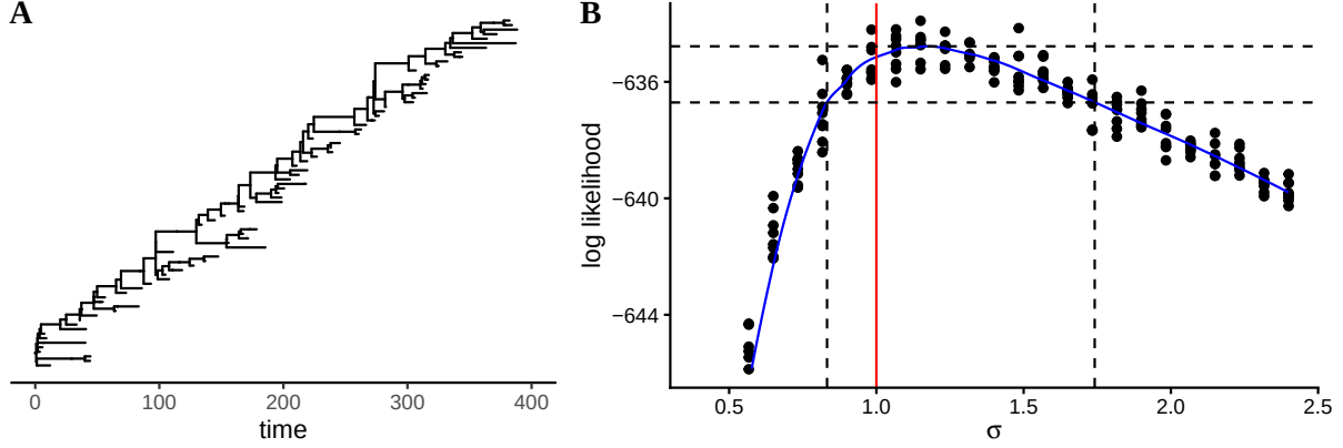
Figure 9. Likelihood computation for the SEIRS model by sequential Monte Carlo, using the scheme of §B4. (A) Simulated genealogy for \beta = 3 , \sigma = 1 , \gamma = 0.5 , \psi = 0.02 , \omega = 0.08 , (S_0, E_0, I_0, R_0) = (70, 1, 0, 50) . (B) Likelihood slice in the \sigma -direction. Each point represents the estimate of an independent sequential Monte Carlo computation. The blue curve shows a LOESS smooth; the dashed vertical lines enclose the Monte Carlo-adjusted 95% confidence interval (Ionides et al., 2017).
