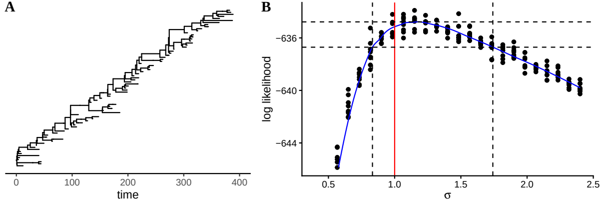
Figure 8. Likelihood computation for the SEIRS model by sequential Monte Carlo, using the scheme of §B4. (A) Simulated genealogy for \beta = 3 , \sigma = 1 , \gamma = 0.5 , \psi = 0.02 , \omega = 0.08 , (S_0, E_0, I_0, R_0) = (70, 1, 0, 50) . (B) Likelihood slice in the \sigma -direction. Each point represents the estimate of an independent sequential Monte Carlo computation. The blue curve shows a LOESS smooth; the dashed vertical lines enclose the Monte Carlo-adjusted 95% confidence interval (Ionides et al., 2017).
