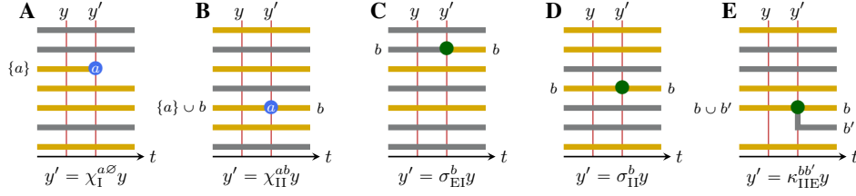
Figure 7. Chop, swap, and fork operators. Each panel shows the local structure in the vicinity of an event. There are two demes, \{E, I\} , denoted by grey and yellow, respectively. In each case, y denotes the coloring (mapping of branches to demes) just before the event; y' denotes the coloring at the event. In (A), the sample labeled a (blue dot) terminates the branch, \{a\} , that bears only that lineage. Symbolically, we write y' = \chi_I^{a\emptyset} y . In (B), the sample labeled a is inline: the branch labeled b descends from it. The branch immediately ancestral to a is therefore \{a\} \cup b . Here, the color does not change at the sample event. Therefore y' = \chi_{II}^{ab} y . In (C), an event (green dot) occurs on branch b and the color changes from E to I. Symbolically, then, y' = \sigma_{EI}^b y . Panel (D) shows an event without an associated change in color. We denote this change with the notation y' = \sigma_{II}^b y . In this case, observe that while d(y') = d(y) , m(y') = 1 \neq 0 = m(y) , whence y' \neq y . In (E), a branch event occurs at the green dot, splitting the branches b, b' from their parent branch b \cup b' . In this case, b \cup b' and b are both in I and b' is in E, whence we write y' = \kappa_{II E}^{bb'} y .
