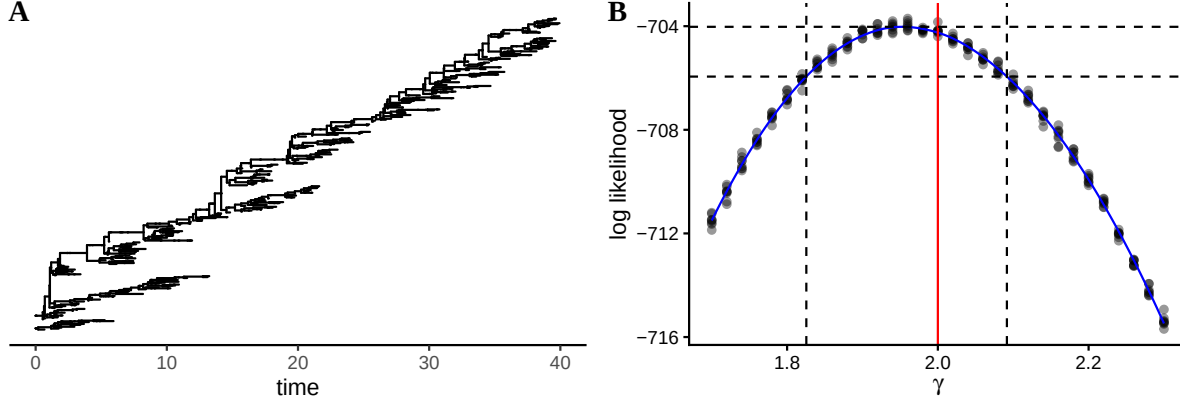
Figure 8. Likelihood computation for the SIRS model by sequential Monte Carlo.
