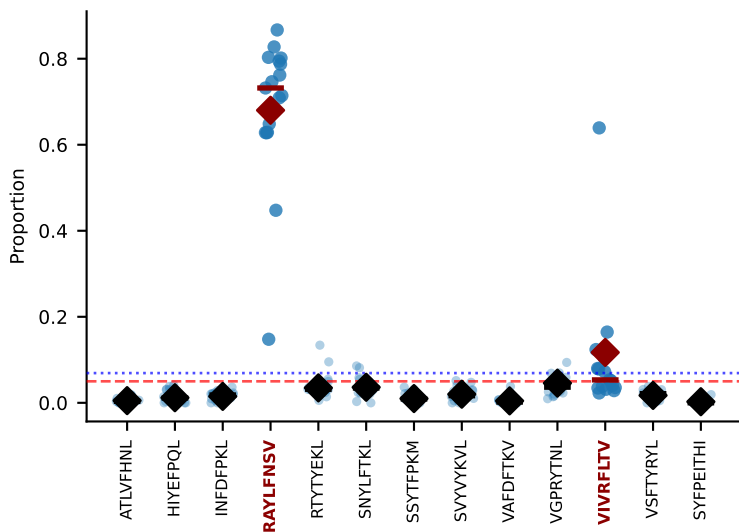
#113 AV6-6-CALGTFSNTDKVVF-AJ34*p03_BV13-1-CASSDVRDSGNTLYF-BJ1-3 DUAL | Above BG: RAYLFNSV+VIVRFLTV n=17 [HTxC:17] thresh=0.069
