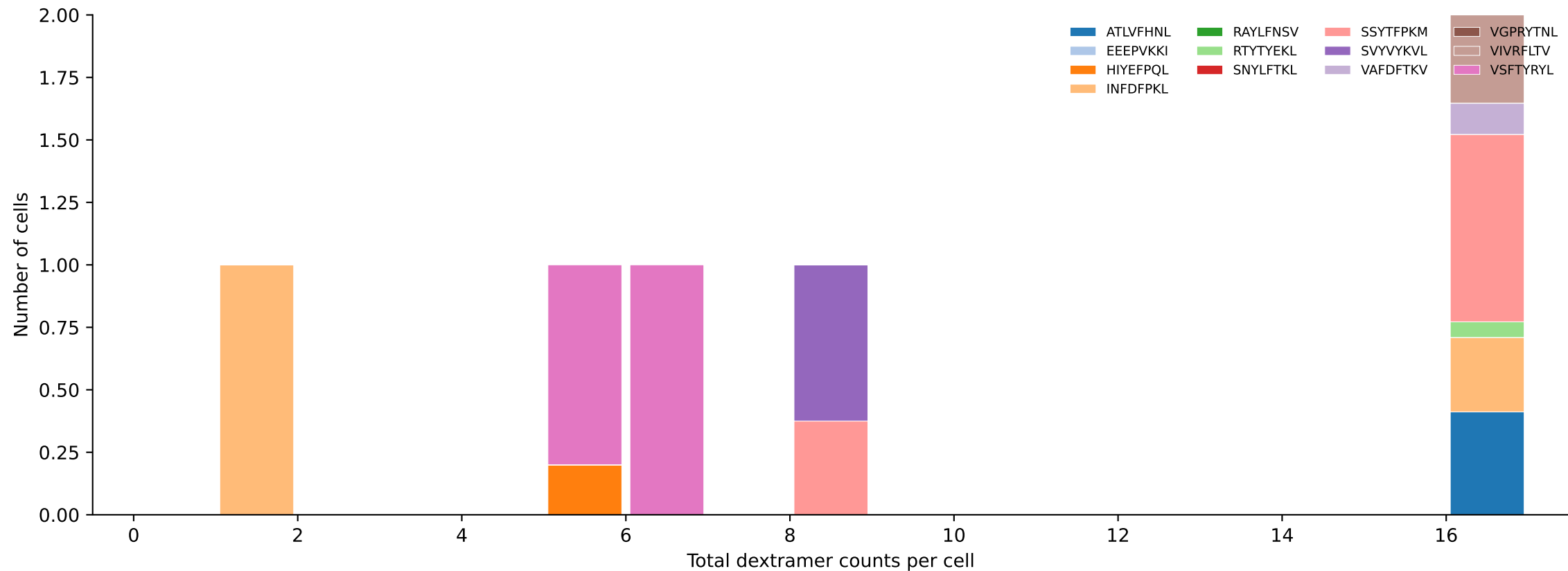
D7ABC_LL Combined | #375 AV8N-2-CATPNYNVLYF-AJ21_BV3-CASSLLGEYEQYF-BJ2-7 (n=6) Total pMHC histogram — stacked by mean peptide proportion per bin [375/392]
