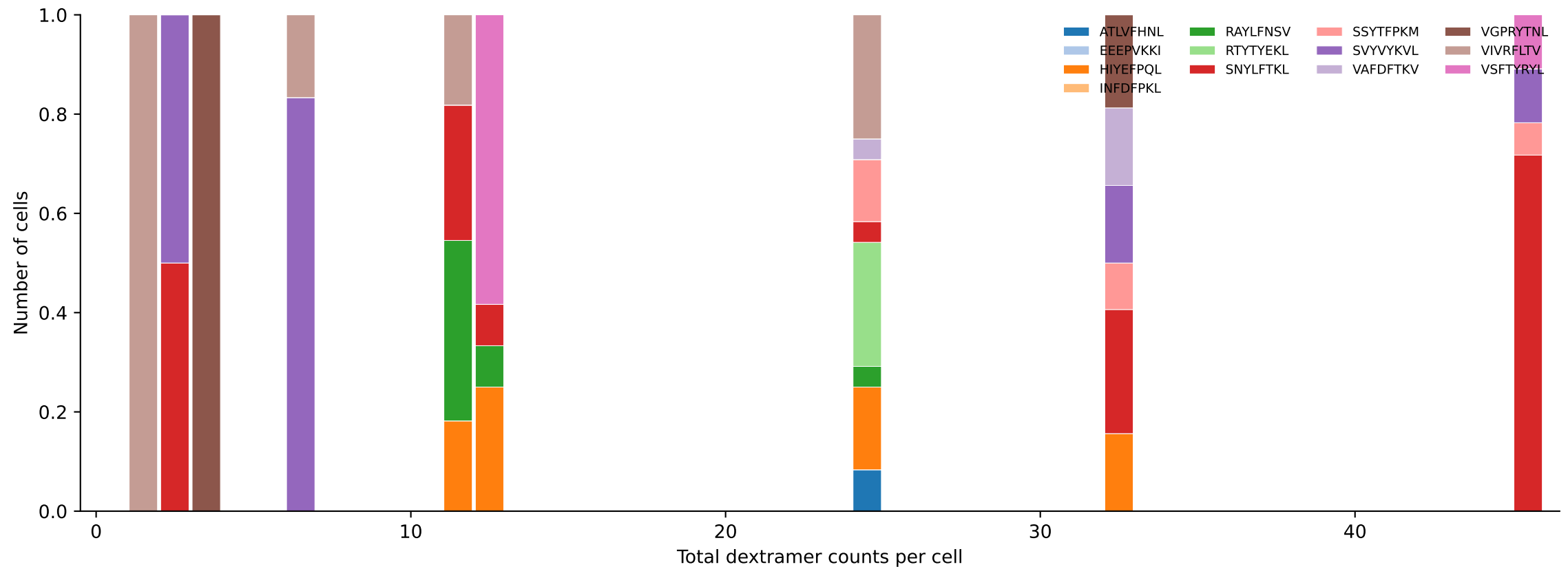
D7ABC_LL Combined | #113 AV16N-CAMRGDSNYQLIW-AJ33_BV13-2-CASGDATISNERLFF-BJ1-4 (n=9) Total pMHC histogram — stacked by mean peptide proportion per bin [113/392]
