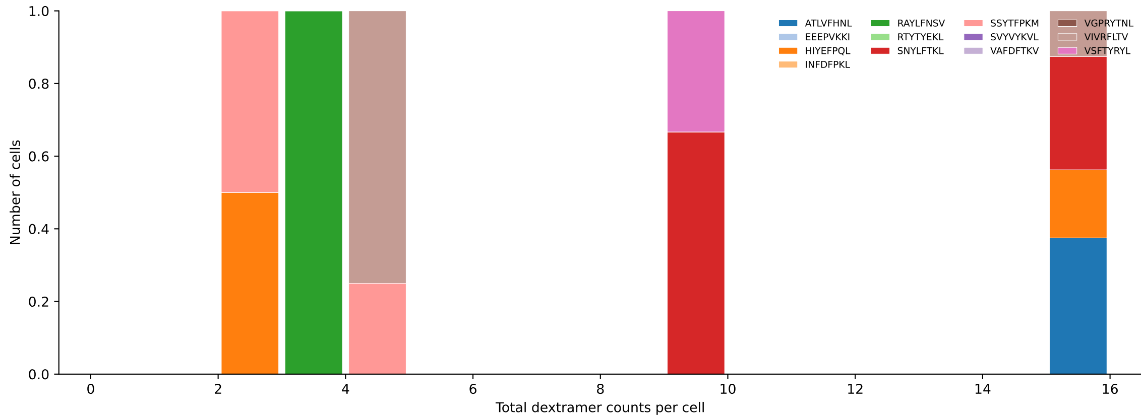
D7ABC_LL Combined | #379 AV3D-3-CALNMGYKLTf-AJ9_BV13-2-CASGARDWGGAQNTLYF-BJ2-4 (n=5) Total pMHC histogram — stacked by mean peptide proportion per bin [379/392]
