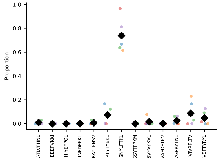
#146 AV13-4/DV7-CAMEVDSNYQLIW-AJ33_BV31-CAWSLGGSDYTf-BJ1-1 coh=0.950, n=7
