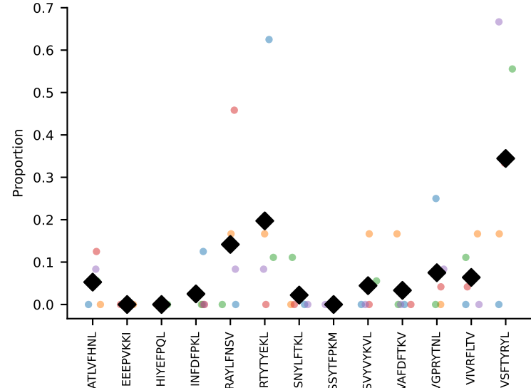
#443 AV5-4-CAAMSNYNVLYF-AJ21_BV2-CASSQERWPETLYF-BJ2-3 coh=0.448, n=15
