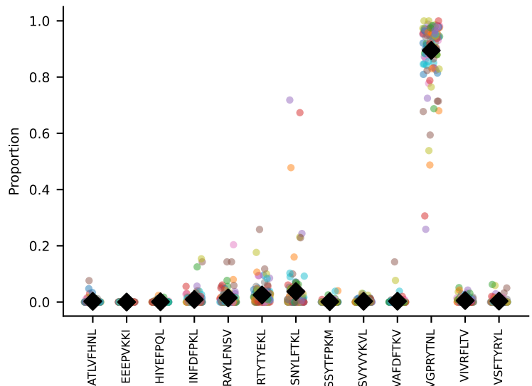
#210 AV8-1-CATDASSGSWQLIF-AJ22_BV13-2-CASGDEGTYNsPLYF-BJ1-1 coh=0.964, n=20
