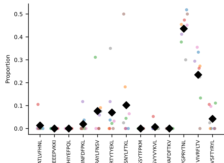
#366 AV16-CAMRDSNTGYQNFYF-AJ49_BV13-2-CASGAGGQNTLYF-BJ2-1 coh=0.766, n=101
