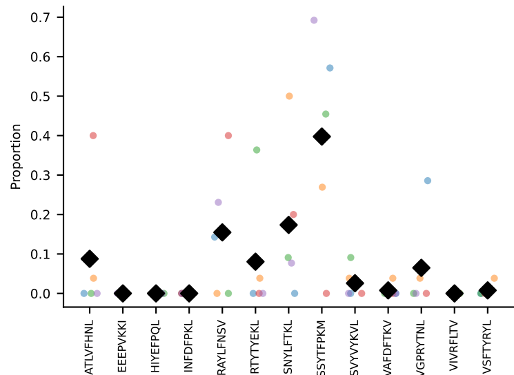
#441 AV3-3-CAVSASNNAGAKLTF-AJ39_BV5-CASSPDRGDERLFF-BJ1-4 coh=0.455, n=55
