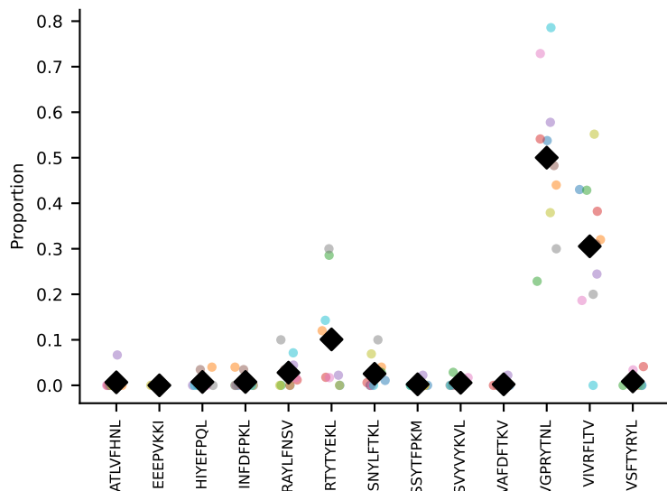
#340 AV13-2-CAIDNNAGAKLTF-AJ39_BV13-3-CASSDRDLYF-BJ2-4 coh=0.841, n=28
