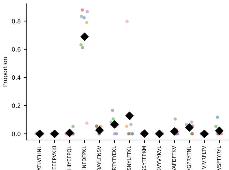
#364 AV12D-3-CALINQGKLIF-AJ23_BV13-2-CASGDINYAEQFF-BJ2-1 coh=0.769, n=8
