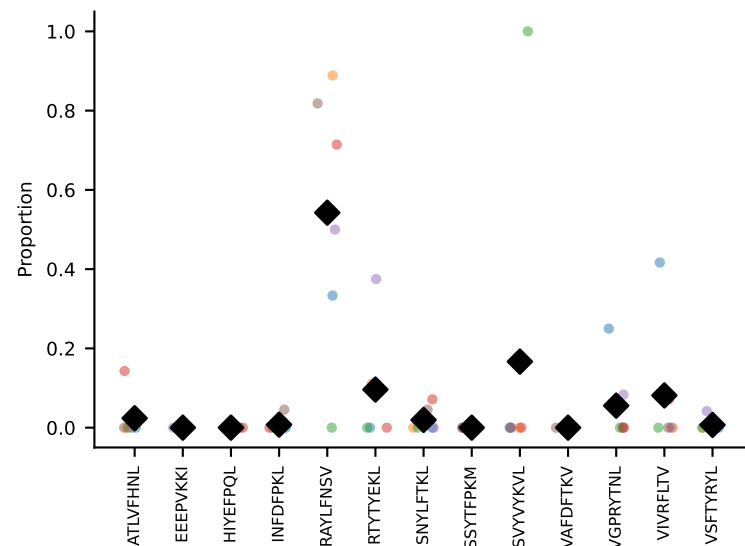
#300 AV16/DV11-CAMREEGGRALIF-AJ15_BV13-1-CASKDTYEQYF-BJ2-7 coh=0.496, n=12
