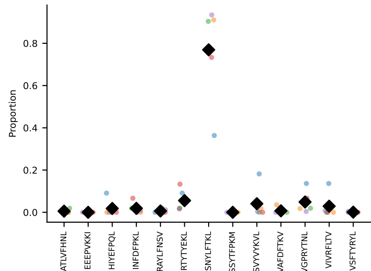
#172 AV12D-3-CALIASGSWQLIF-AJ22_BV13-2-CASGDAGNQAPLF-BJ1-5 coh=0.912, n=5
