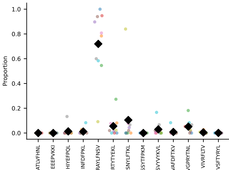
#361 AV14D-3/DV8-CAASEGSALGRLHF-AJ18_BV12-2-CASSLDSNQDTQYF-BJ2-5 coh=0.783, n=5
