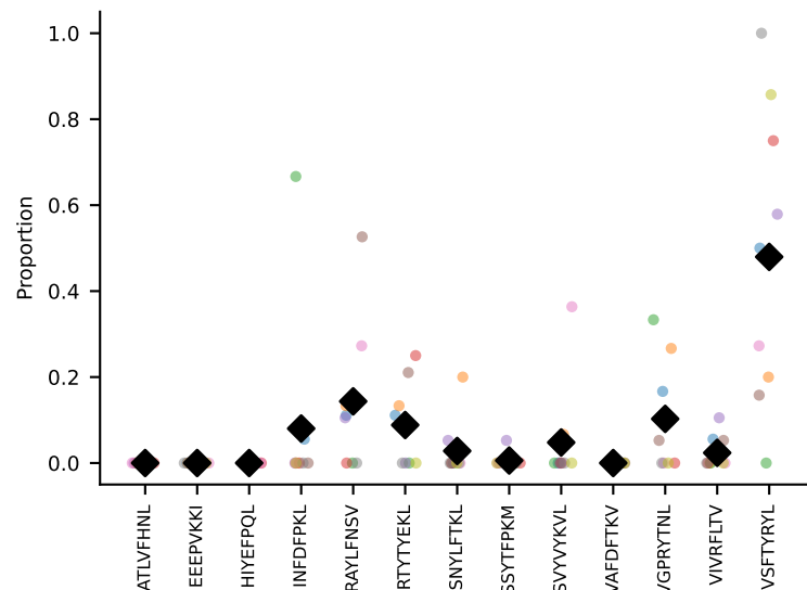
#422 AV14-2-CAASSSNNRIFF-AJ31_BV13-2-CASGGGWGTEVFF-BJ1-#423 AV6-7/DV9-CALSDHAGYQNFYF-AJ49_BV13-2-CASGARTGENYAEQFF-BJ1-1 coh=0.524, n=19
