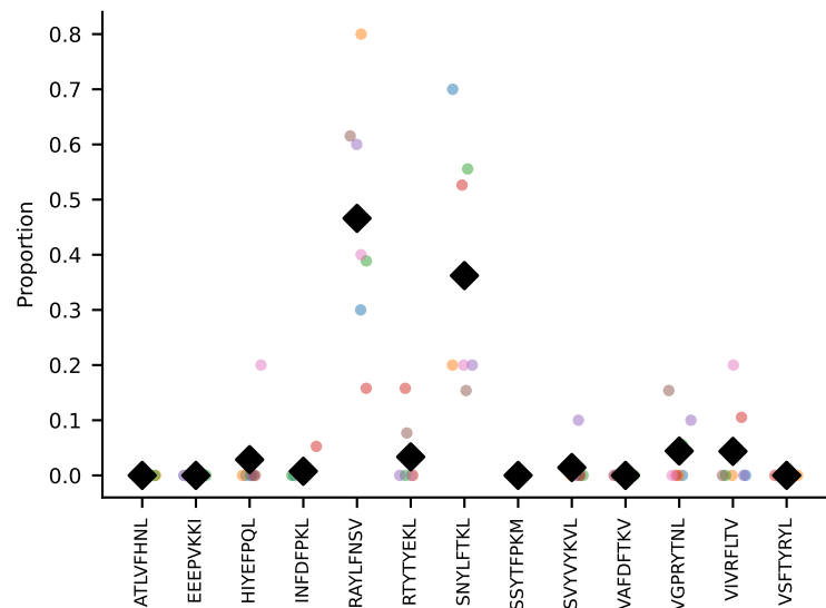
#291 AV12D-2-CALNQGGSAKLIF-AJ57_BV1-CTCSADWGNYAEQFF-BJ2-1#374 AV4-4/DV10-CAAEENTGYQNIFYF-AJ49_BV14-CASSFGTGGEQYF-BJ2-1 coh=0.748, n=90
