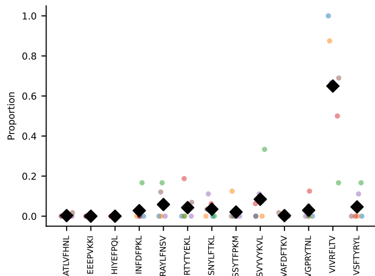
#371 AV4-3-CAAEASTGNYKYVF-AJ40_BV3-CASSLVQVTEVFF-BJ1-1 coh=0.753, n=14
