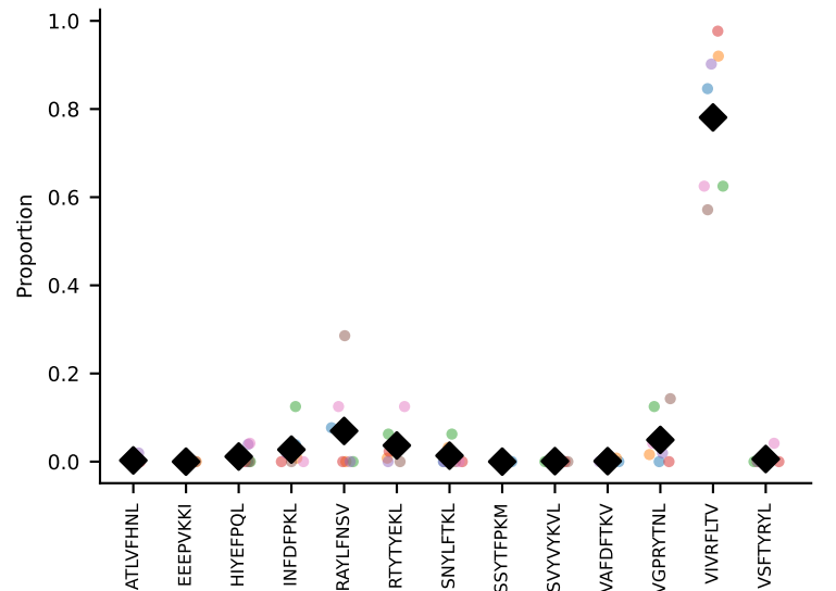
#219 AV9-2-CVLNTGYQNfYF-AJ49_BV13-1-CASSVAGREQYF-BJ2-7 coh=0.948, n=13
