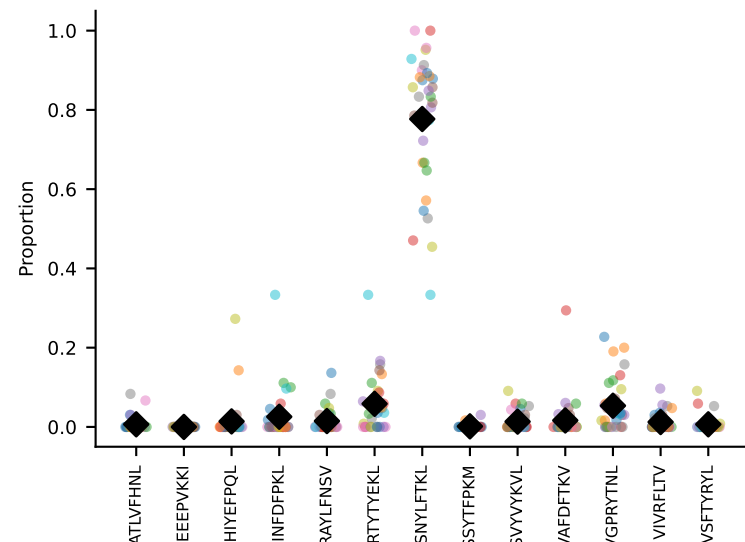
#233 AV13-4/DV7-CAMERGG5NAKLTF-AJ42_BV13-2-CASGEGQGKNTLYF-BJ2-4 coh=0.932, n=9
