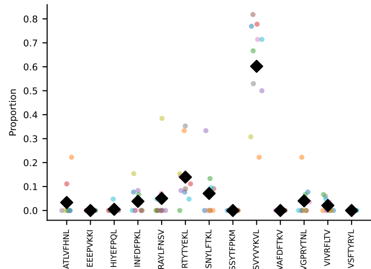
#363 AV14-2-CAASADTGNYKYVF-AJ40_BV13-3-CASSDMGGQNTLYF-BJ2-1 coh=0.781, n=8
