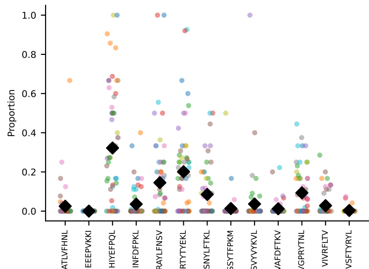
#445 AV13D-2-CAIDPNYNVLYF-AJ21_BV13-3-CASSEKGREQYF-BJ2-7 coh=0.442, n=40
