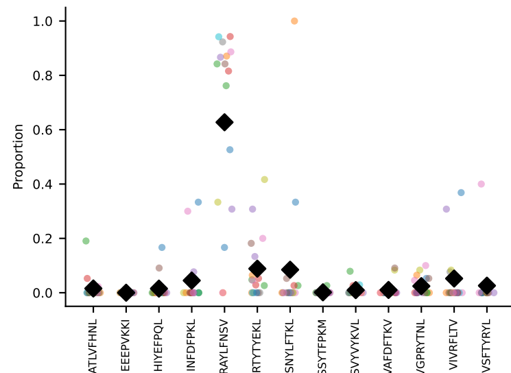
#398 AV13-1-CALERSNRRIF-AJ31_BV2-CASSQDRRGDTQYF-BJ2-5 coh=0.606, n=65
