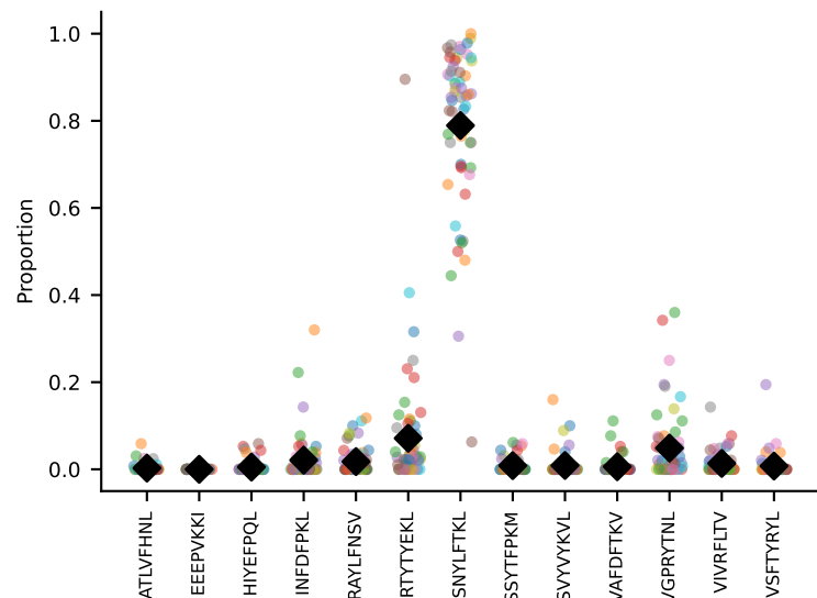
#249 AV13-4/DV7-CAMPNSNNRIFF-AJ31_BV3-CASSLGVDQYF-BJ2-5 coh=0.912, n=25
