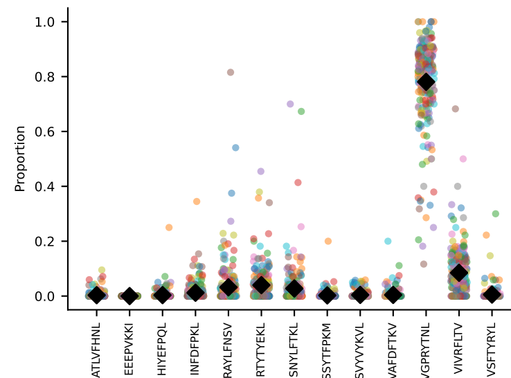
#239 AV16-CAMRDSNTGYQNFYF-AJ49_BV13-2-CASGDGGKNTLYF-BJ2-2 coh=0.925, n=8
