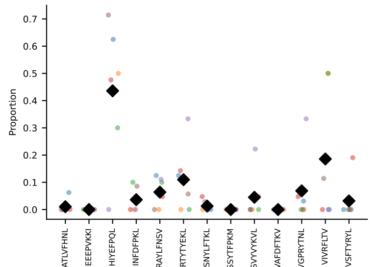
#423 AV6-7/DV9-CALSDHAGYQNFYF-AJ49_BV13-2-CASGARTGENYAEQFF-BJ1-1 coh=0.521, n=5
