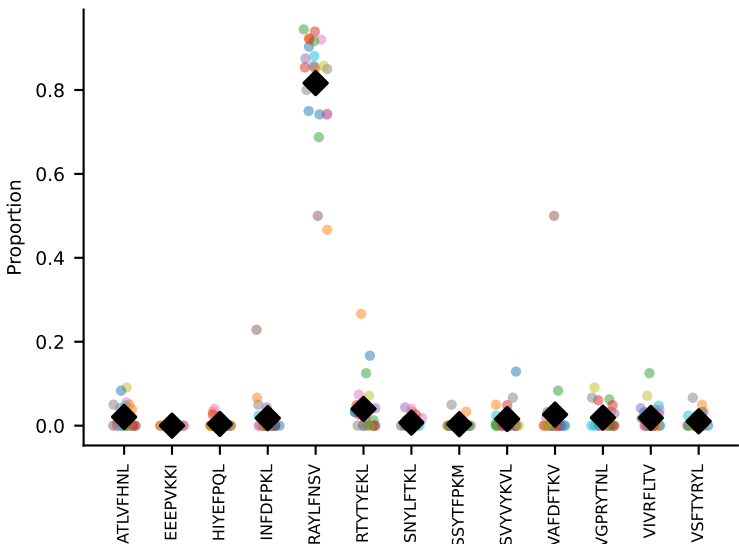
#307 AV7-2-CAAITGSGGKLTf-AJ44_BV31-CAWSLGNYAEQFF-BJ2-1 coh=0.951, n=6
