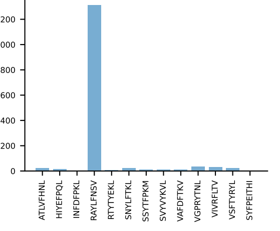
AV16/DV11-CAMREHNTNTGKLTf-AJ27_BV1-CTCSADRVGNTLYF-AJ16 RAW n:10→0 LOST
