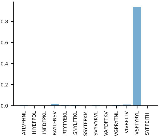
AV6D/DV11-CAMREGNNNNRIFF-AJ31_BV13-2-CAGGTVYEQYF-BJ2-7 PROP n:11→0 LOST
