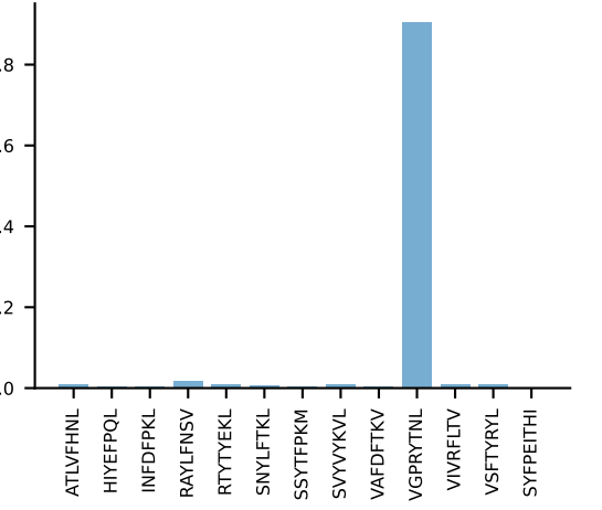
AV13D-2-CAIDPNTDKVVF-AJ34*p03_BV14-CASSSGNTLYF-BJ1-3 PROP n:10→0 LOST
