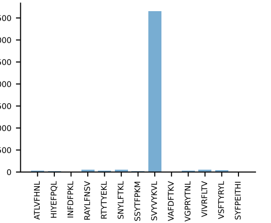
AV6D/DV11-CAMREGNSGTYQRF-AJ13_BV13-2-CASGVDNSGNMIF-BJ1-1 RAW n:11→0 LOST
