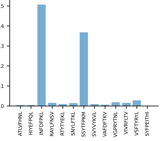
AV6D/DV11-CAMREGNSGTYQRF-AJ13_BV3-CASSPDWTSATETLYF-BJ1-1 PROP n:9→0 LOST
