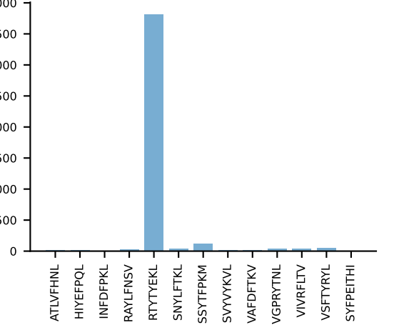
AV16D/DV11-CAMREGSTGYQNIFY-AJ49_BV13-2-CASGEQVYEQYF-BJ2-7 RAW n:10→0 LOST
