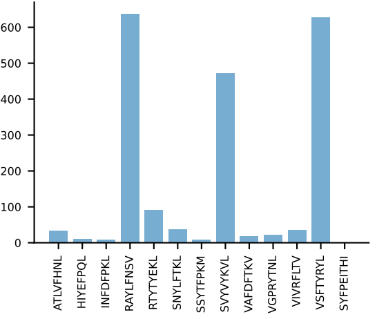
AV16D/DV11-CAMREGSNYQLIW-AJ33_BV13-2-CASGGVYEQYF-BJ2-7 RAW n:10→0 LOST
