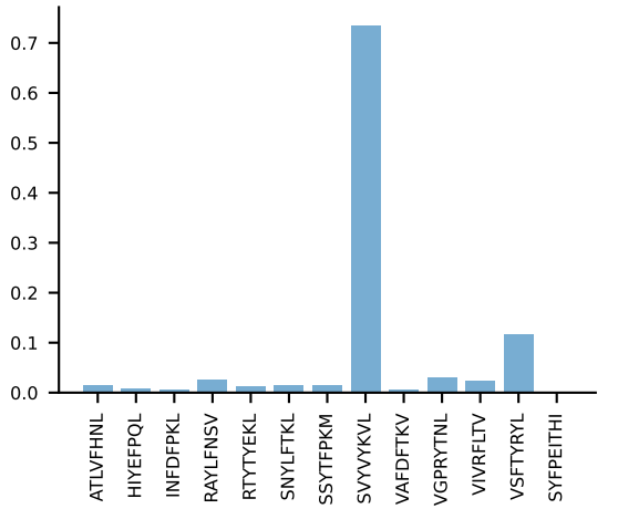
AV13D-2-CAIDPNTDKVVF-AJ34*p03_BV14-CASSSGNTLYF-BJ1-3 PROP n:11→0 LOST
