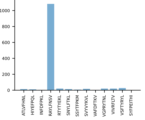
AV16/DV11-CAMREDNNNAPRF-AJ43*p03_BV5-CASSQDWTGGTEV-AJ15 RAW n:10→0 LOST
