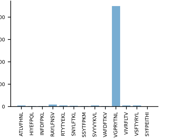
AV13D-2-CAIDPNTDKVVF-AJ34*p03_BV14-CASSSGNTLYF-BJ1-3 RAW n:10→0 LOST
