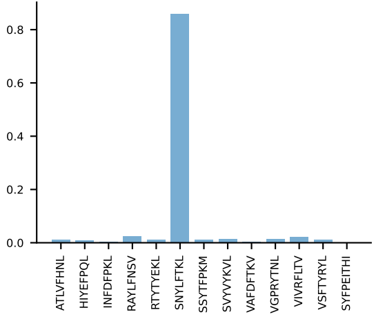
AV16D/DV11-CAMREGLNNRIFF-AJ31_BV30-CSSRGLGGYEQYF-BJ2-7 PROP n:10→0 LOST
