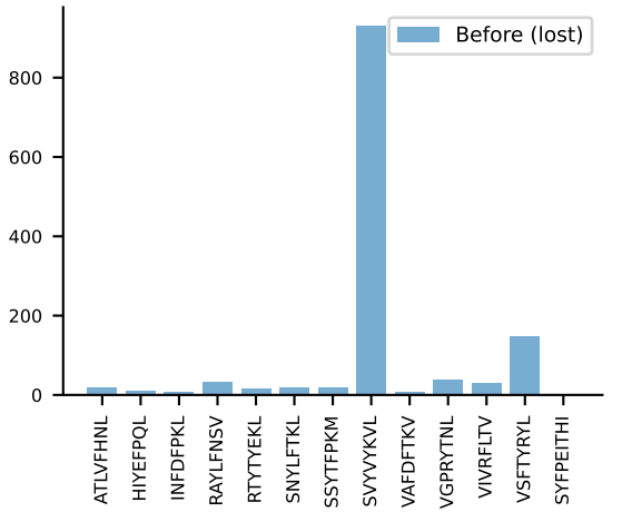
AV13D-2-CAIDPNTDKVVF-AJ34*p03_BV14-CASSSGNTLYF-BJ1-3 RAW n:11→0 LOST
