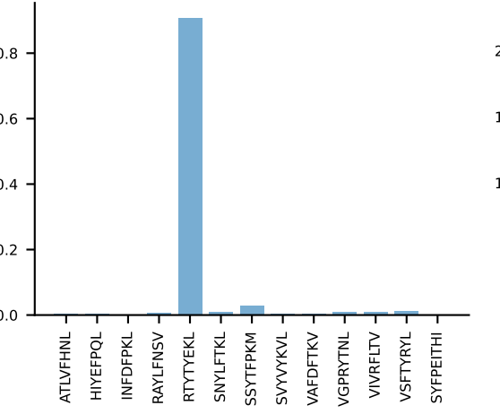
AV16D/DV11-CAMREGSTGYQNIFY-AJ49_BV13-2-CASGEQVYEQYF-BJ2-7 PROP n:10→0 LOST
