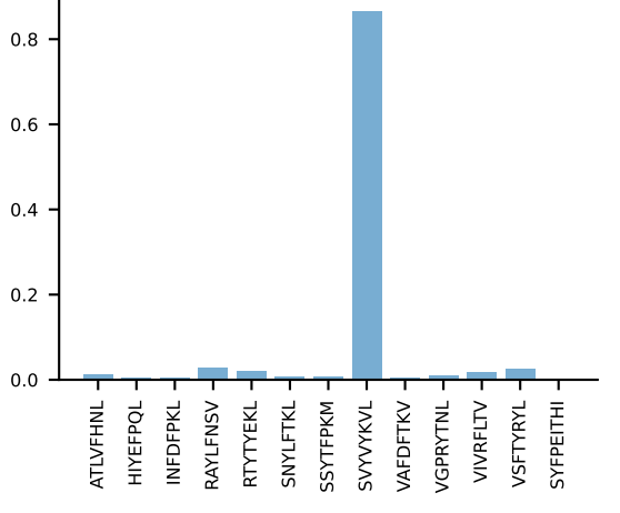
AV16/DV11-CAMREDNNNAPRF-AJ43*p03_BV5-CASSQDWTGGTEV-AJ15 PROP n:10→0 LOST
