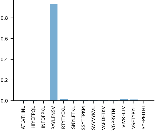
AV16/DV11-CAMREHNTNTGKLTf-AJ27_BV1-CTCSADRVGNTLYF-AJ16 PROP n:10→0 LOST
