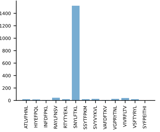
AV16D/DV11-CAMREGLNNRIFF-AJ31_BV30-CSSRGLGGYEQYF-BJ2-7 RAW n:10→0 LOST
