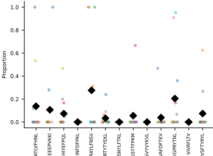
#105 AV14-2-CAASASSGSWQLIF-AJ22_BV31-CAWSLQSGNTLYF-BJ1-3 coh=0.154, n=26
