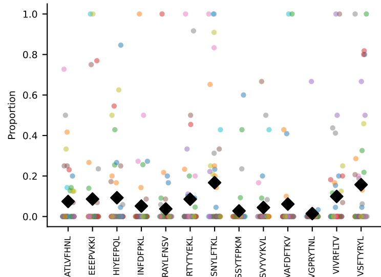
#79 AV7-2-CAAGNTGKLIF-AJ37_BV1-CTCSAVRVGYEYF-BJ2-7 coh=0.179, n=49
