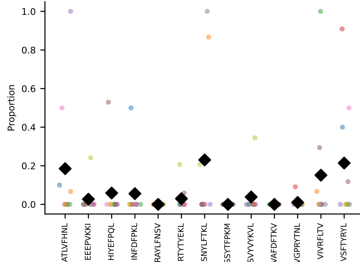
#103 AV9D-2-CVLSAANSAGNKLTF-AJ17_BV16-CASSLGEDTYQYF-BJ2-5 coh=0.156, n=6
