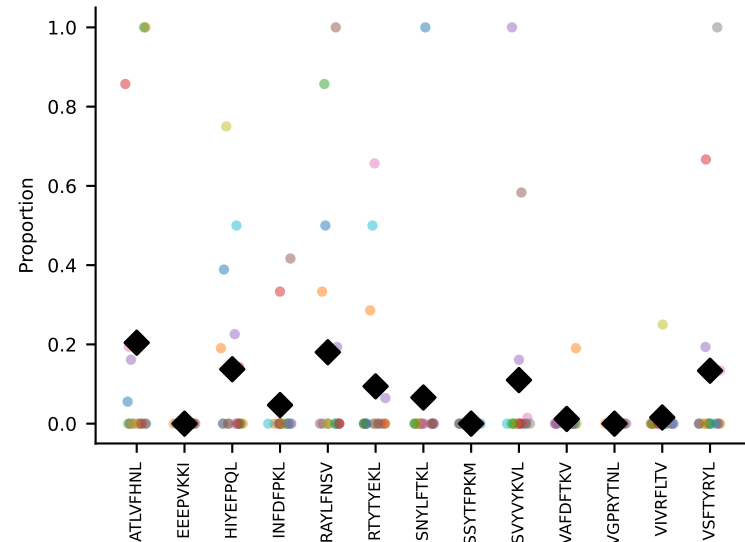
#77 AV16-CAMREGQGGS AKLIF-AJ57_BV16-CASSLVWGQGSSYEYF-BJ2-7 coh=0.182, n=21
