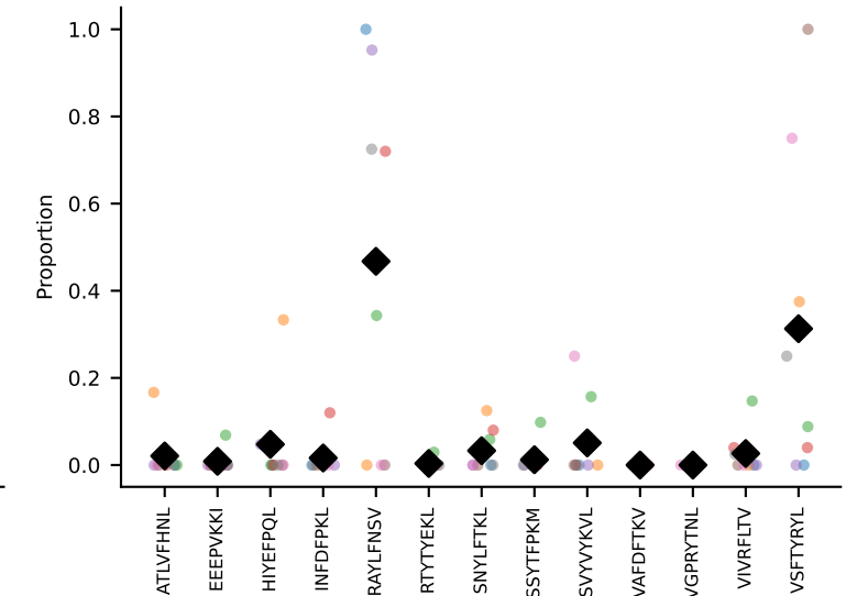
#24 AV16N-CAMRDNYAQGLTF-AJ26_BV3-CASSLGPSSYEQYF-BJ2-7 coh=0.403, n=279
