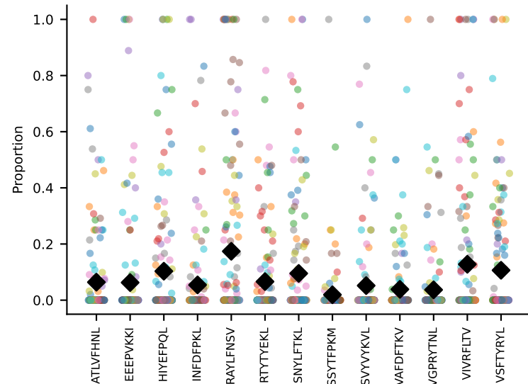
#78 AV14-2-CAASGNYNVLYF-AJ21_BV3-CASSLDWGGSYEYF-BJ2-7 coh=0.180, n=8
