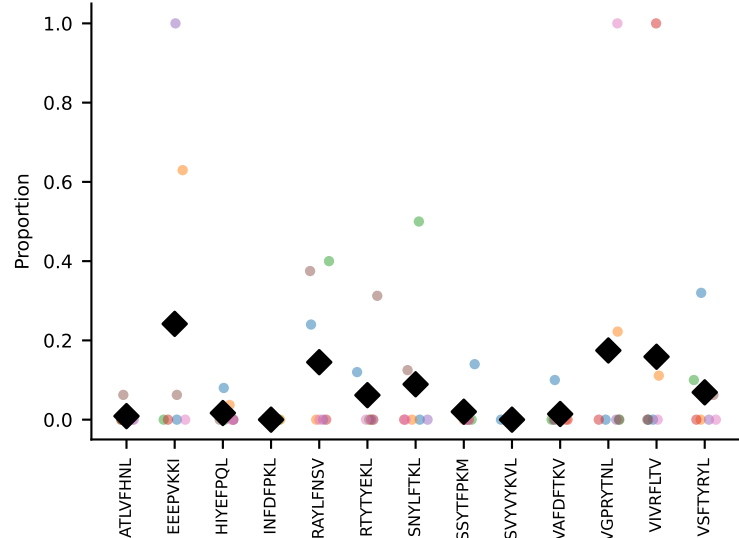
#102 AV7-6-CAVYGNEKITF-AJ48_BV5-CASSPDRGYTYF-BJ2-5 coh=0.156, n=12
