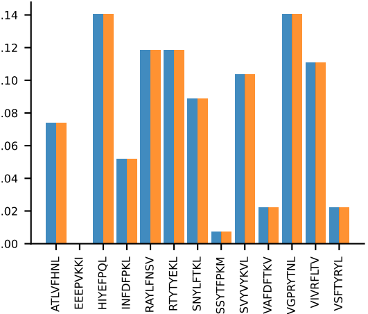
AV3-3-CAVSAPEGADRLTF-AJ45_BV13-2-CASGDARDNQAPLF-BJ1-5
