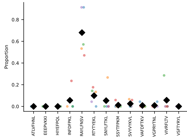
#114 AV12-2-CALSMQQGTGSKLSF-AJ58_BV1-CTCSAVRISNERLFF-BJ1-4 coh=0.846, n=59
