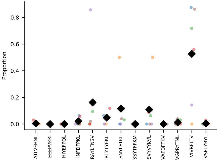
#173 AV5-4-CAAMSNYNVLVYF-AJ21_BV2-CASSQERWPETLYF-BJ2-3 coh=0.448, n=15
