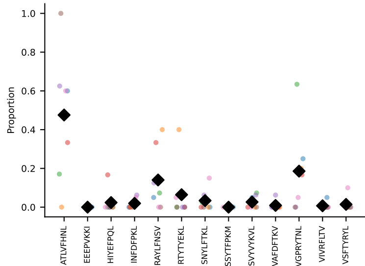
#162 AV6-6-CALGEAGGSNAKLTF-AJ42_BV14-CASSPGLSYNSPLYF-BJ1-1 coh=0.525, n=5
