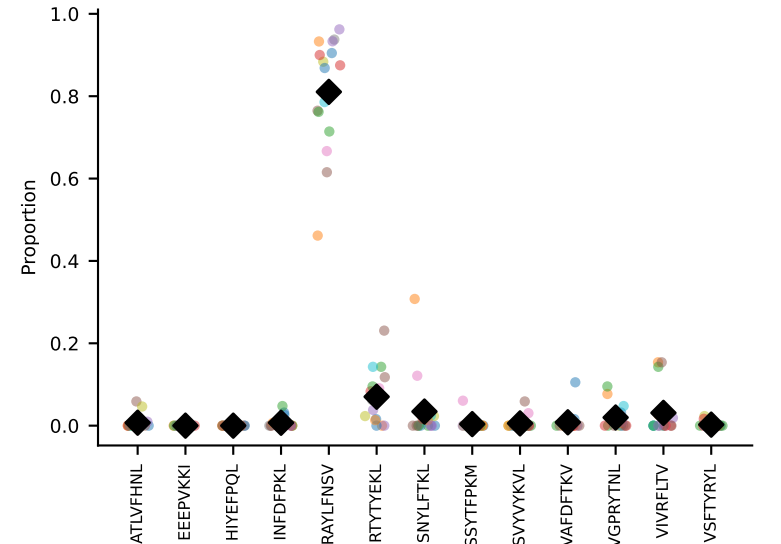
#68 AV6N-6-CALSGANTGKLTF-AJ52_BV1-CTCSANRVDLTLYF-BJ2-4 coh=0.952, n=24
