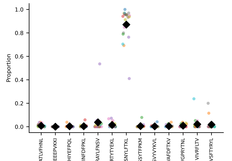
#72 AV7-1-CAATSSGQKLVF-AJ16_BV13-1-CASSDVGGRG TGQLYF-BJ2-7 coh=0.950, n=20
