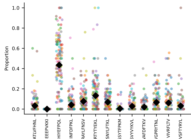
#156 AV16N-CAMREEAGNTGKLIF-AJ37_BV20-CGARDWGGYEQYF-BJ2- coh=0.559, n=32
