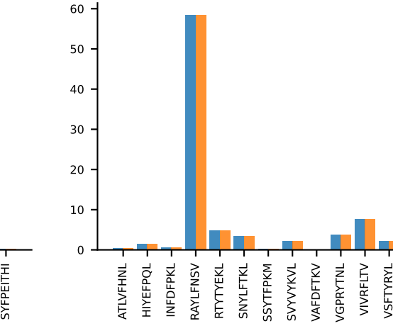
AV16D/DV11-CAMRDPYGGSGNKLI-AJ32_BV1-CTCSAVREDTQYF-BJ2-2AV16D/DV11-CAMRDPYGGSGNKLI-AJ32_BV1-CTCSAVREDTQYF-BJ2-2 MEAN n:6→6
