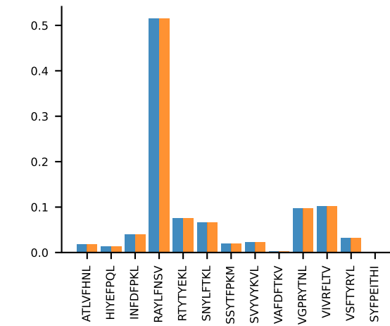
AV6-5-CALSDGGTGSKLSF-AJ58_BV17-CASSPGLGGRFNEQYF-BJ2-2AV6-5-CALSDGGTGSKLSF-AJ58_BV17-CASSPGLGGRFNEQYF-BJ2-2 PROP n:6→6
