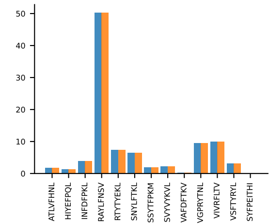
AV6-5-CALSDGGTGSKLSF-AJ58_BV17-CASSPGLGGRFNEQYF-BJ2-2AV6-5-CALSDGGTGSKLSF-AJ58_BV17-CASSPGLGGRFNEQYF-BJ2-2 MEAN n:6→6
