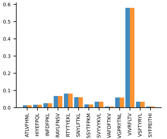
AV14-1-CAARGDNNRIFF-AJ31_BV1-CTCSANRVNDNQAPLF-BJ1-5AV14-1-CAARGDNNRIFF-AJ31_BV1-CTCSANRVNDNQAPLF-BJ1-5 PROP n:6→6
