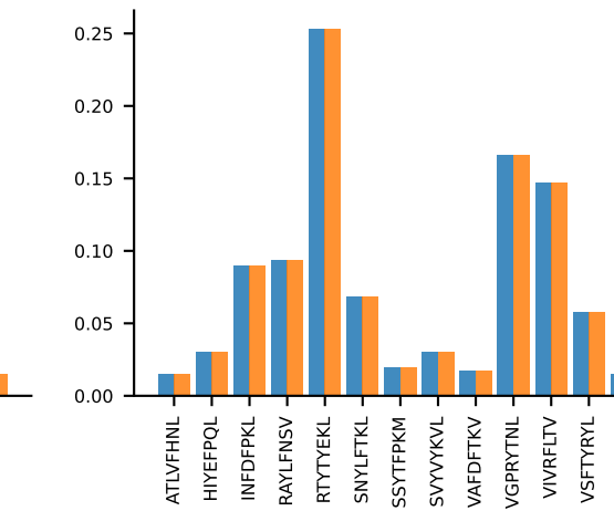
AV7-3-CAVNAYKVIF-AJ30_BV13-2-CASGDLGGRDAETLYF-BJ2-3AV7-3-CAVNAYKVIF-AJ30_BV13-2-CASGDLGGRDAETLYF-BJ2-3 MEAN n:6→6
