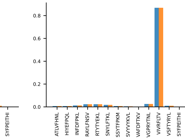
AV16D/DV11-CAMRDPYGGSGNKLI-AJ32_BV1-CTCSAVREDTQYF-BJ2-2AV16D/DV11-CAMRDPYGGSGNKLI-AJ32_BV1-CTCSAVREDTQYF-BJ2-2 MEAN n:6→6
