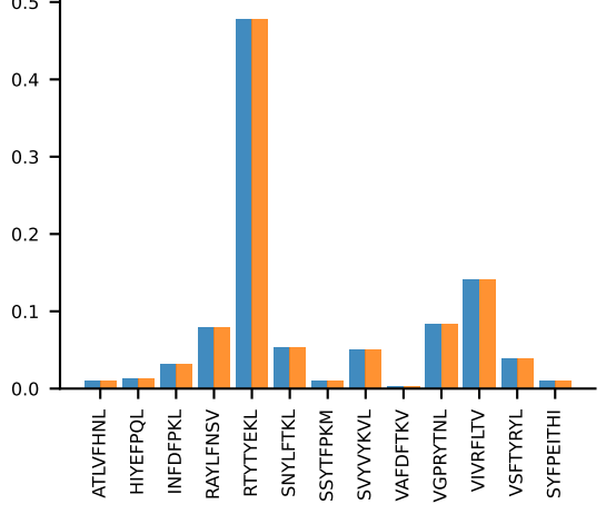
AV12-2-CALSDRYGNEKITF-AJ48_BV29-CASSPLKGANSDYTF-BJ1-1AV12-2-CALSDRYGNEKITF-AJ48_BV29-CASSPLKGANSDYTF-BJ1-1 PROP n:6→6
