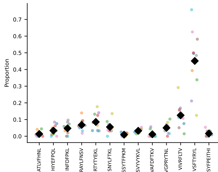
#9-A-V16D/DV11-CAMRENSGYNKLTf-AJ11*p02_BV13-2-CASGETGGREQYF coh=0.794, n=6
