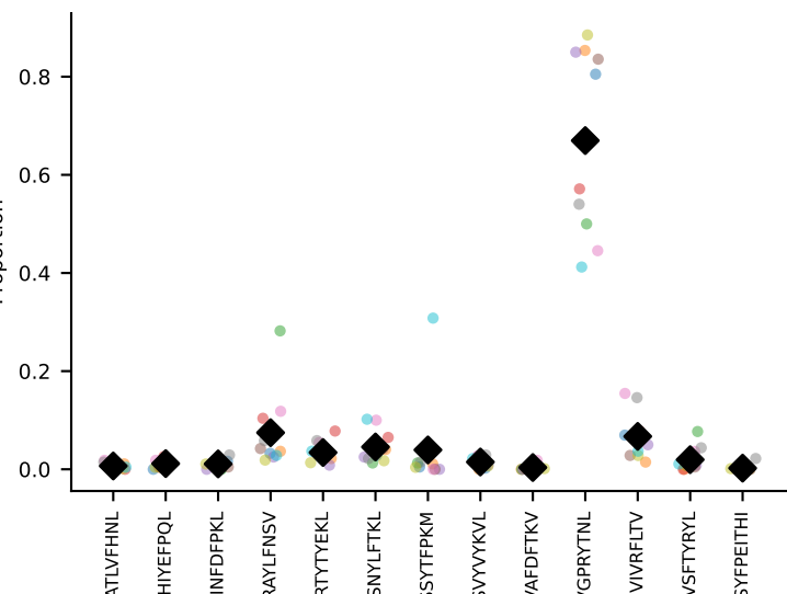
#12 AV6D-7-CALRYGGSGNKLIF-AJ32_BV3-CASSLGTGDTQYF-BJ2-5 coh=0.921, n=10
