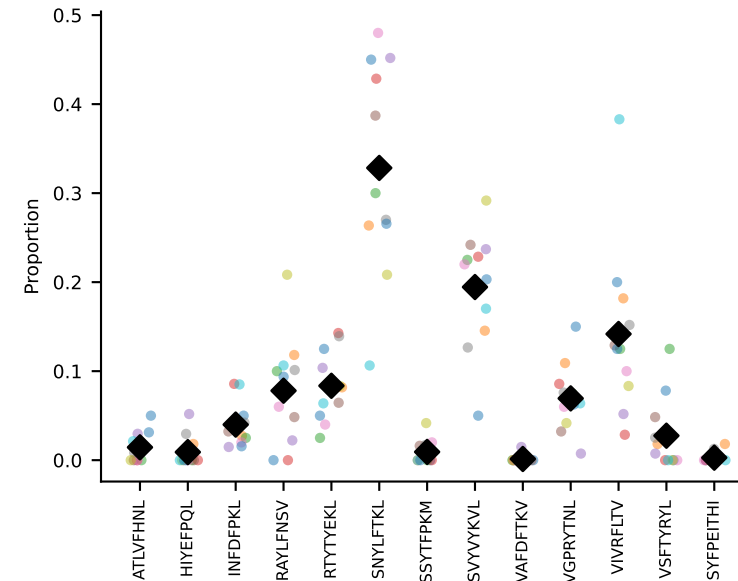
#20 AV6-6-CALGSYTGADRLTF-AJ45_BV13-1-CASSDRGANTGQLYF-BJ2 coh=0.710, n=6
