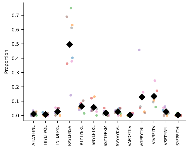
#18 AV16D/DV11-CAMREGDSNYQLIW-AJ33_BV13-2-CASGYRAPNSDYT coh=0.820, n=8
