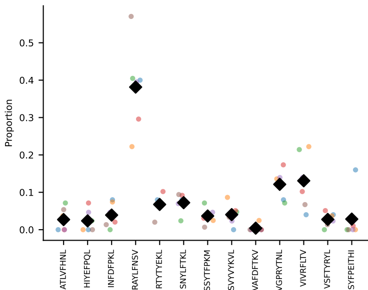
#17 AV15-2/DV6-2-CALSELPGSNAKLTF-AJ42_BV13-2-CASGRGAGNTLYF- coh=0.837, n=8
