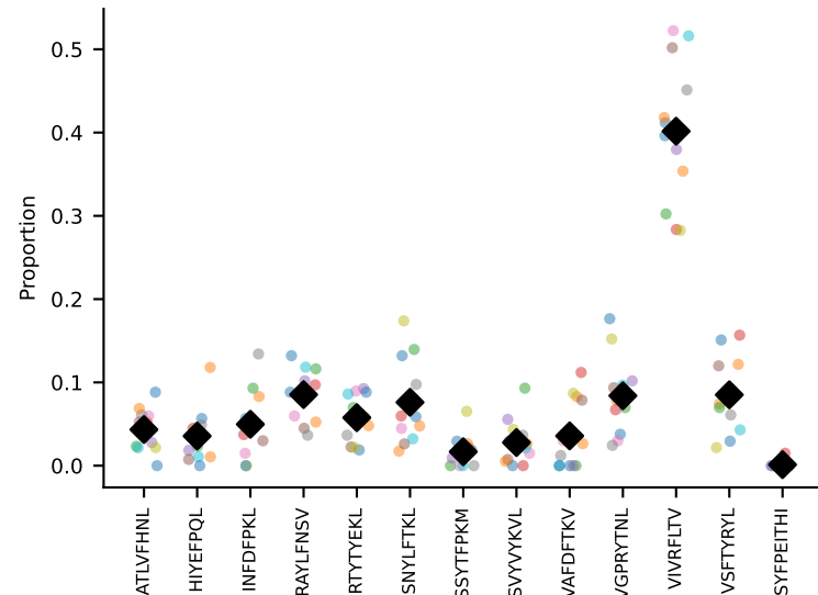
#51 AV1-CAVRDSYAQGLTF-AJ26_BV13-1-CASSDDRVGNTLYF-BJ1-3 coh=0.912, n=12
