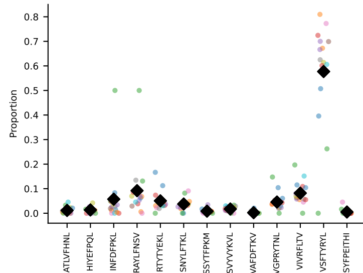
#83 AV6D-6-CALSDRGNTNGKLTTF-AJ27_BV29-CASTPGLQDTQYF-BJ2-5 coh=0.828, n=7
