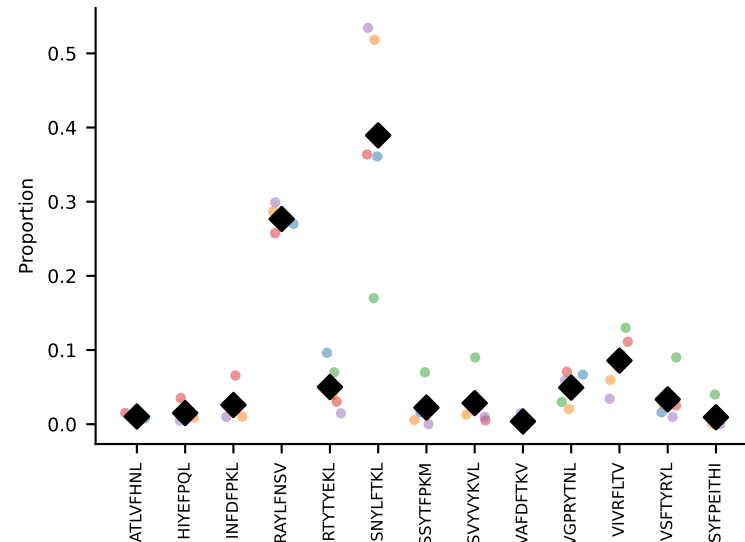
#49 AV9D-3-CAVSPDTNAYKVIF-AJ30_BV13-2-CASGDWGRGEQYF-BJ2-7#50 AV16D/DV11-CAMREGSSGSWQLIF-AJ22_BV1-CTCSADRVYAEQFF-BJ2-1 coh=0.913, n=5
