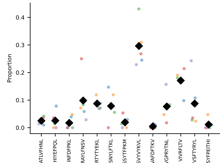
#84 AV5-1-CSASNGAKLTTF-AJ39_BV13-2-CASGDVTGGDSPLYF-BJ1-6 coh=0.825, n=5
