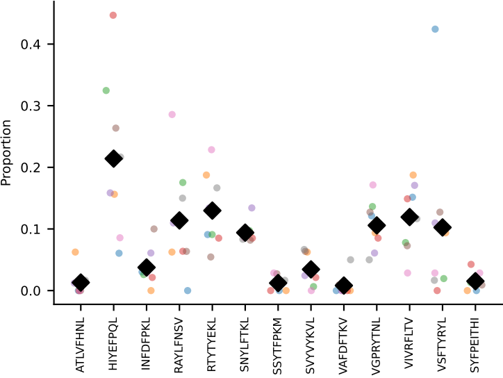
#117 AV16D/DV11-CAMRVSN TGYNFYF-AJ49_BV1-CTCSEDRVYAEQFF-BJ2-1 coh=0.716, n=8
