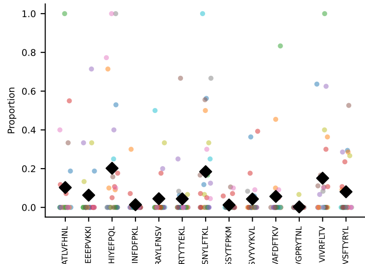
#59 AV7-2-CAASKGGRALIF-AJ15_BV13-1-CASSDWASSYEQYF-BJ2-7 coh=0.244, n=27
