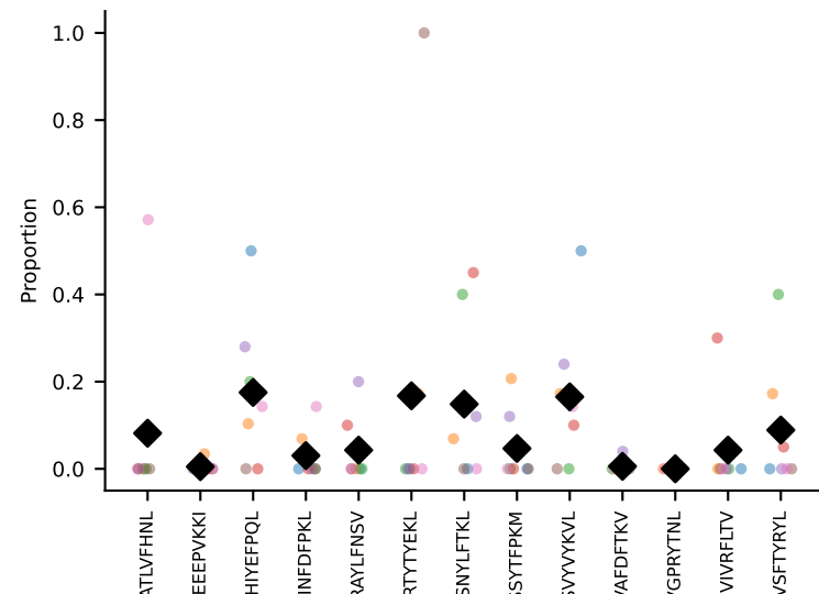
#45 AV7D-5-CAVRDTGGLSGKLT-F-AJ2_BV1-CTCSADRLGSAETLYF-BJ2-3 coh=0.272, n=7
