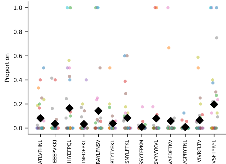
#79 AV3D-3-CAAGTGGYKVVVF-AJ12_BV26-CASSLGSLNQDTQYF-BJ2-5 coh=0.205, n=6
