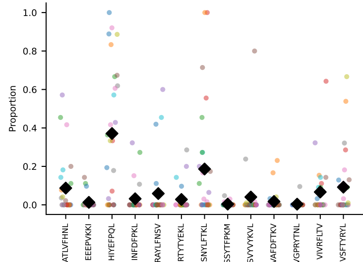
#24 AV21/DV12-CILRVAWNNNAPRF-AJ43_BV2-CASSQEQGYAEQFF-BJ2-7 coh=0.356, n=27
