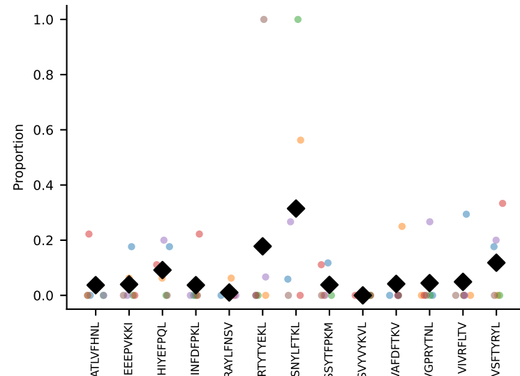
#57 AV12-2-CALRGTYGNYKYVF-AJ40_BV1-CTCSASRDPYNSPLYF-BJ1-6 coh=0.248, n=6
