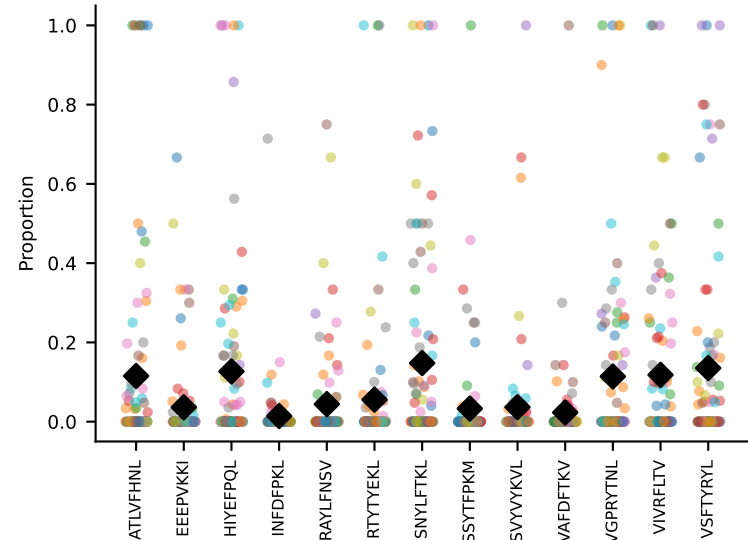
#77 AV10-CAASMDYANKMIF-AJ47_BV3-CASSPGTGIEQYF-BJ2-7 coh=0.211, n=8
