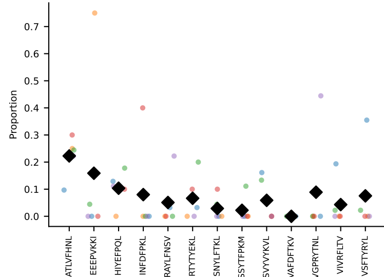
#56 AV7-2-CAASMGTTGGYKVVF-AJ12_BV13-2-CASLGEYAEQFF-BJ2-1 coh=0.253, n=5
