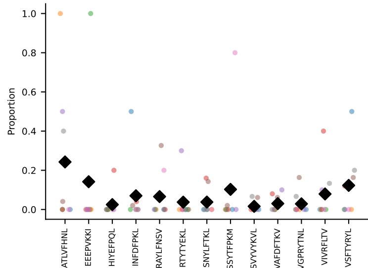
#91 AV8N-2-CATENYGSSGNKLIF-AJ32_BV3-CASSLGREYTQYF-BJ2-5 coh=0.162, n=14
