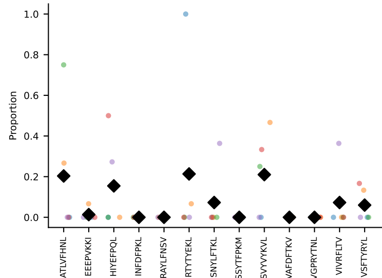
#90 AV7-5-CAVSMDNYAQGLTF-AJ26_BV1-CTCSAVRVSGNTLYF-BJ1-3 coh=0.164, n=5
