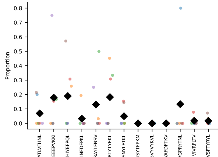
#60 AV14D-3/DV8-CAASETSGSWQLIF-AJ22_BV5-CASSPRLGGDTQYF-BJ coh=0.244, n=6
