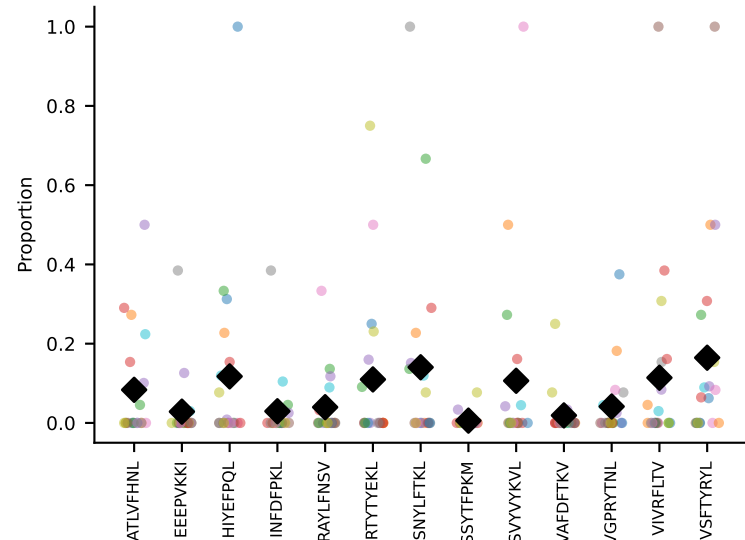
#58 AV10-CAASDVGDNSKLIW-AJ38_BV1-CTCSADWTSGNTLYF-BJ1-3 coh=0.245, n=5
