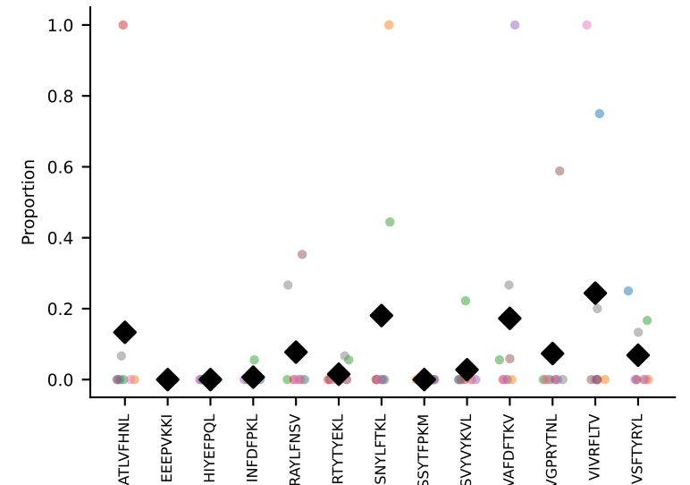
#96 AV7D-6-CAGNYSNNRLTL-AJ7_BV16-CASSLNWGANYAEQFF-BJ2-1 coh=0.153, n=8
