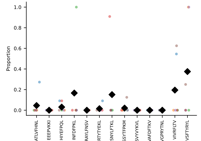
#92 AV12D-3-CALSGPGTGSNRLTF-AJ28_BV29-CASTANTEVFF-BJ1-1 coh=0.161, n=26
