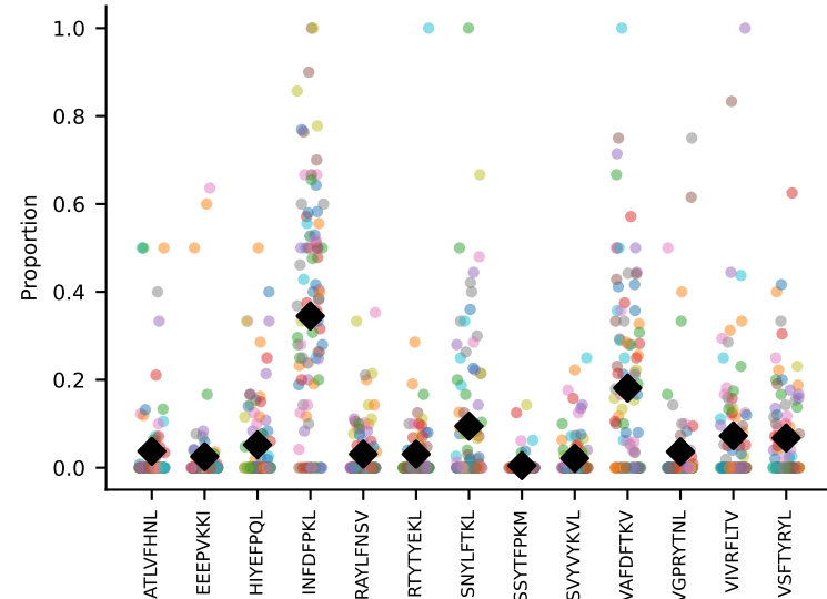
#17 AV16N-CAMREGNSNNRIFF-AJ31_BV13-1-CASRDINTEVFF-BJ1-1 coh=0.434, n=10
