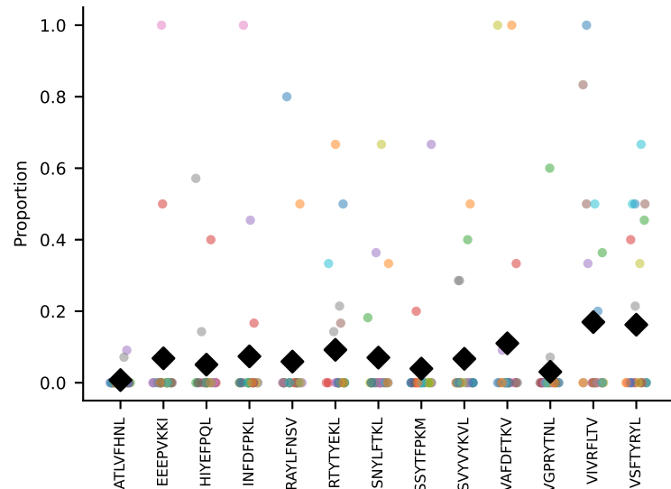
#95 AV7-3-CAVSAEGADRLTF-AJ45_BV1-CTCSADRGGSPLYF-BJ1-6 coh=0.154, n=22
