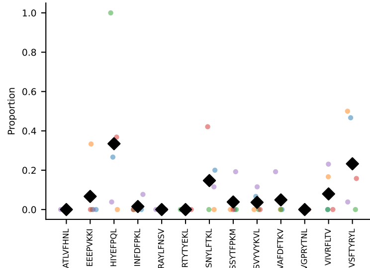
#23 AV14-1-CAASASSGSWQLIF-AJ22_BV1-CTCSGRDRANQAPLF-BJ1-5 coh=0.363, n=5
