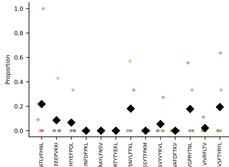
#94 AV7-2-CAADNVGDNSKLIW-AJ38_BV4-CASSPGTGYSDYTF-BJ1-2 coh=0.155, n=5
