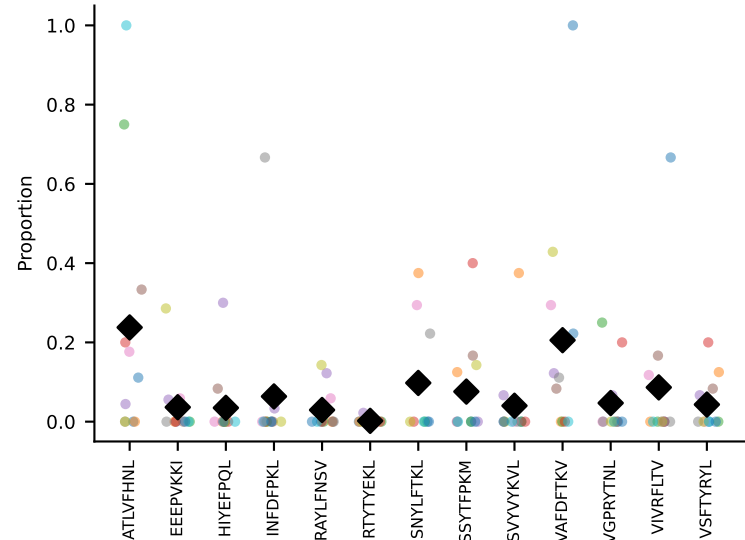
#54 AV14-2-CAASASSGSWQLIF-AJ22_BV31-CAWSLAGSGNTLYF-BJ1-3 coh=0.254, n=19
