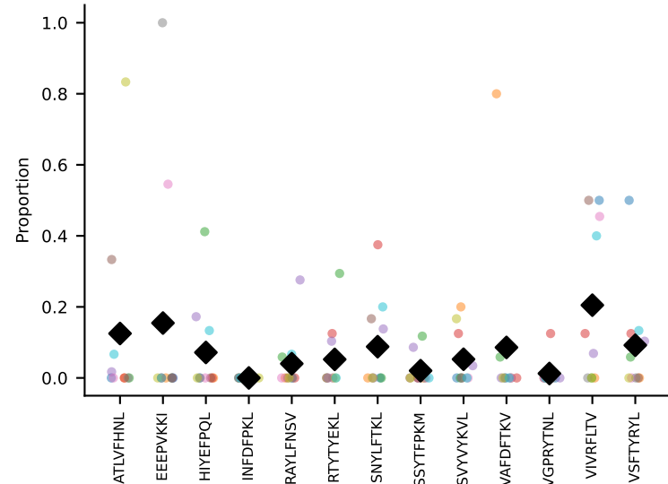
#78 AV16-CAMGTGSGGKLT-L-AJ44_BV1-CTCSTRGANERLFF-BJ1-4 coh=0.209, n=34
