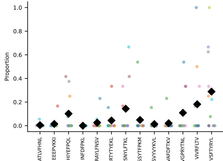
#55 AV19-CAANQGGSAKLIF-AJ57_BV5-CASSRQVNYAEQFF-BJ2-1 coh=0.253, n=9
