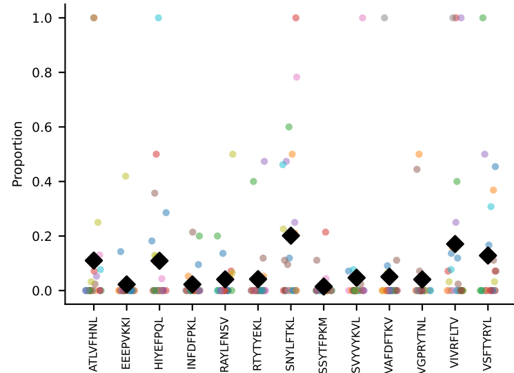
#70 AV14-2-CAASASSGSWQLIF-AJ22_BV13-1-CASSGTGGINQAPLF-BJ1-5 coh=0.222, n=25
