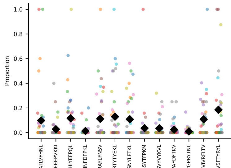
#48 AV7-4-CAASEDYNQGKLIF-AJ23_BV31-CAWSLGHYAEQFF-BJ2-1 coh=0.268, n=39
