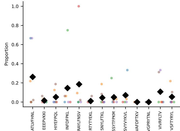
#69 AV14-2-CAASGTGYQNFYF-AJ49_BV2-CASSQAWGNQDTQYF-BJ2-5 coh=0.226, n=6
