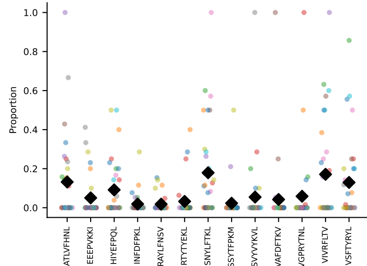
#53 AV14-2-CAASAASGSWQLIF-AJ22_BV31-CAWSLAGSGNTLYF-BJ1-3 coh=0.259, n=7
