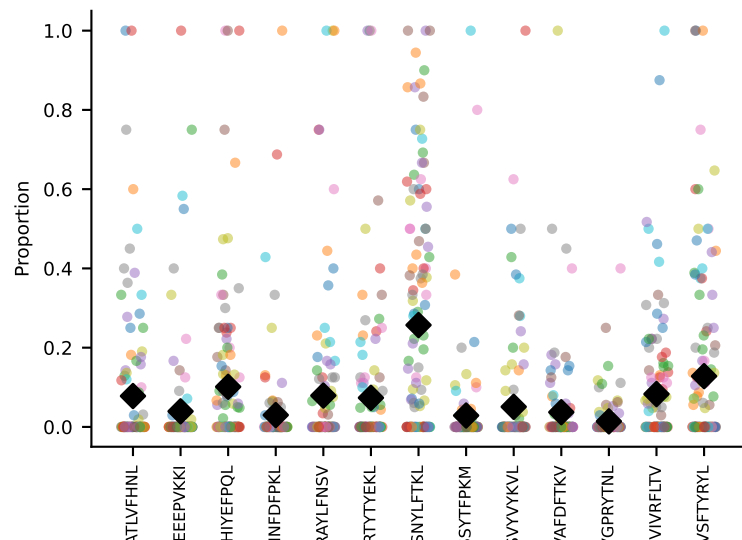
#46 AV16N-CAMREETGNTGKLIF-AJ37_BV1-CTCSANRVDTQYF-BJ2-5 coh=0.269, n=8
