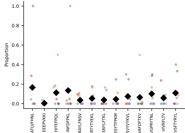
#81 AV3D-3-CAVSEPSGSWQLIF-AJ22_BV5-CASSQGRGHERLFF-BJ1-4 coh=0.203, n=9
