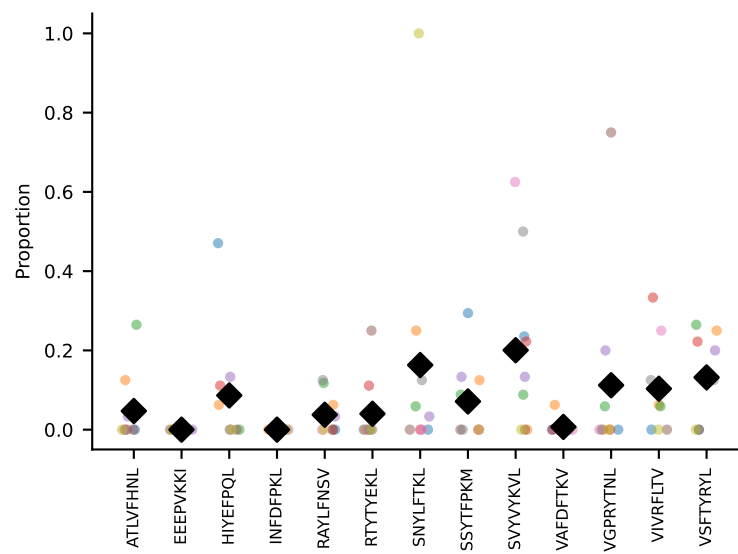
#43 AV3D-3-CAAGTGGYKVVF-AJ12_BV26-CASSLGSNLNQDTQYF-BJ2-5 coh=0.311, n=8
