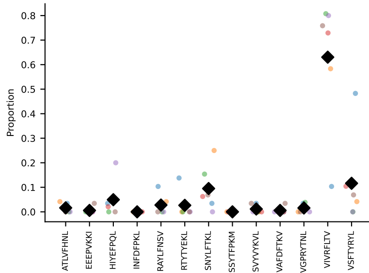
#7 AV16-CAMRESNTGYQNFYF-AJ49_BV13-2-CASGTGGQNTLYF-BJ2-4 coh=0.618, n=84
