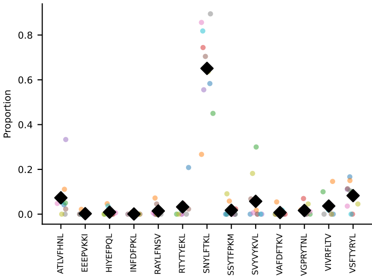
#5 AV6N-6-CARASSGSWQLIF-AJ22_BV13-1-CASSDAGTEVFF-BJ1-1 coh=0.645, n=6
