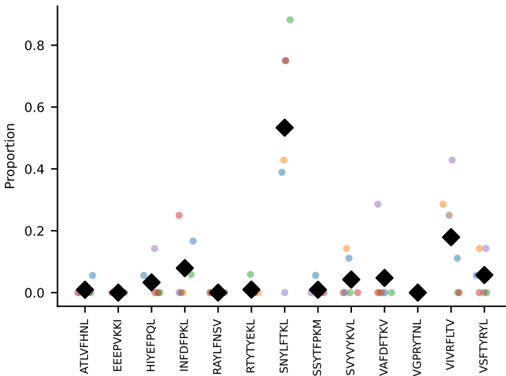
#9 AV16N-CAMREGNSNNRIFF-AJ31_BV13-1-CASRDINTEVFF-BJ1-1 coh=0.610, n=6
