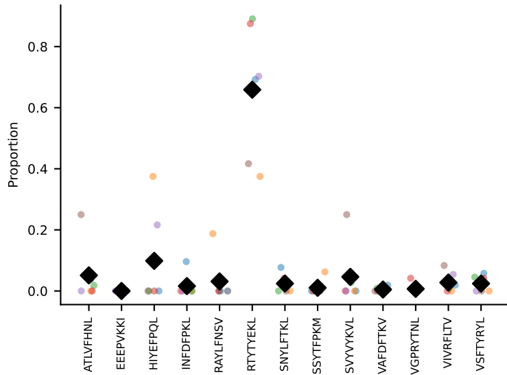
#6 AV16-CAMREANTGYQNFYF-AJ49_BV13-2-CASGTGGQNTLYF-BJ2-4 coh=0.622, n=19
