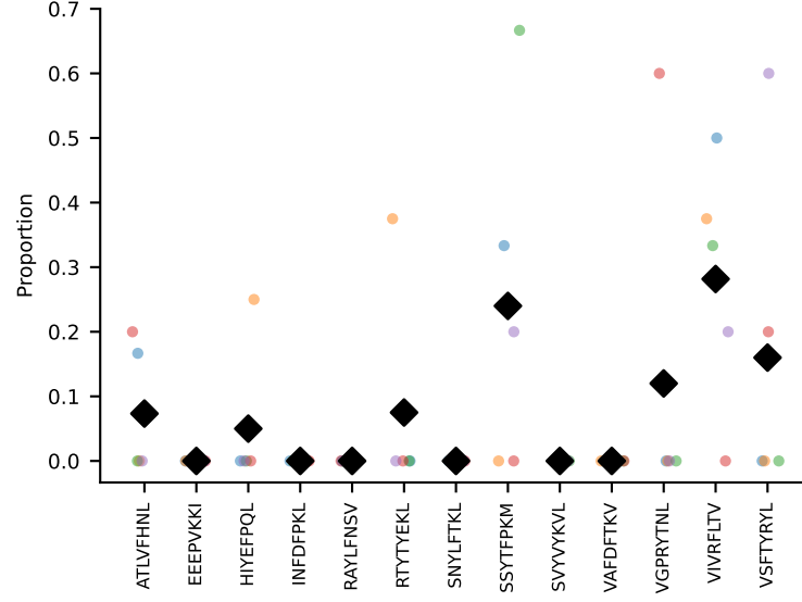
#47 AV8D-2-CATDNQGGRALIF-AJ15_BV19-CASSIGTSGNTLYF-BJ1-3 coh=0.299, n=5
