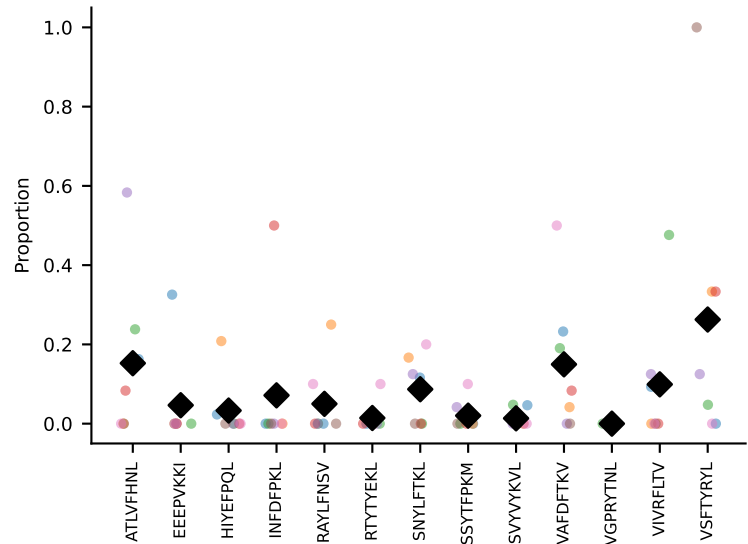
#42 AV4D-3-CAAENNYAQLTF-AJ26_BV1-CTCSADRLNTLYF-BJ2-4 coh=0.259, n=10
