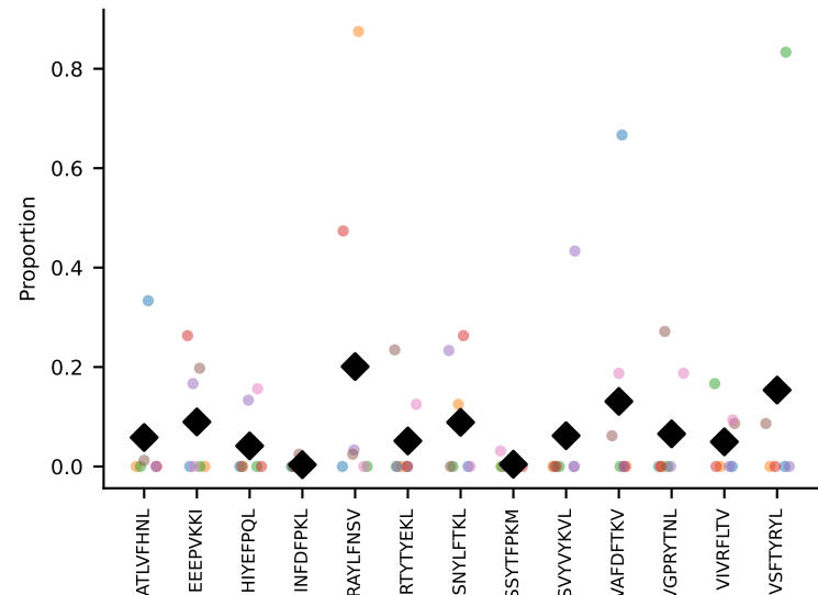
#82 AV16-CAMRETGYQNIFYF-AJ49_BV13-1-CASSDAYTEVFF-BJ1-1 coh=0.179, n=27
