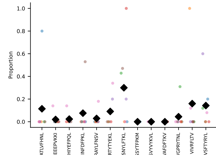
#77 AV7-3-CAVSPGGYKVVVF-AJ12_BV13-2-CASGDAQGAGQLYF-BJ2-2 coh=0.186, n=13
