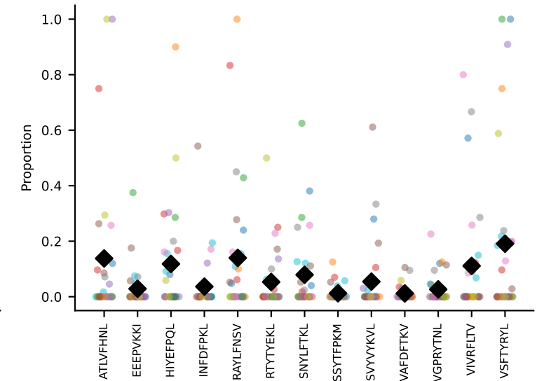
#44 AV14-2-CAASADQGGRALIF-AJ15_BV16-CASSLDHSQNTLYF-BJ2-4 coh=0.258, n=8
