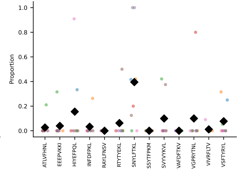
#48 AV13D-4-CAMELDSNYQLIW-AJ33_BV4-CASHGSYNSPLYF-BJ1-6 coh=0.250, n=9
