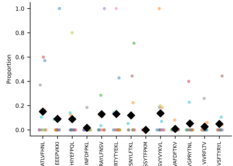
#84 AV16N-CAMREYVQGGRALIF-AJ15_BV16-CASSFVGNQDTQYF-BJ2- coh=0.176, n=12
