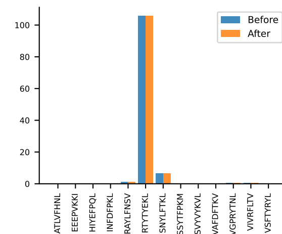
AV8-2-CATNTGNYKYVF-AJ40_BV1-CTCSAGGLGSTGQLYF-BJ2-2 MEAN n:6→6
