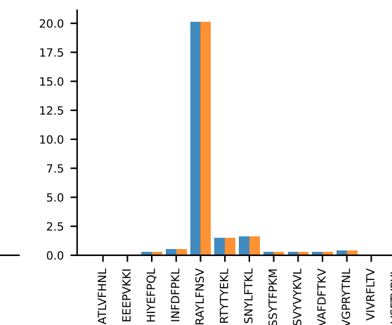
AV6-3-CAMRSNNYNVLYF-AJ21_BV13-2-CASGDAGVNQDTQYF-BJ2-5 MEAN n:6→6
