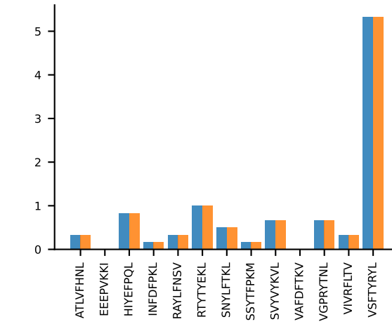
AV3D-3-CAVESSNTNKVVF-AJ34_BV13-2-CASGRDRAQNTLYF-BJ2-2 MEAN n:6→6
