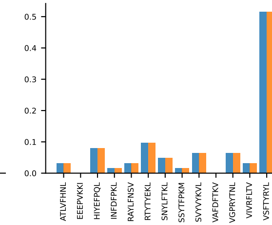
AV3D-3-CAVESSNTNKVVF-AJ34_BV13-2-CASGRDRAQNTLYF-BJ2-2 PROP n:6→6
