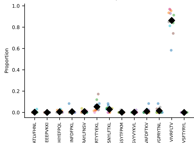
#10 AV6-6-CALGDQGTGSKLSF-AJ58_BV13-1-CASKDTYEYQYF-BJ2-7 coh=0.975, n=8
