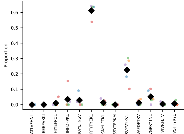
#19 AV16/DV11-CAMRESNTGYQNfYF-AJ49_BV13-2-CASGEGQGKNTLYF-BJ2-4 coh=0.957, n=8
