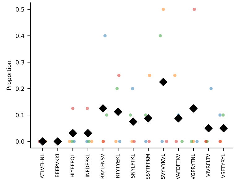
#57 AV16N-CAMREGQAYKVIF-AJ30_BV13-2-CASGGRAQDTQYF-BJ2-5 coh=0.399, n=10
