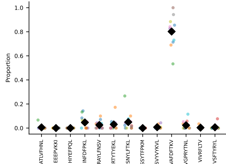
#17 AV6D-7-CALGDTGANTGKLTf-AJ52_BV17-CASSRAGWGGYEQYF-BJ2-7 coh=0.961, n=4
