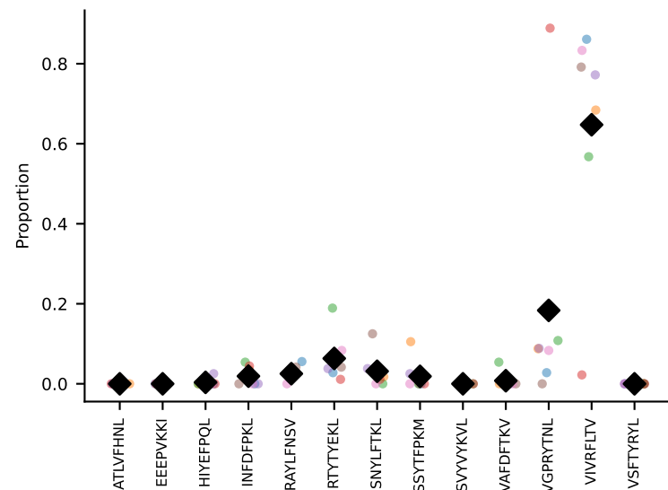
#42 AV6-5-CAPSNTNKVVf-AJ34_BV19-CASSITYQDTQYF-BJ2-5 coh=0.677, n=4
