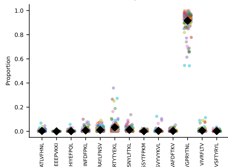
#9 AV7D-5-CAVSMTNSAGNKLTF-AJ17_BV13-3-CASSDAGQAERLFF-BJ1-4 coh=0.982, n=8
