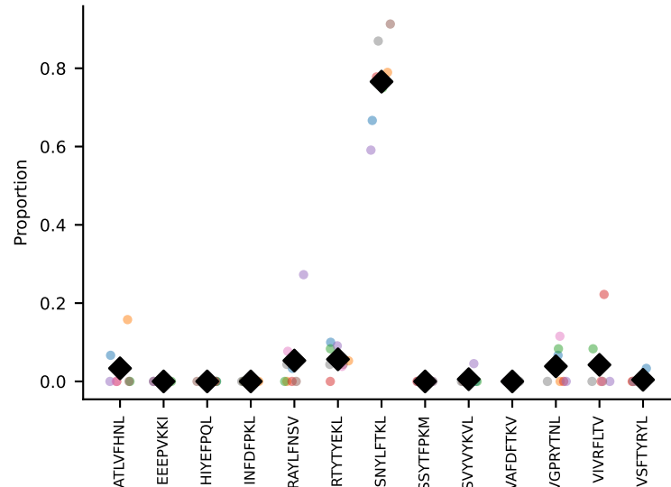
#23 AV6-6-CALGASNTEGADRLTF-AJ45_BV13-3-CASSDRDLYF-BJ2-4 coh=0.937, n=37
