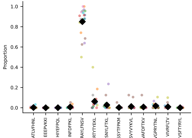
#20 AV4-2-CAVEGTGGYKVF-AJ12_BV13-1-CASSAGADSPLYF-BJ1-6 coh=0.950, n=14
