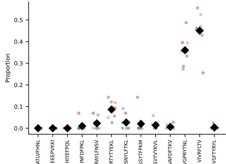
#22 AV9-2-CAPIASSFSKLVF-AJ50_BV13-2-CASGDVGGANERLFF-BJ1-4 coh=0.943, n=7
