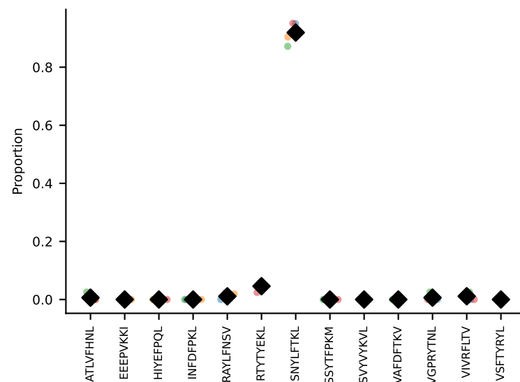
#6 AV17-CALGNNAGAKLTF-AJ39_BV17-CASSRQGAREQYF-BJ2-7 coh=0.989, n=13
