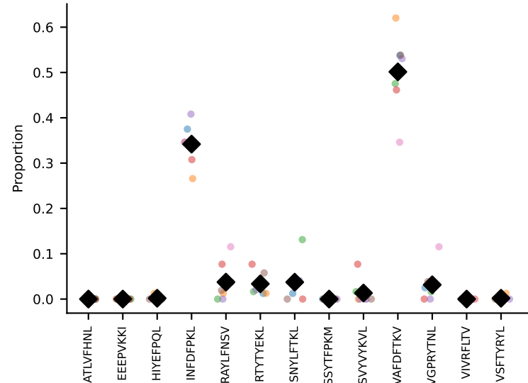
#18 AV17-CALGNNAGAKLTf-AJ39_BV13-1-CASSILGGSYEQYF-BJ2-7 coh=0.959, n=18
