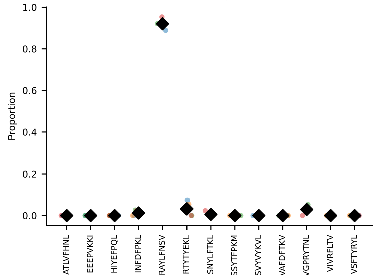
#7 AV5-4-CAASSNSGGSNAKLTF-AJ42_BV3-CASSLGQISNERLFF-BJ1-4 coh=0.987, n=14
