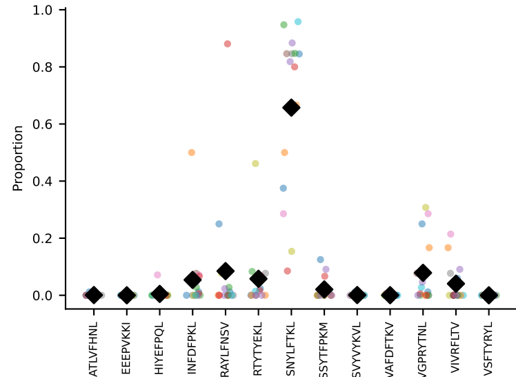
#44 AV7-2-CAASRGDYANKMIF-AJ47_BV13-3-CASSARVEQYF-BJ2-7 coh=0.605, n=5
