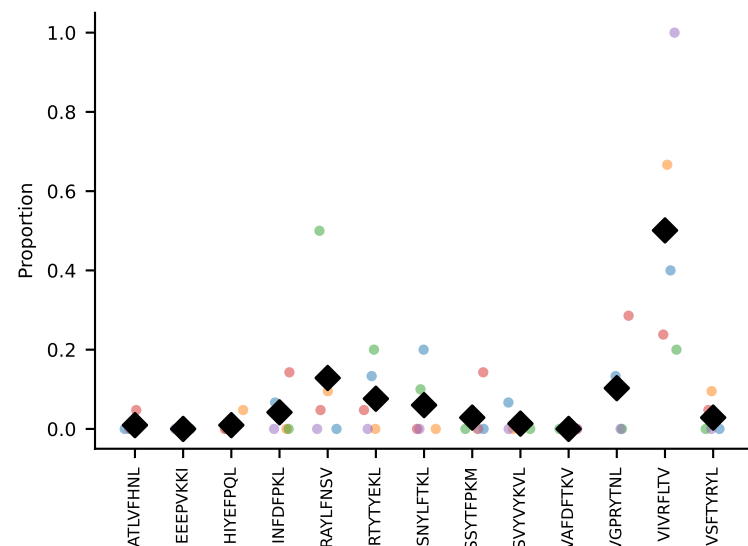
#48 AV7D-5-CAGTQVVGQLTf-AJ5_BV13-1-CASSGTGMYEQYF-BJ2-7 coh=0.570, n=4
