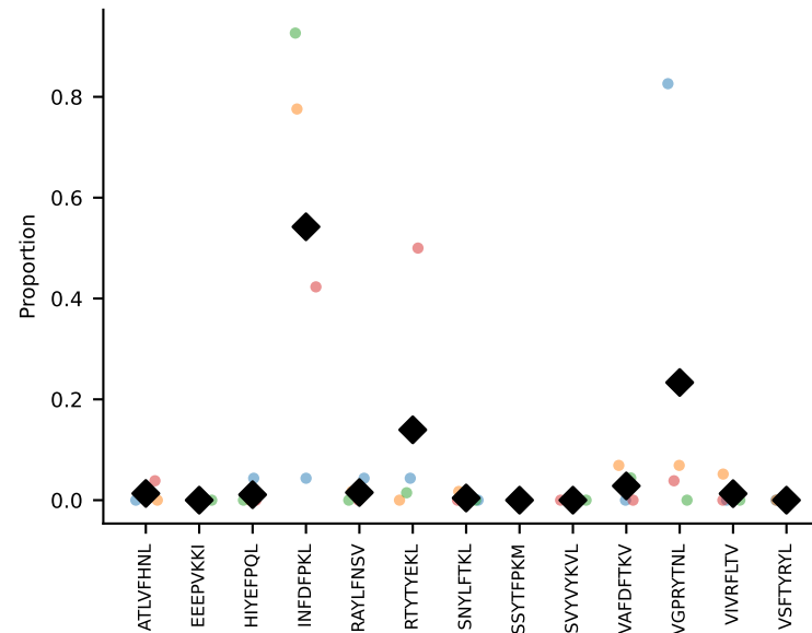
#55 AV3D-3-CAVRGGSGGKLTf-AJ44_BV13-3-CASSGGPTGQLYF-BJ2-2 coh=0.436, n=4
