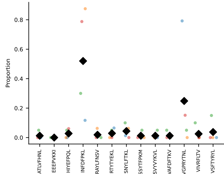
#54 AV7D-3-CAVTGNYKYVF-AJ40_BV14-CASSLRGEQYF-BJ2-7 coh=0.437, n=5
