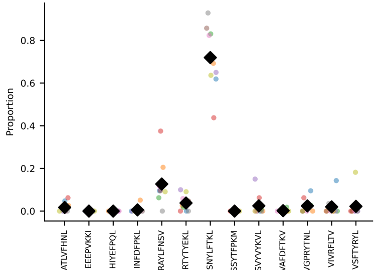
#24 AV13-4/DV7-CAMERGGSSNAKLTf-AJ42_BV13-2-CASGEGQGKNTLYF-BJ2-4 coh=0.932, n=9
