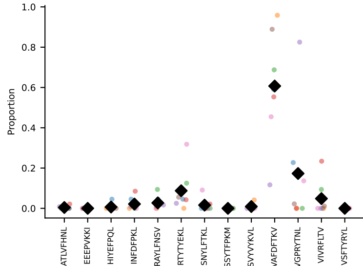
#43 AV16/DV11-CAMREGGGYKVVf-AJ12_BV4-CASSRDWYEQYF-BJ2-7 coh=0.645, n=4
