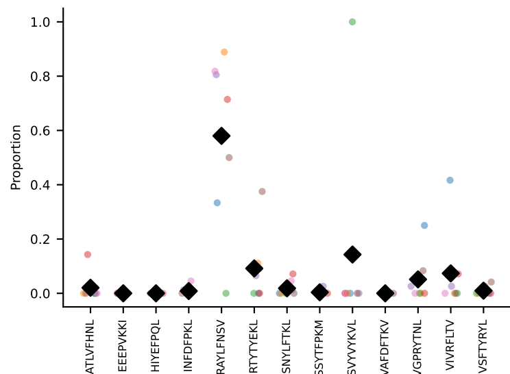
#47 AV14-2-CAARSAGNKLTf-AJ17_BV1-CTCSAVRANSDYTF-BJ1-2 coh=0.574, n=7
