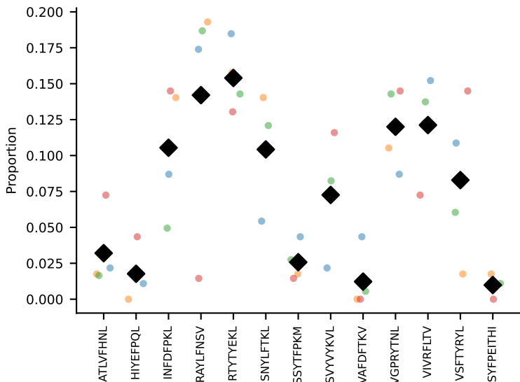
coh=0.814, n=4
