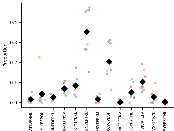
coh=0.794, n=6
