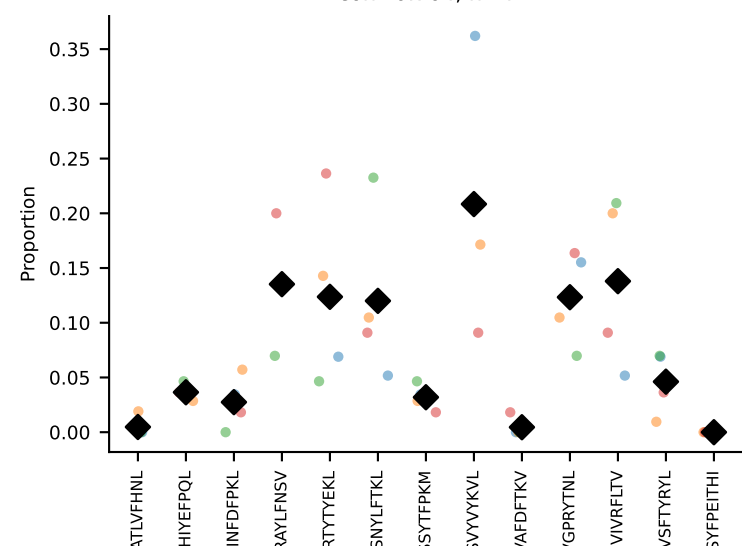
coh=0.764, n=4
