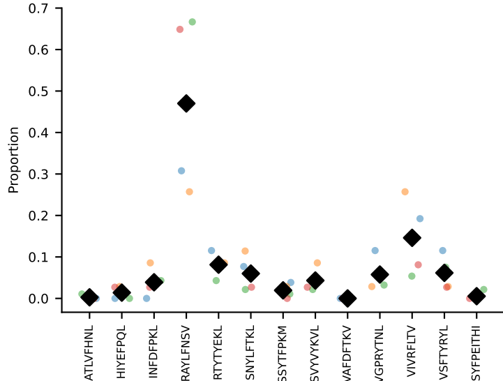
coh=0.779, n=4
