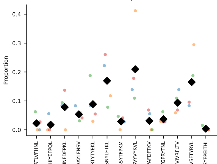
coh=0.746, n=4
