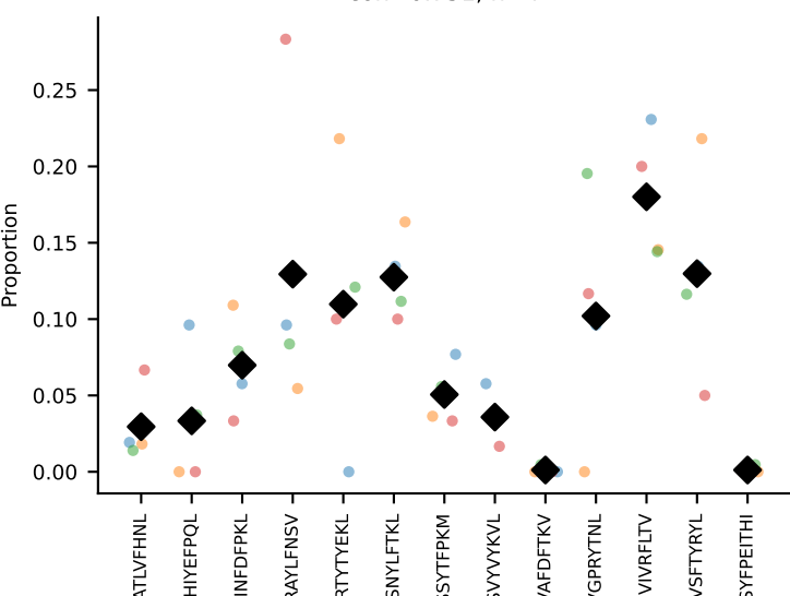
coh=0.751, n=4
