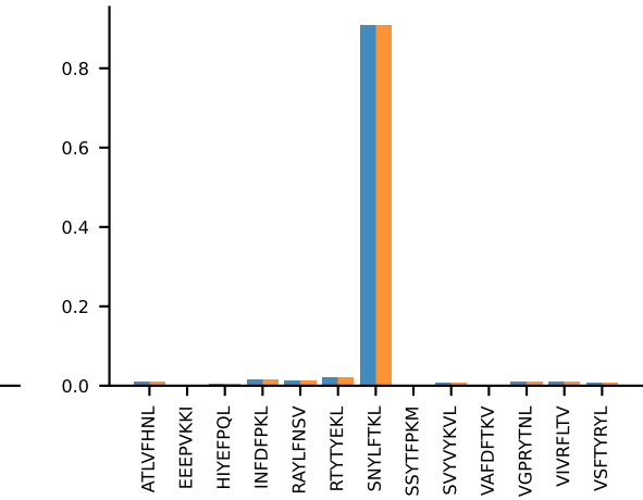
AV16N-CAMREVSNNVLYF-AJ21_BV13-2-CASGDQNGSGNTLYF-BJ1-1AV16N-CAMREVSNNVLYF-AJ21_BV13-2-CASGDQNGSGNTLYF-BJ1-1
