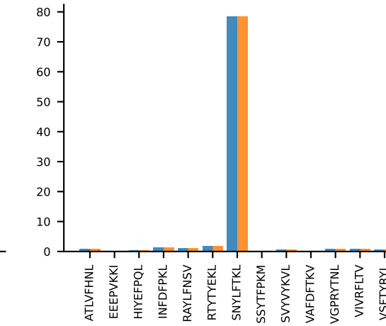
AV16N-CAMREVSNNVLYF-AJ21_BV13-2-CASGDQNGSGNTLYF-BJ1-1AV16N-CAMREVSNNVLYF-AJ21_BV13-2-CASGDQNGSGNTLYF-BJ1-1
