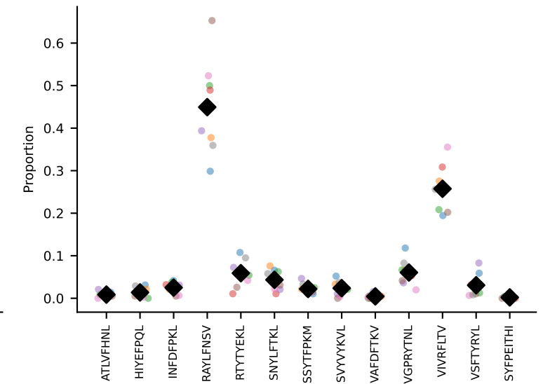
#44 AV15-1/DV6-1-CALWELASSNTDKVVF-AJ34*P03_BV3-CASSFGTGGYYEQ-BJ2-5 coh=0.955, n=10
