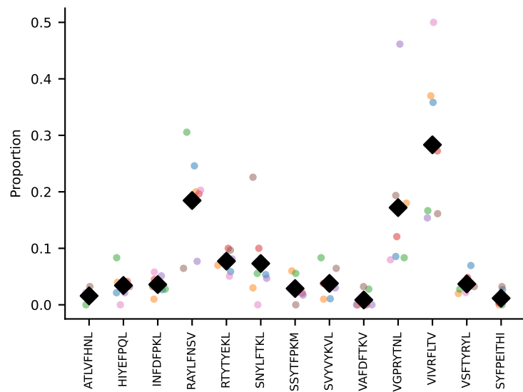
#126 AV3-3-CAVDTNAYKVIF-AJ30_BV13-2-CASGDGGREQYF-BJ2-7 coh=0.745, n=15
