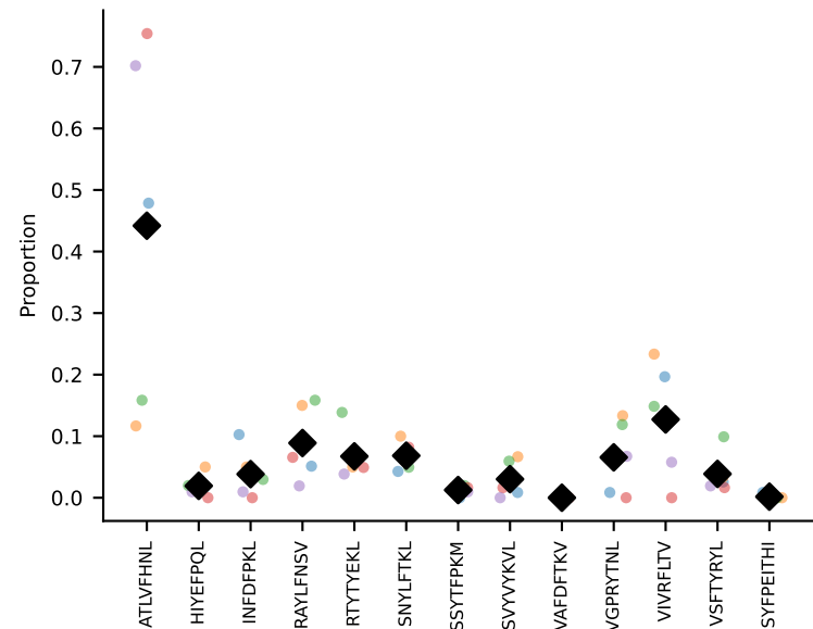
#140 AV16/DV11-CAMREDSSGGSNYKLTFF-AJ53_BV13-2-CASGGAGNSPLYF-BJ2-7 coh=0.331, n=5
