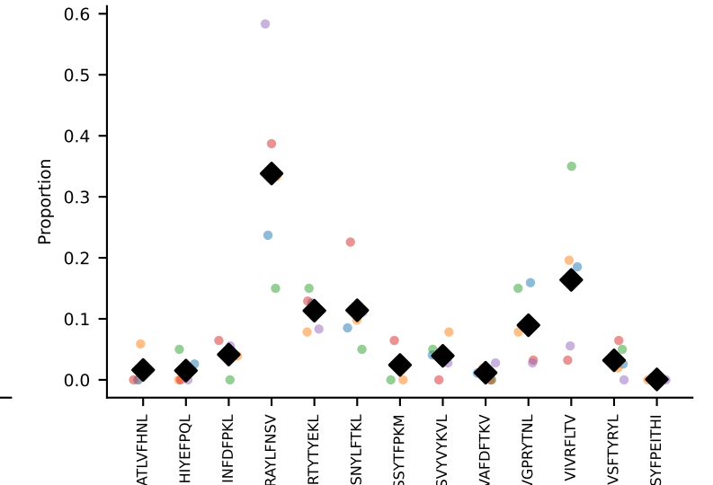
#119 AV13-1-CAMNQGSsAKLIF-AJ57_BV1-CTCSALNYAEQFF-BJ2-1-#120 AV16D/DV11-CAMRDTNAYKVIf-AJ30_BV13-2-CASGDVGGGQNTLYf-BJ2-5 coh=0.768, n=5
