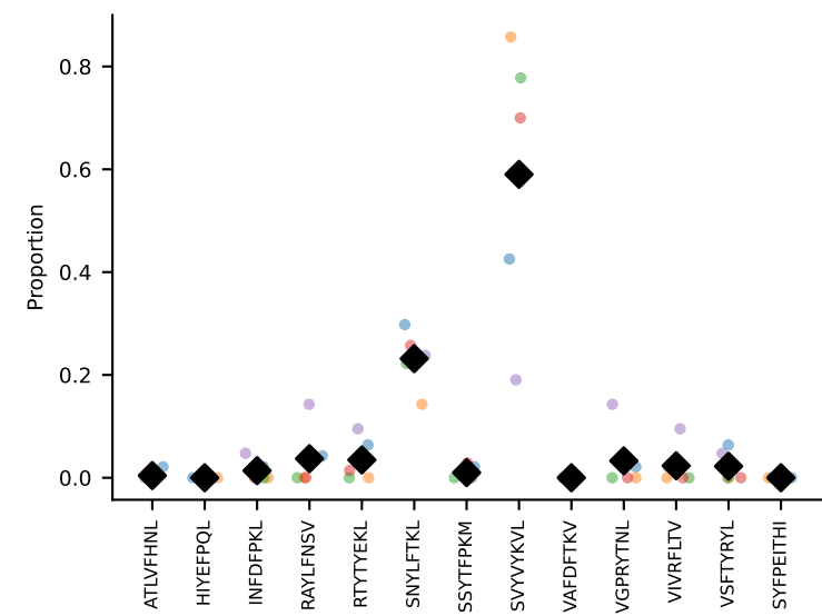
#186 AV6D-7-CALSDMGYKLTF-AJ9_BV13-2-CASGDVDSYNSPLYF-BJ1-3 coh=0.835, n=5
