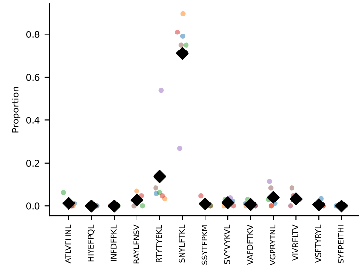
#124 AV6-4-CALVPDYANKMIF-AJ47_BV13-3-CASSDRGQVFF-BJ1-1 coh=0.830, n=6
