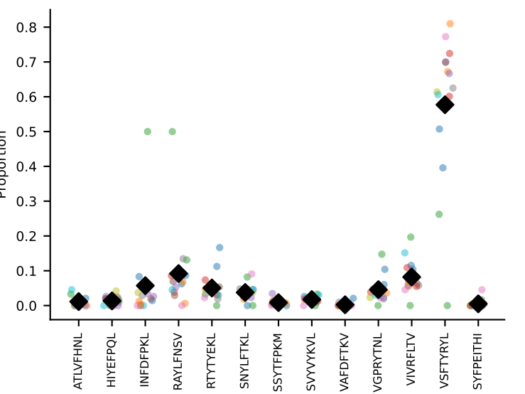
#87 AV7-4-CADNTNTGKLTF-AJ27_BV12-2-CASSLEQGEDTQYF-BJ2-5 coh=0.830, n=18
