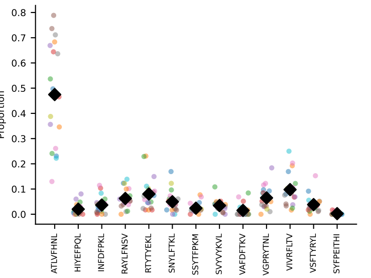
#190 AV6D-6-CALSDRGNTNTGKLTF-AJ27_BV29-CASTPGLQDTQYF-BJ2-5 coh=0.828, n=6
