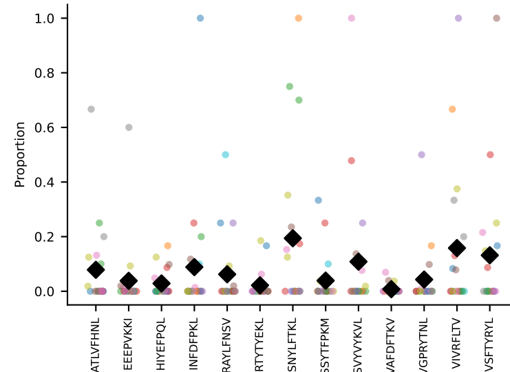
#106 AV17-CALEGSGYGNEKITF-AJ48_BV1-CTCSGDRVSIEQYF-BJ2-7 coh=0.240, n=12
