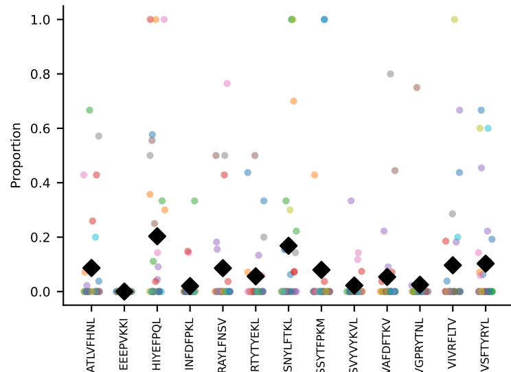
#139 AV7-3-CAVSAEGADRLTF-AJ45_BV1-CTCSADRGGNSPLYF-BJ1-1 coh=0.196, n=28
