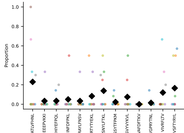
#140 AV15D-2/DV6D-2-CALSELRDRGSALGRLHF-AJ18_BV4-CASSPTGKVFF coh=0.196, n=8
