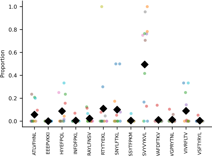
#236 AV9-4-CAVSAAGTGSNRLTF-AJ28_BV1-CTCSADWGVWAETLYF-BJ2-3 coh=0.455, n=6
