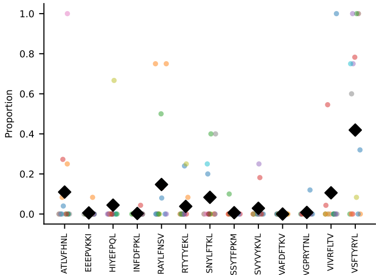
#70 AV6N-6-CALSATSSGQKLIV-AJ16_BV23-CSSSQSQTTNTEVFF-BJ1-1 coh=0.297, n=31
