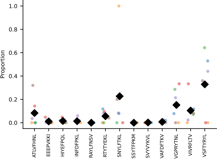
#238 AV6-2-CVLGSNMGYKLTF-AJ9_BV29-CASSLGRGVNQAPLF-BJ1-5 coh=0.448, n=7
