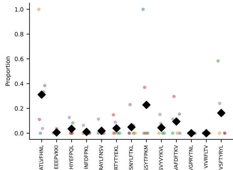
#271 AV8D-2-CATDNSNNRIFF-AJ31_BV5-CASSQGLGYAEQFF-BJ2-1 coh=0.323, n=6
