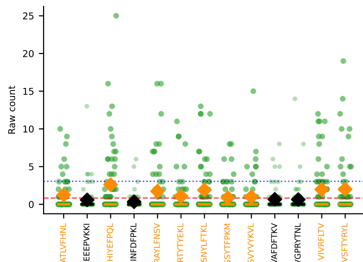
#91 AV16N-CAMREGNNAGAKLTf-AJ39_BV16-CASSSGQKNTVEFF-BJ1-1 SINGLE | Above BG: none n=65 [D7C:65] thresh=3.0
