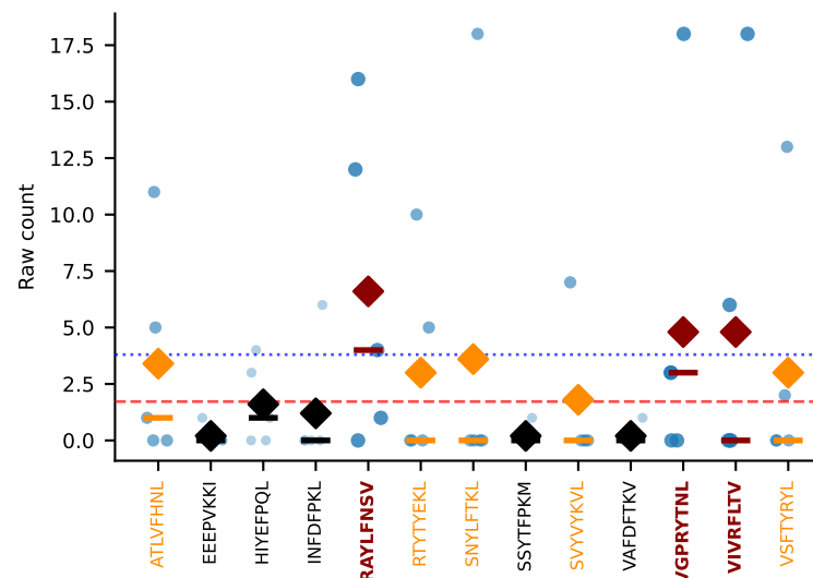
#276 AV13D-2-CAIDYNQGLKIF-AJ23_BV1-CTCSAVRISGNTLYF-BJ1-3 MULTI-SPECIFIC | Above BG: RAYLFNSV+VGPRYTNL+1more n=5 [D7A:5] thresh=3.8
