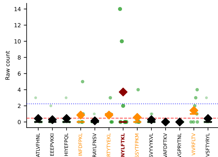
#88 AV8D-2-CATDAMNTGGLSGKLTf-AJ2_BV13-1-CASSPGQYAEQFF-BJ2-1 SINGLE | Above BG: SNYLF TKL n=7 [D7C:7] thresh=2.2
