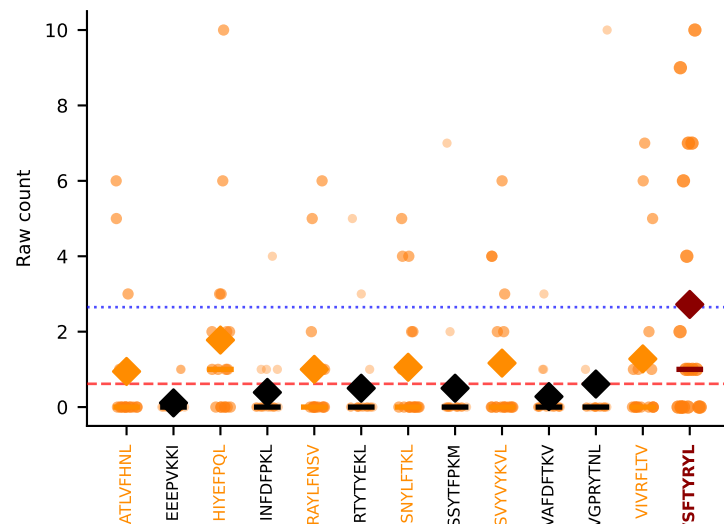
#87 AV8N-2-CATDHQGGRALIF-AJ15_BV29-CASSSGTSGNTLYF-BJ1-3 SINGLE | Above BG: VSFTYRYL n=18 [D7B:18] thresh=2.6
