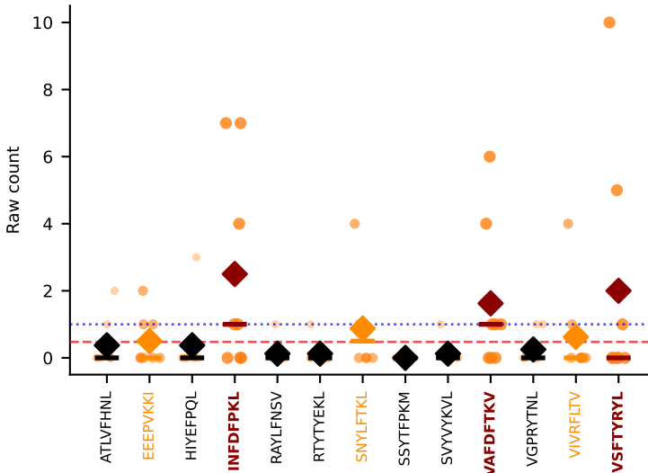
#293 AV13-1-CALEGRGSNYQLTF-AJ53_BV14-CASSSRYEQYF-BJ2-7 MULTI-SPECIFIC | Above BG: INFDFPKL+VAFDFTKV+1more n=8 [D7B:8] thresh=1.0
