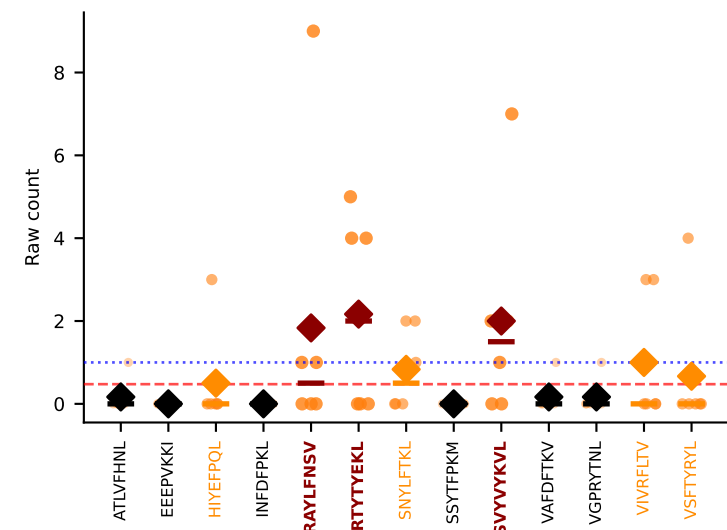
#273 AV12D-3-CALFYQGGRALIF-AJ15_BV13-1-CASSEGGREQYF-BJ2-7 MULTI-SPECIFIC | Above BG: RAYLFNSV+RTTYEKL+1more n=6 [D7B:6] thresh=1.0
