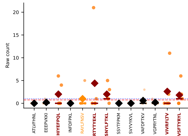
#268 AV9D-3-CAVSMQGGSAKLIF-AJ57_BV13-3-CASDRGRDTQYF-BJ2-5 MULTI-SPECIFIC | Above BG: HIYEFPL+RTTYEKL+3more n=5 [D7B:5] thresh=1.0
