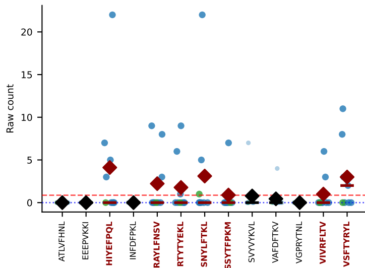
#317 AV13-1-CALGTNSAGNKLTF-AJ17_BV2-CASSQDRVYEQYF-BJ2-7 MULTI-SPECIFIC | Above BG: HIYEPQL+RAYLFNSV+5more n=9 [D7A:8, D7C:1] thresh=0.0
