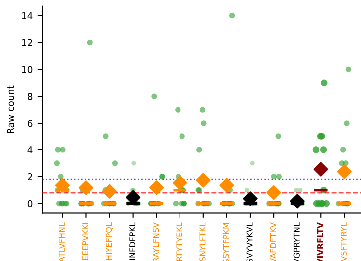
#90 AV19-CAANQGGSAKLIF-AJ57_BV5-CASSRQVNYAEQFF-BJ2-1 SINGLE | Above BG: VIVRFLTV n=11 [D7C:11] thresh=1.8
