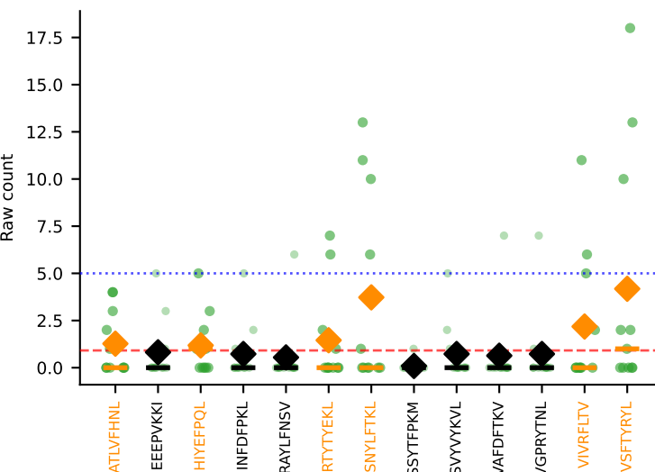
#96 AV8-1-CATDYDTNAYKVIF-AJ30_BV13-2-CASGDPIRNERLFF-BJ1-4 SINGLE | Above BG: none n=11 [D7C:11] thresh=5.0
