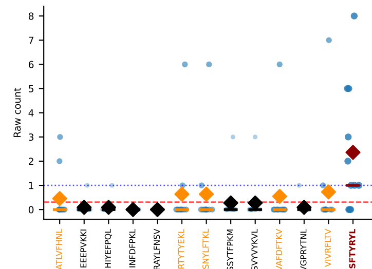
#94 AV6-6-CALGMSNYNVLYF-AJ21_BV13-2-CASGDEGPQDTQYF-BJ2-5 SINGLE | Above BG: VSFTYRYL n=11 [D7A:11] thresh=1.0
