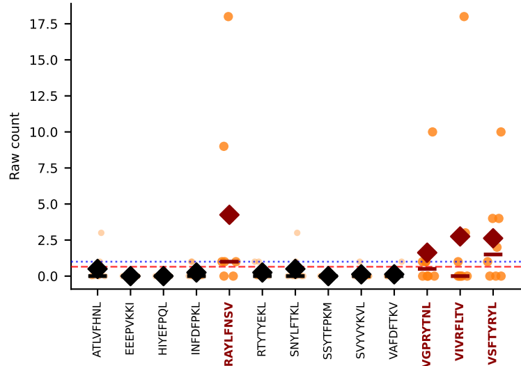
#290 AV12-2-CALSDRDSAGNKLTF-AJ17_BV13-3-CASSDRLNTGQLYF-BJ2-2 MULTI-SPECIFIC | Above BG: RAYLFNSV+VGPRYTNL+2more n=8 [D7B:8] thresh=1.0
