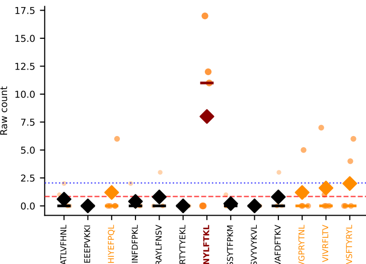
#92 AV15-1/DV6-1-CALWELNNYAQGLTf-AJ26_BV13-1-CASSDAGAEVFF-BJ1-1 SINGLE | Above BG: SNYLF TKL n=5 [D7B:5] thresh=2.0
