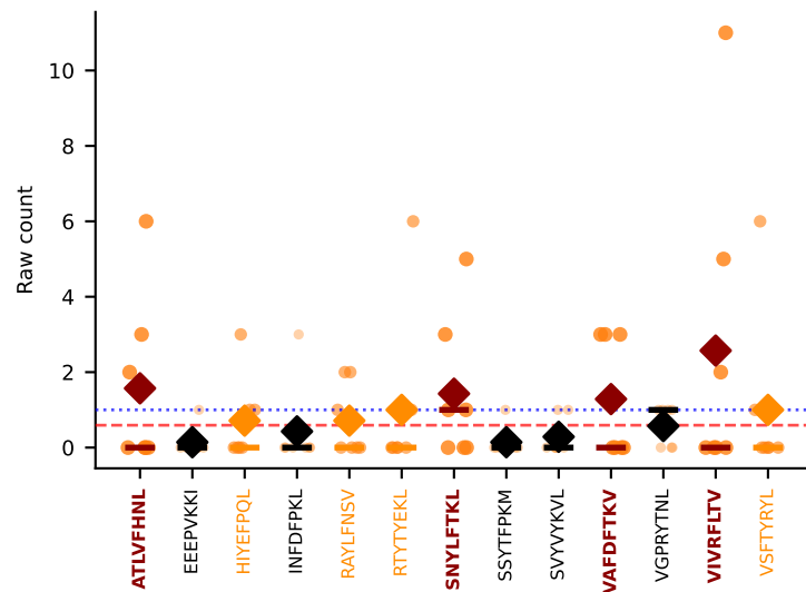
#320 AV19-CATNQGGSAKLIF-AJ57_BV5-CASSQOGNYAEQFF-BJ2-1 MULTI-SPECIFIC | Above BG: ATLVFHNL+SNYLFTKL+2more n=7 [D7B:7] thresh=1.0
