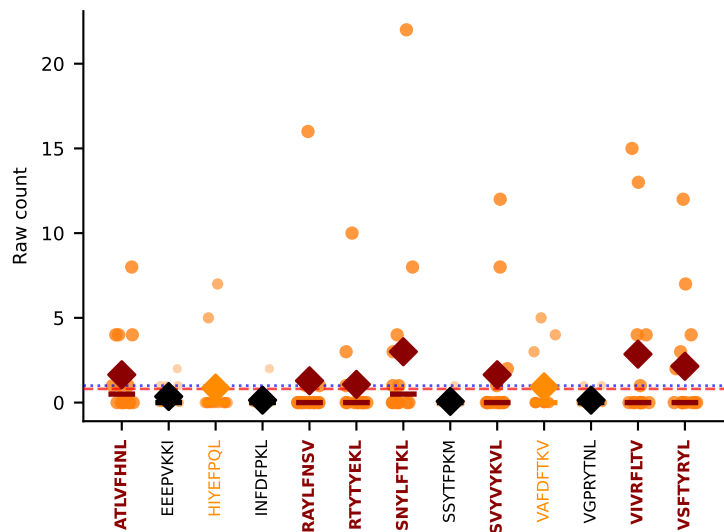
#313 AV9D-3-CALYGSSGNKLIF-AJ32_BV29-CASSLRVHEQYF-BJ2-7 MULTI-SPECIFIC | Above BG: ATLVFHNL+RAYLFNSV+5more n=14 [D7B:14] thresh=1.0
