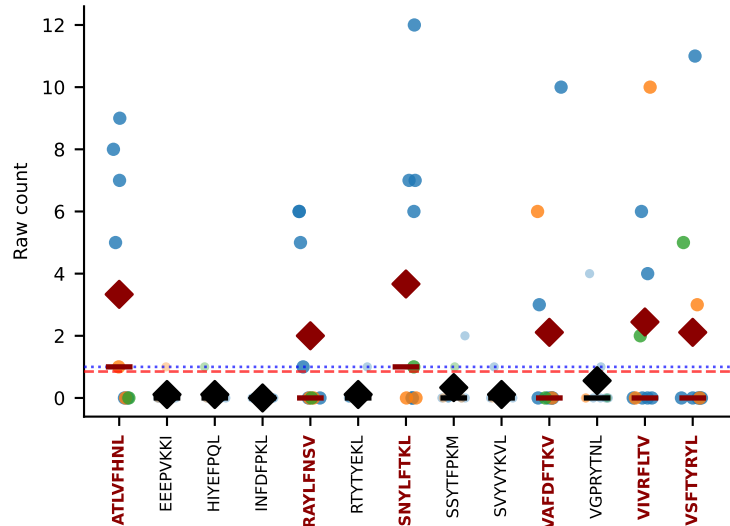
#294 AV16N-CAMREGDSNYQLIW-AJ33_BV13-2-CASGDRANSDYTF-BJ1-2 MULTI-SPECIFIC | Above BG: ATLVFHNL+RAYLFNSV+4more n=9 [D7A:6, D7B:2, D7C:1] thresh=1.0
