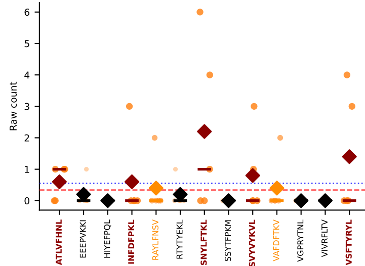
#289 AV3D-3-CAVSGSGSWQLIF-AJ22_BV13-3-CASSDRTTGGFSYEQYF-BJ2-7 MULTI-SPECIFIC | Above BG: ATLVFHNL+INFDFPKL+3more n=5 [D7B:5] thresh=0.5
