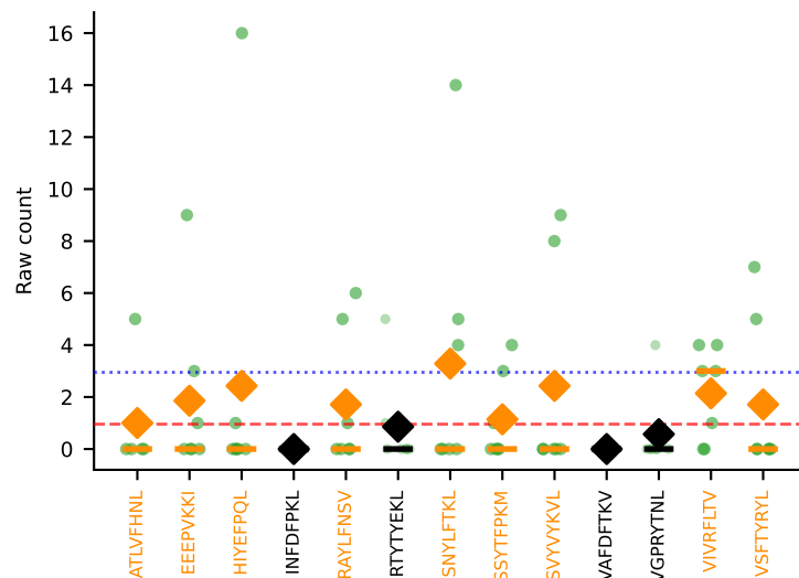
#86 AV8D-2-CATTGQGGRALIF-AJ15_BV19-CASSPGTGGETEVFF-BJ1-1 SINGLE | Above BG: none n=7 [D7C:7] thresh=2.9
