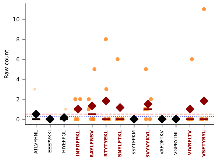
#322 AV12-3-CALSDSGSFNKLTF-AJ4_BV14-CASSLRGQQYF-BJ2-7 MULTI-SPECIFIC | Above BG: INFDFPKL+RAYLFNSV+5more n=6 [D7B:6] thresh=0.2
