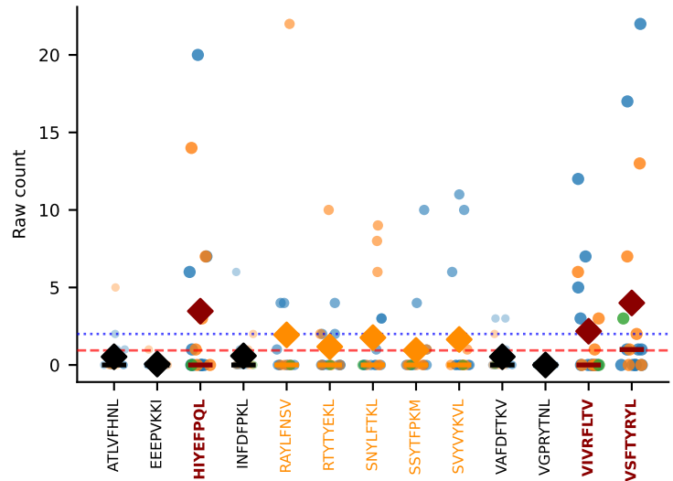
#300 AV12-2-CALNQGGSAKLIF-AJ57_BV1-CTCSADWGNYAEQFF-BJ2-1 MULTI-SPECIFIC | Above BG: HIYEPQL+VIVRFLTV+1more n=17 [D7A:10, D7B:6, D7C:1] thresh=2.0
