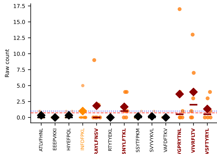
#272 AV10-CAASADYANKMIF-AJ47_BV3-CASSLAGQGYEQYF-BJ2-7 MULTI-SPECIFIC | Above BG: RAYLFNSV+SNYLFTKL+3more n=6 [D7B:6] thresh=1.0
