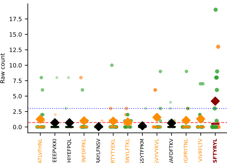
#93 AV14D-3/DV8-CAASASSGSWQLIF-AJ22_BV31-CAWSPLQGANTVEFF-BJ1-1 SINGLE | Above BG: VSFTYRYL n=16 [D7B:5, D7C:11] thresh=3.0
