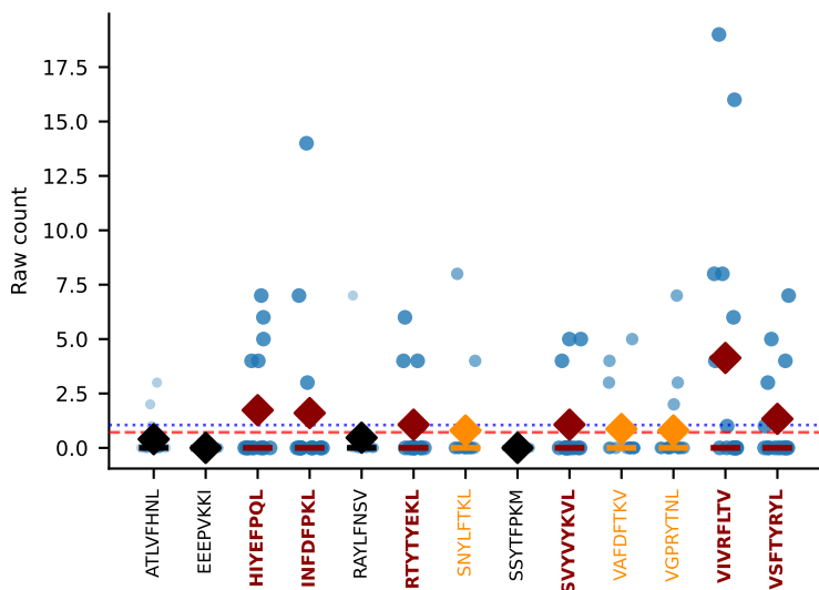
#321 AV13D-2-CAIDRQGGRALIF-AJ15_BV13-1-CASSRTGVNOAPLF-BJ1-5 MULTI-SPECIFIC | Above BG: HIYEPQL+INFDFPKL+4more n=15 [D7A:15] thresh=1.0
