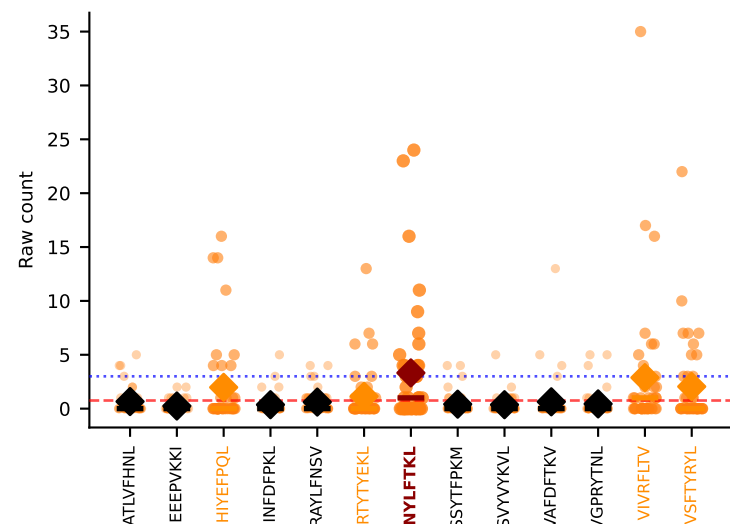
#89 AV7-5-CAVGGSGGKLTf-AJ44_BV4-CASSLGRHTEVFF-BJ1-1 SINGLE | Above BG: SNYLF TKL n=41 [D7B:41] thresh=3.0
