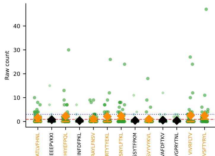
#95 AV14-2-CAAGASSGSWQLIF-AJ22_BV31-CAWSLAGSGNTLYF-BJ1-3 SINGLE | Above BG: none n=41 [D7A:2, D7C:39] thresh=3.0
