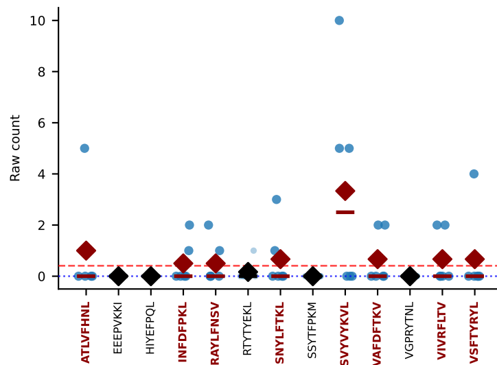
#314 AV14D-1-CAASAGGSAKLIF-AJ57_BV12-2-CASSLGQGAGAEQFF-BJ2-1 MULTI-SPECIFIC | Above BG: ATLVFHNL+INFDFPKL+6more n=6 [D7A:6] thresh=0.0
