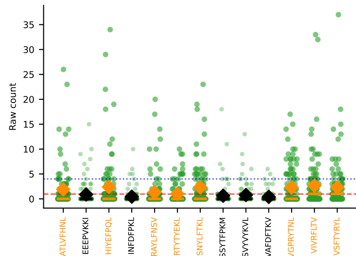
#85 AV8D-2-CATDGTNKKVF-AJ34_BV3-CASSLAREYEQYF-BJ2-7 SINGLE | Above BG: none n=107 [D7C:107] thresh=4.0
