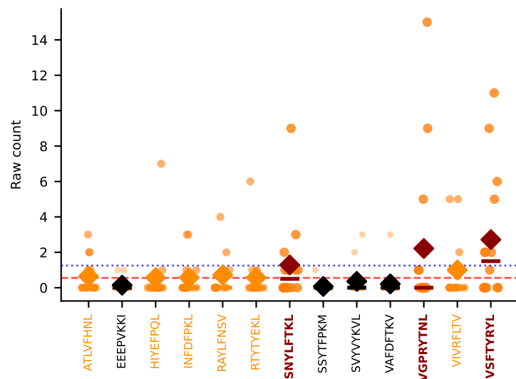
#324 AV7-5-CAVSMPGNTGKLIF-AJ37_BV4-CASSWGNYAEQFF-BJ2-1 MULTI-SPECIFIC | Above BG: SNYLFTKL+VGPRYTNL+1more n=14 [D7B:14] thresh=1.2
