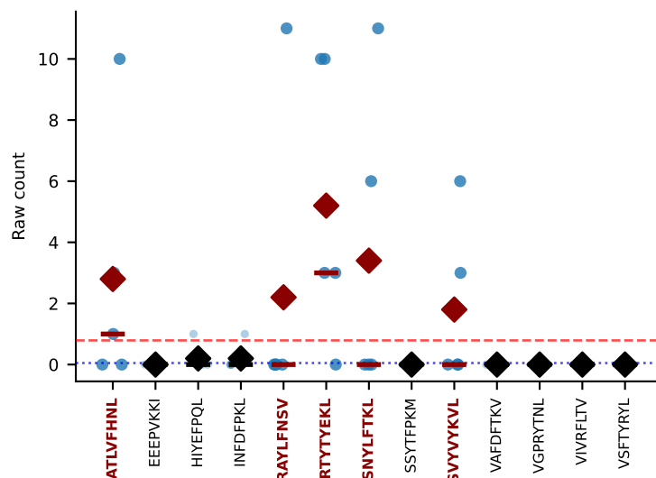
#270 AV10N-CAASPNYNVLYF-AJ21_BV13-1-CASSDVGQDQTQYF-BJ2-5 MULTI-SPECIFIC | Above BG: ATLVFHNL+RAYLFNSV+3more n=5 [D7A:5] thresh=0.0
