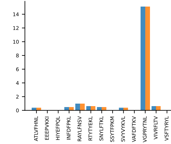
AV10-CAASLDTNAYKVIF-AJ30_BV13-2-CASGGQTVEVFF-BJ1-1AV10-CAASLDTNAYKVIF-AJ30_BV13-2-CASGGQTVEVFF-BJ1-1
