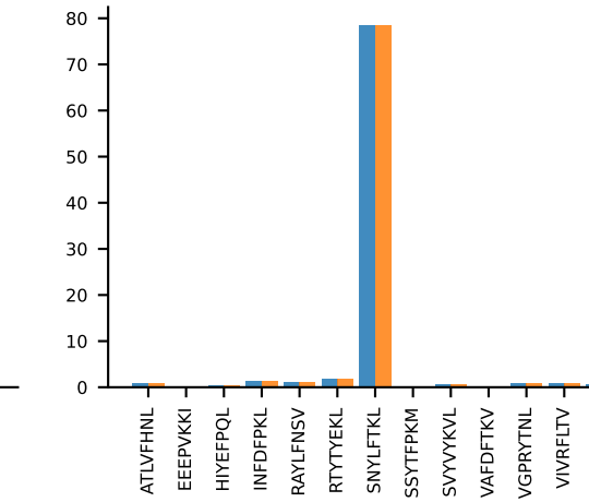
AV16N-CAMREVSNYNVLYF-AJ21_BV13-2-CASGDQGNsgNTLYF-BJ1-1AV16N-CAMREVSNYNVLYF-AJ21_BV13-2-CASGDQGNsgNTLYF-BJ1-1
