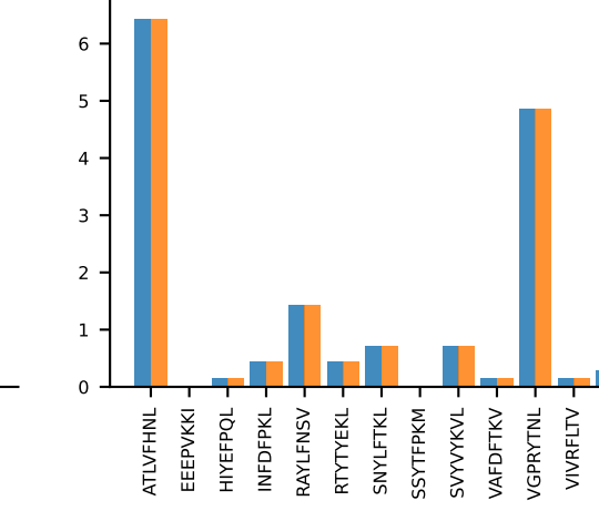
AV5-6-CALGNQGGSAKLIF-AJ57_BV12-2-CASSPDWGEdTOYF-BJ1-1AV5-6-CALGNQGGSAKLIF-AJ57_BV12-2-CASSPDWGEdTOYF-BJ1-1
