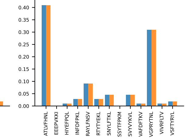
AV5-6-CALGNQGGSAKLIF-AJ57_BV12-2-CASSPDWGEdTOYF-BJ1-1AV5-6-CALGNQGGSAKLIF-AJ57_BV12-2-CASSPDWGEdTOYF-BJ1-1
