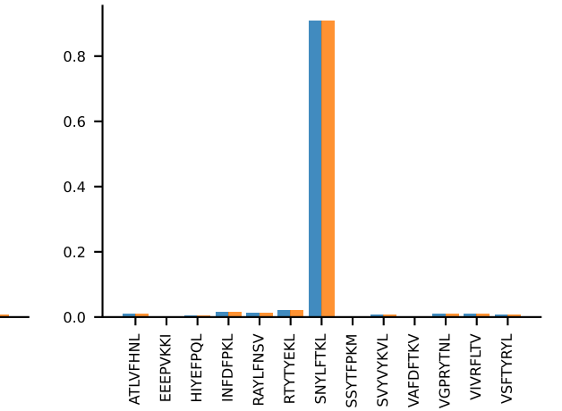
AV16N-CAMREVSNYNVLYF-AJ21_BV13-2-CASGDQGNsgNTLYF-BJ1-1AV16N-CAMREVSNYNVLYF-AJ21_BV13-2-CASGDQGNsgNTLYF-BJ1-1
