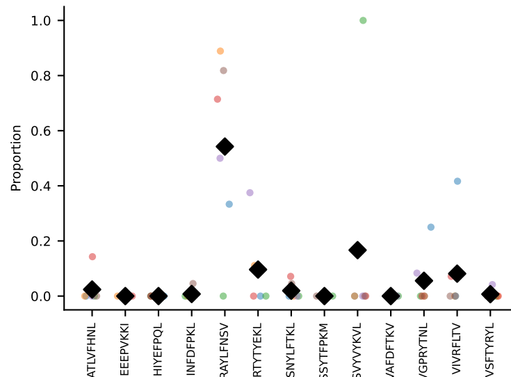
#223 AV8N-2-CATEDQGGRALIF-AJ15_BV5-CASSQEASNERLFF-BJ1-4 coh=0.472, n=6
