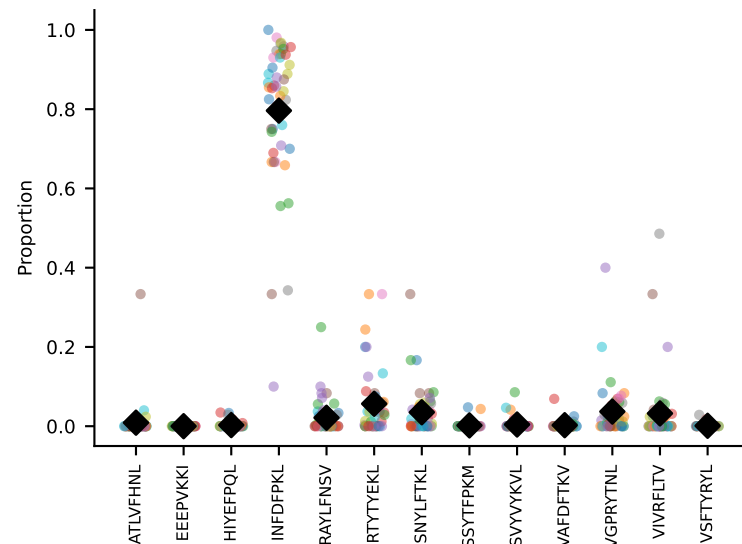
#130 AV8-1-CATEGYQNIFYF-AJ49_BV12-1-CASSLTGGYEYQF-BJ2-7 coh=0.905, n=45
