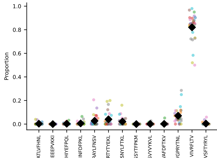
#66 AV9-4-CAVRWDYANKMIF-AJ47_BV3-CASSLSYEQYF-BJ2-7 coh=0.966, n=120
