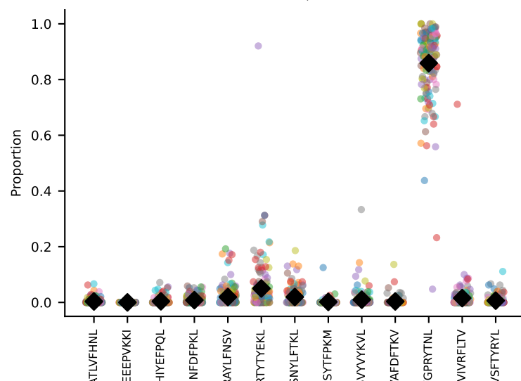
#71 AV7-5-CAVSMDYANKMIF-AJ47_BV3-CASSLAAYEQYF-BJ2-7 coh=0.961, n=149
