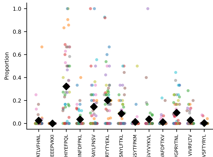
#227 AV3-3-CAVSASNAGAKLTF-AJ39_BV5-CASSPDRGDERLFF-BJ1-4 coh=0.455, n=55
