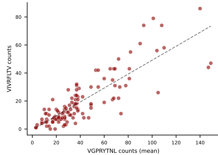
VIVRFLTV r=0.841 , p=3.50\text{e-}32
