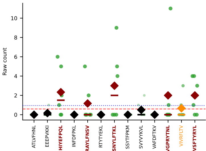
#316 AV13D-2-CAIDTNTGKLTF-AJ27_BV26-CASSLDRAITGQLYF-BJ2-2 MULTI-SPECIFIC | Above BG: HIYEPQL+RAYLFNSV+3more n=6 [D7C:6] thresh=0.9
