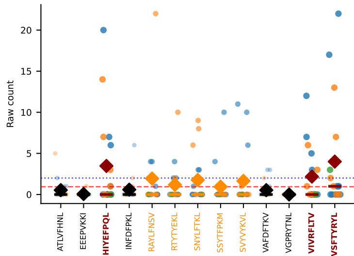
#300 AV12-2-CALNQGGSAKLIF-AJ57_BV1-CTCSADWGNIAEQFF-BJ2-1 MULTI-SPECIFIC | Above BG: HIYEPQL+VIVRFLTV+1more n=17 [D7A:10, D7B:6, D7C:1] thresh=2.0
