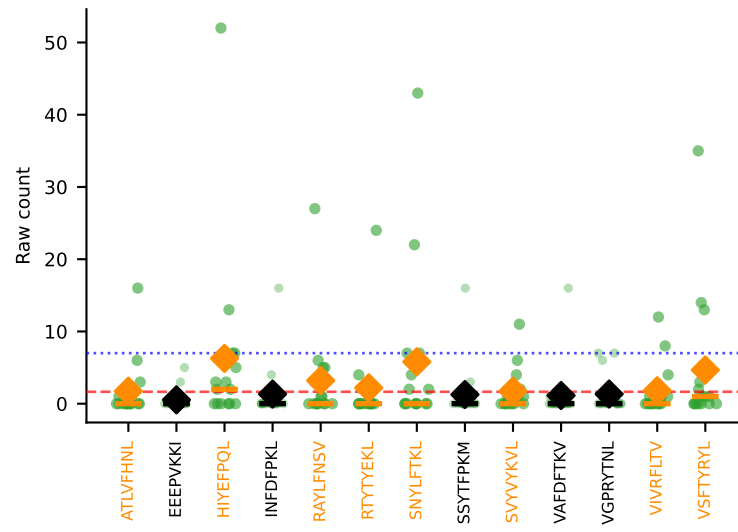
#71 AV7N-4-CAVSEDGRSALGR LHF-AJ18_BV1-CTCSAGGDYAEQFF-BJ2-1 SINGLE | Above BG: none n=15 [D7C:15] thresh=7.0
