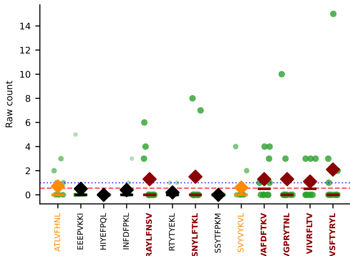
#346 AV7D-6-CAGNYSNNRLTL-AJ7_BV16-CASSLNWGANAYAEQFF-BJ2-1 MULTI-SPECIFIC | Above BG: RAYLFNSV+SNYLFTKL+4more n=10 [D7C:10] thresh=1.0
