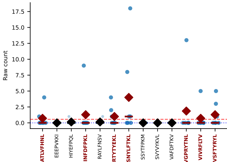
#341 AV7-1-CAVKGNNNAPRF-AJ43_BV13-2-CASRLGGYEQYF-BJ2-7 MULTI-SPECIFIC | Above BG: ATLVFHNL+INFDFPKL+5more n=7 [D7A:7] thresh=0.0
