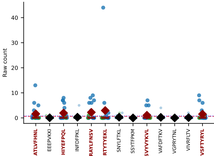
#340 AV12D-3-CALSDHYNQGLIF-AJ23_BV2-CASSQDISYEQYF-BJ2-7 MULTI-SPECIFIC | Above BG: ATLVFHNL+HIYEPQL+4more n=18 [D7A:16, D7C:2] thresh=0.8
