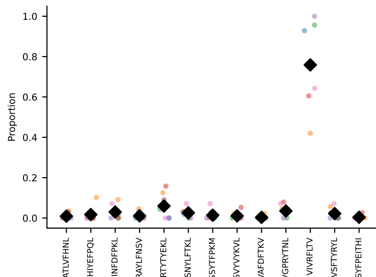
#35 AV9D-4-CALSATNAVIVf-AJ30_BV13-2-CASGDAAGKDTQYF-BJ2-5 coh=0.960, n=7
