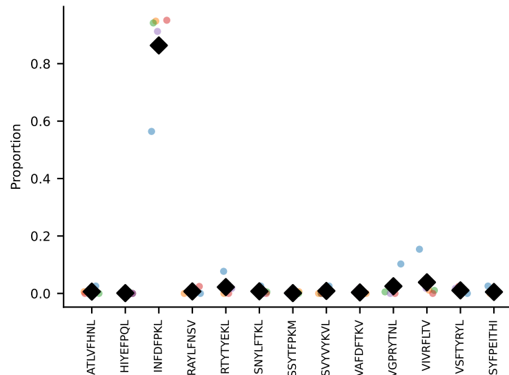
#31 AV7D-3-CAVIGSGSWQLIF-AJ22_BV13-2-CASGEPQGANSPLYF-BJ1-7 coh=0.972, n=26
