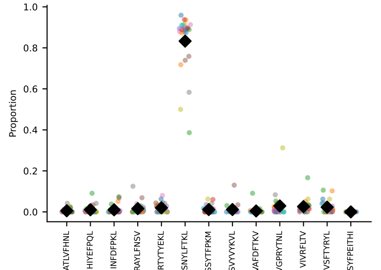
#36 AV16D/DV11-CAMREGYAQGLTf-AJ26_BV13-2-CASWDISGNTLYF-BJ2-2 coh=0.959, n=15
