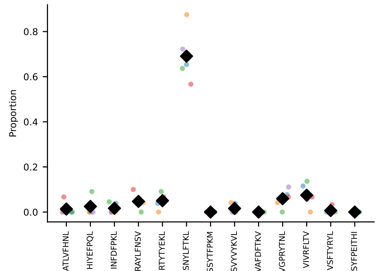
#32 AV16D/DV11-CAMREGVSAGNKLTf-AJ17*p02_BV13-1-CASSDVGAEQFF-BJ2-2 coh=0.970, n=25
