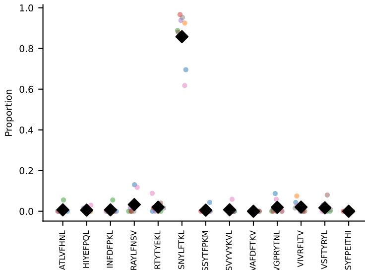
#29 AV12-2-CALSDLRTGGADRlTF-AJ45_BV13-1-CASSDVGAEQFF-BJ2-1 coh=0.973, n=8
