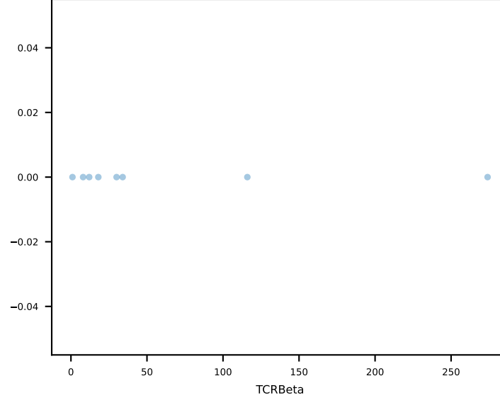
VIVRFLTV r=-0.14 p=0.73
