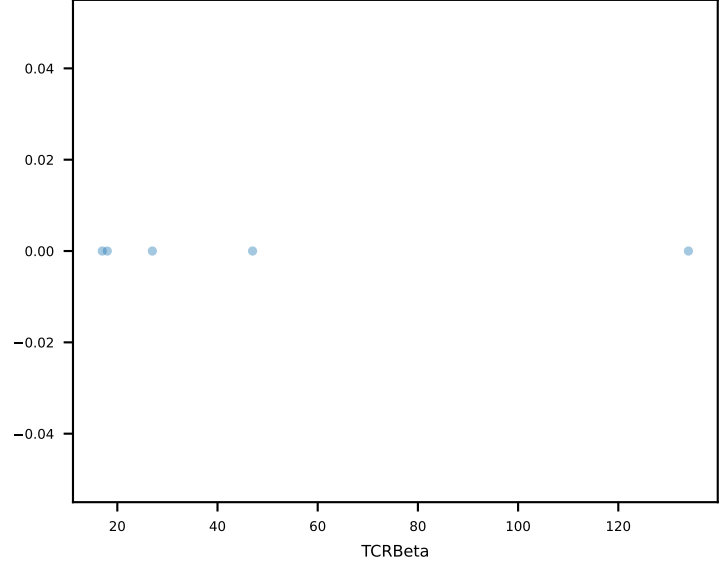
SVVYVKVL
