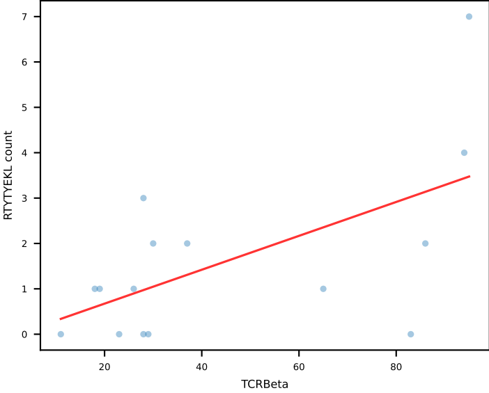
RTYTYEKL r=0.59 p=0.02
