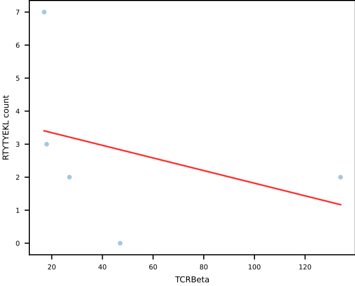
RTYTYEKL r=-0.36 p=0.55
