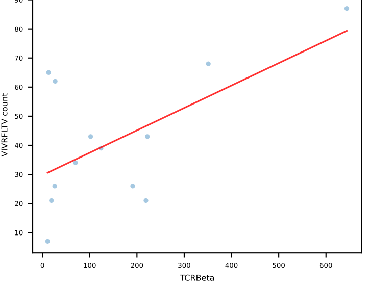
VIVRFLTV r=0.61 p=0.028
