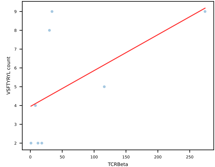
VSFTYRYL r=0.57 p=0.14
