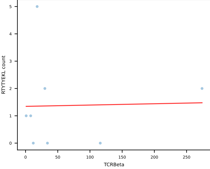
RTYTYEKL r=0.03 p=0.95
