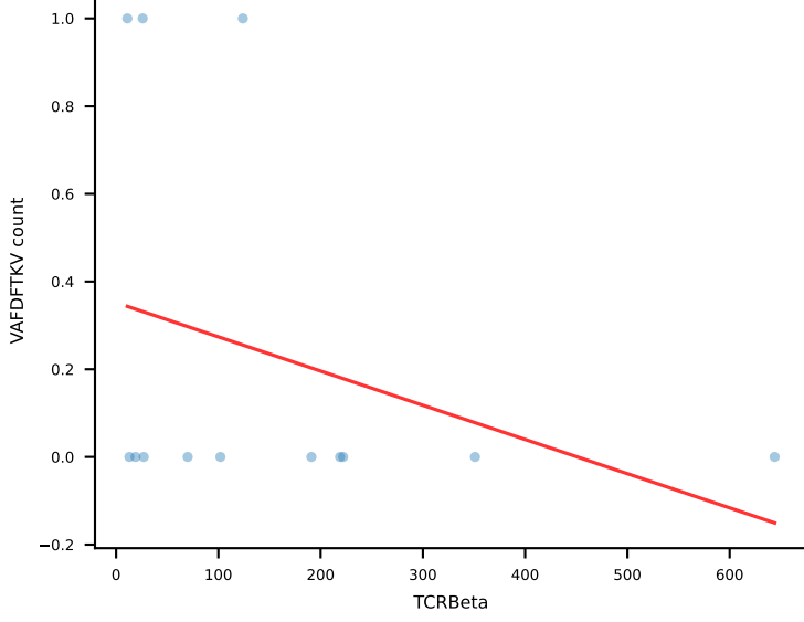
VAFDFTKV r=-0.32 p=0.28
