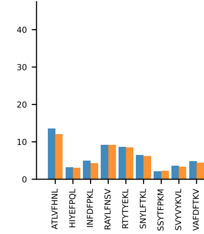
AV17-3-CAVDNTAYKVIF-AJ30_BV13-2-CASGDGGREQYF-BJ2-7 MEAN n:15→15
