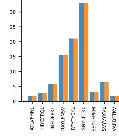
AV17-2-CALNTGYQNFYF-AJ49_BV13-1-CASSDAGGYEQYF-BJ2-7 MEAN n:13→13
