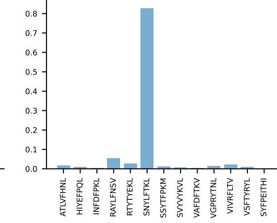
AV13-1-CAMEPGGNKLTf-AJ56_BV13-3-CASSDRYEQYf-BJ2-7 PROP n:5→0 LOST
