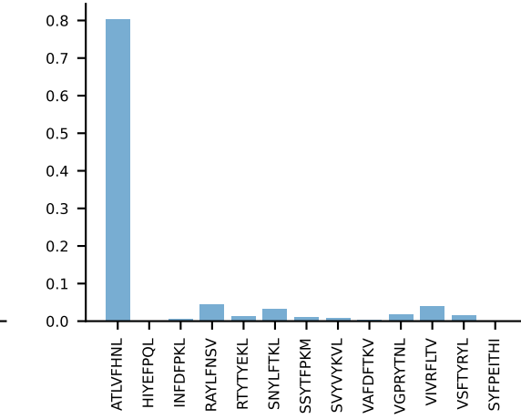
AV12-2-CALRASNTDKVfVf-AJ34*p03_BV1-CTCSADWDEQYf-BJ2-2 PROP n:5→0 LOST
