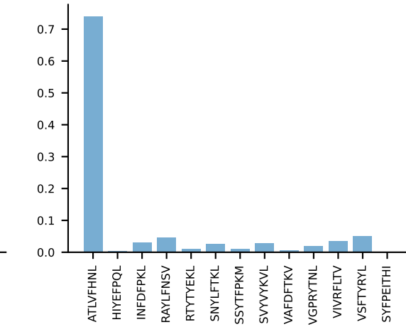
AV14D-1-CAASKDTGNYKYVf-AJ40_BV13-3-CASSDSNTEVFF-BJ1-1 PROP n:5→0 LOST
