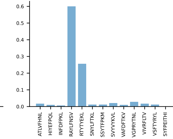
AV6-4-CALVTDYAQGLTf-AJ26_BV3-CASSLAFgDEQYf-BJ2-7 PROP n:5→0 LOST
