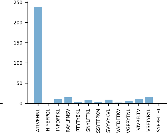
AV14D-1-CAASKDTGNYKYVf-AJ40_BV13-3-CASSDSNTEVFF-BJ1-1- AV14D-1-CAASKDTGNYKYVf-AJ40_BV13-3-CASSDSNTEVFF-BJ1-1 RAW n:5→0 LOST
