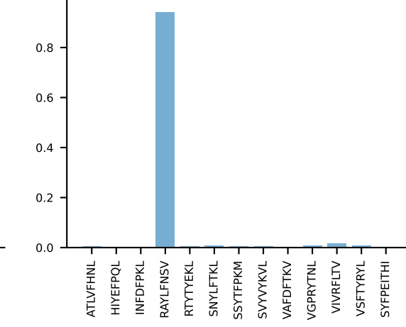
AV3-3-CAVSDPsgSWQLIF-AJ22_BV13-3-CASRGDRAEQYf-BJ2-7 PROP n:5→0 LOST
