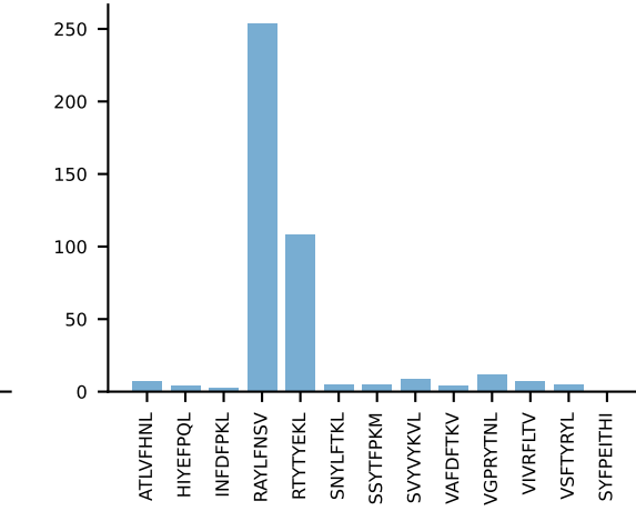
AV6-4-CALVTDYAQGLTf-AJ26_BV3-CASSLAFgDEQYf-BJ2-7- AV6-4-CALVTDYAQGLTf-AJ26_BV3-CASSLAFgDEQYf-BJ2-7 RAW n:5→0 LOST
