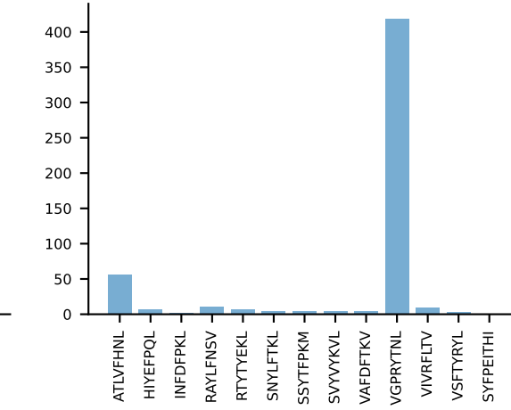
AV13-1-CAMERSSSGwQLIF-AJ22_BV4-CASSYGEQYf-BJ2-7- AV13-1-CAMERSSSGwQLIF-AJ22_BV4-CASSYGEQYf-BJ2-7 RAW n:5→0 LOST
