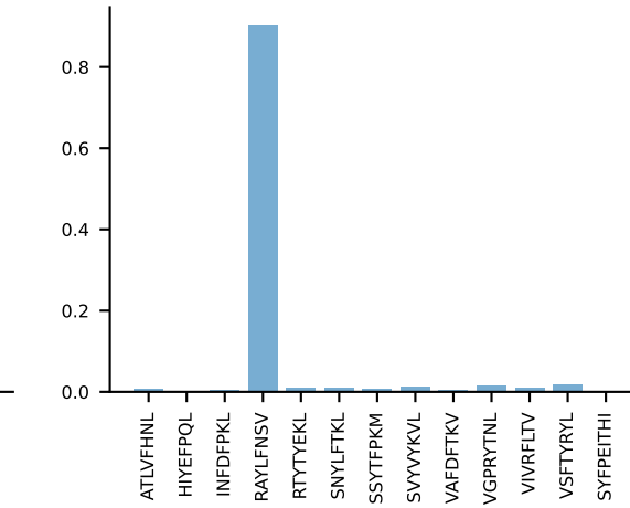
AV8-2-CATDATRMDYANKMIF-AJ47_BV3-CASSLARDYEQYf-BJ2-7 PROP n:5→0 LOST
