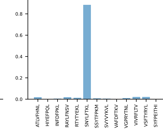
AV13D-2-CAIDPNYNVLYf-AJ21*p03_BV29-CASSPWGNTEVFF-BJ1-1 PROP n:5→0 LOST
