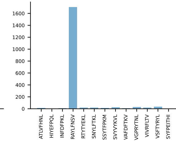
AV8-2-CATDATRMDYANKMIF-AJ47_BV3-CASSLARDYEQYf-BJ2-7AV8-2-CATDATRMDYANKMIF-AJ47_BV3-CASSLARDYEQYf-BJ2-7 RAW n:5→0 LOST
