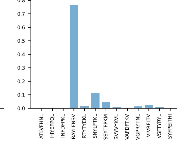
AV7D-2-CAASDYKvVf-AJ12_BV1-CTCSAVRVSGNTLYf-BJ1-3 PROP n:5→0 LOST
