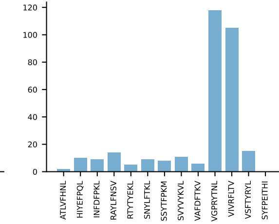
AV19-CAAGGQGGSAKLIf-AJ57_BV13-1-CASSDEQgAPNERLFF-BJ1-1- AV19-CAAGGQGGSAKLIf-AJ57_BV13-1-CASSDEQgAPNERLFF-BJ1-1 RAW n:5→0 LOST
