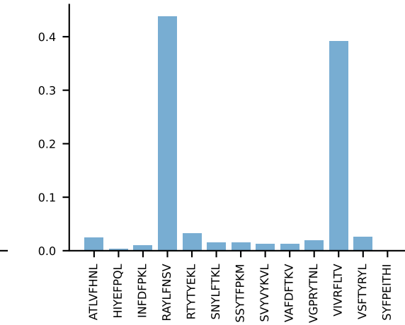
AV6D-4-CALAPDRIFF-AJ31_BV13-2-CASGDWGGNGTgQLYf-BJ2-2 PROP n:5→0 LOST
