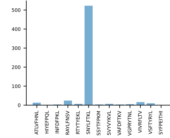
AV3-3-CAVSDPsgSWQLIF-AJ22_BV13-3-CASRGDRAEQYf-BJ2-7AV3-3-CAVSDPsgSWQLIF-AJ22_BV13-3-CASRGDRAEQYf-BJ2-7 RAW n:5→0 LOST
