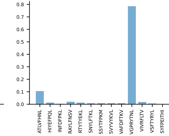
AV13-1-CAMERSSSGwQLIF-AJ22_BV4-CASSYGEQYf-BJ2-7 PROP n:5→0 LOST
