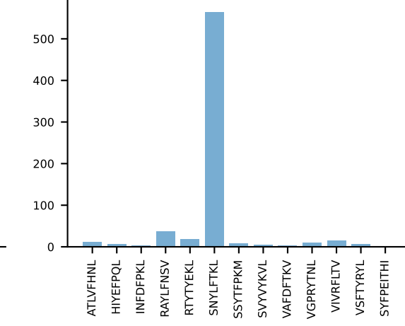
AV13-1-CAMEPGGNKLTf-AJ56_BV13-3-CASSDRYEQYf-BJ2-7- AV13-1-CAMEPGGNKLTf-AJ56_BV13-3-CASSDRYEQYf-BJ2-7 RAW n:5→0 LOST
