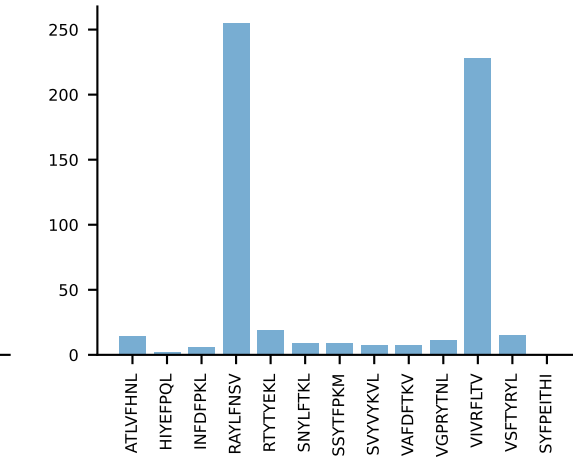
AV6D-4-CALAPDRIFF-AJ31_BV13-2-CASGDWGGNGTgQLYf-BJ2-2AV6D-4-CALAPDRIFF-AJ31_BV13-2-CASGDWGGNGTgQLYf-BJ2-2 RAW n:5→0 LOST
