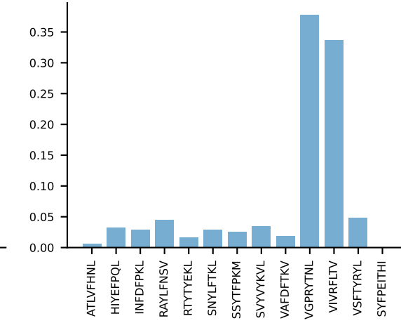
AV19-CAAGGQGGSAKLIf-AJ57_BV13-1-CASSDEQgAPNERLFF-BJ1-1 PROP n:5→0 LOST
