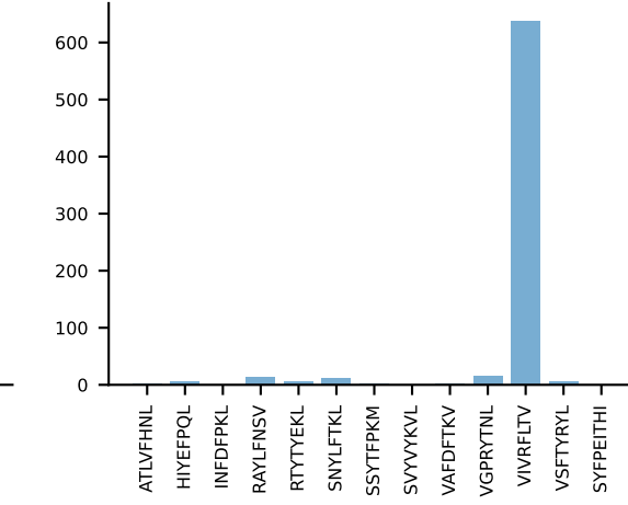
AV7D-2-CAASDYKvVf-AJ12_BV1-CTCSAVRVSGNTLYf-BJ1-3- AV7D-2-CAASDYKvVf-AJ12_BV1-CTCSAVRVSGNTLYf-BJ1-3 RAW n:5→0 LOST
