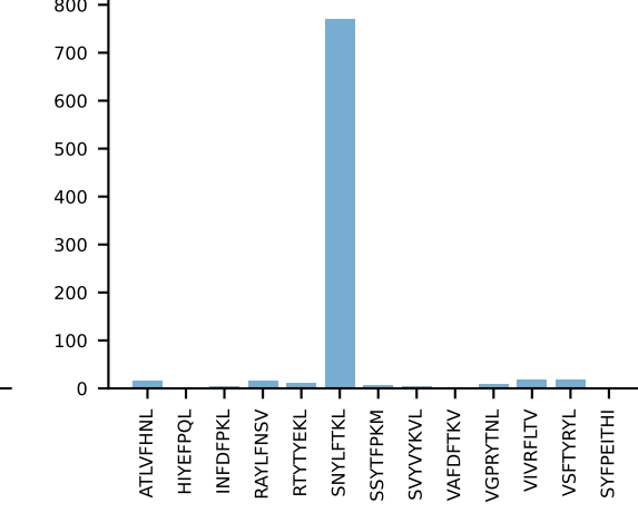
AV13D-2-CAIDPNYNVLYf-AJ21*p03_BV29-CASSPWGNTEVFF-BJ1-1AV13D-2-CAIDPNYNVLYf-AJ21*p03_BV29-CASSPWGNTEVFF-BJ1-1 RAW n:5→0 LOST
