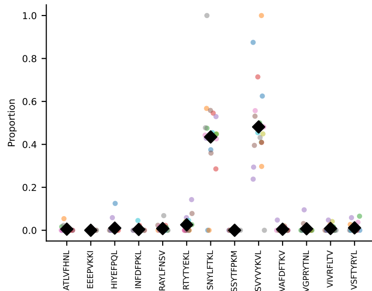
#15 AV16-CAMREANTGYQNIFYF-AJ49_BV13-2-CASGEGAQNTLYF-BJ2-4 coh=0.857, n=18
