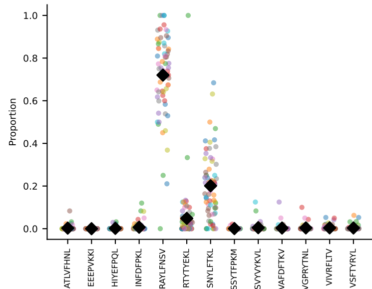
#18 AV10N-CAASRASGSWQLIF-AJ22_BV16-CASSLTGEGNTLYF-BJ1-3 coh=0.497, n=6
