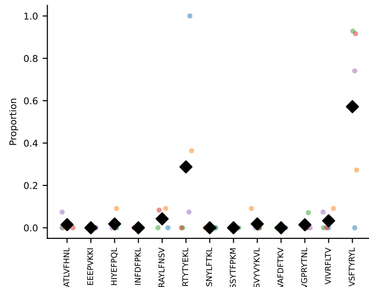
#17 AV12D-3-CALSGENSGTYQRF-AJ13_BV12-2-CASSLAGVYQDTQYF-BJ2-5 coh=0.558, n=5
