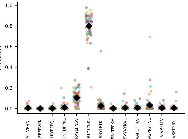
#84 AV16N-CAMRDTNAYKVIF-AJ30_BV13-2-CASGGANTEVFF-BJ1-1 coh=0.949, n=69
