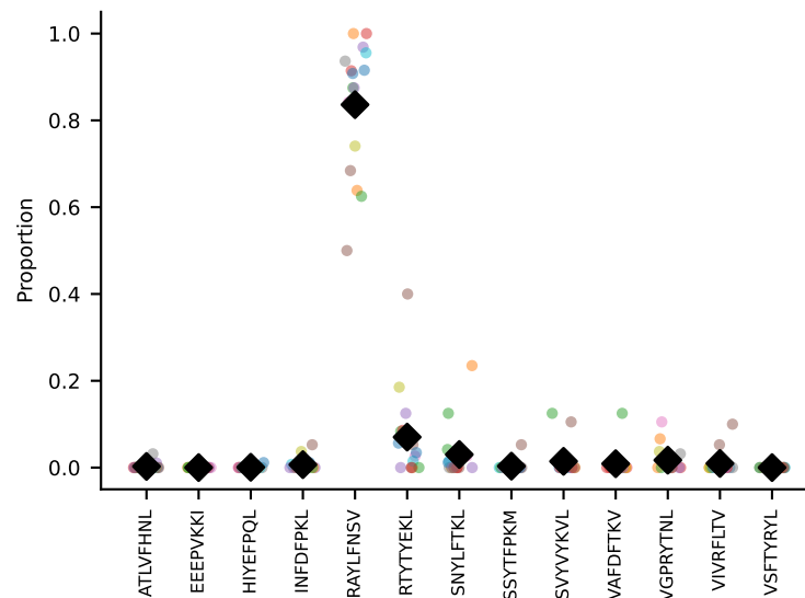
#83 AV4-2-CAVEGTGGYKVVF-AJ12_BV13-1-CASSAGADSPLYF-BJ1-6 coh=0.950, n=13
