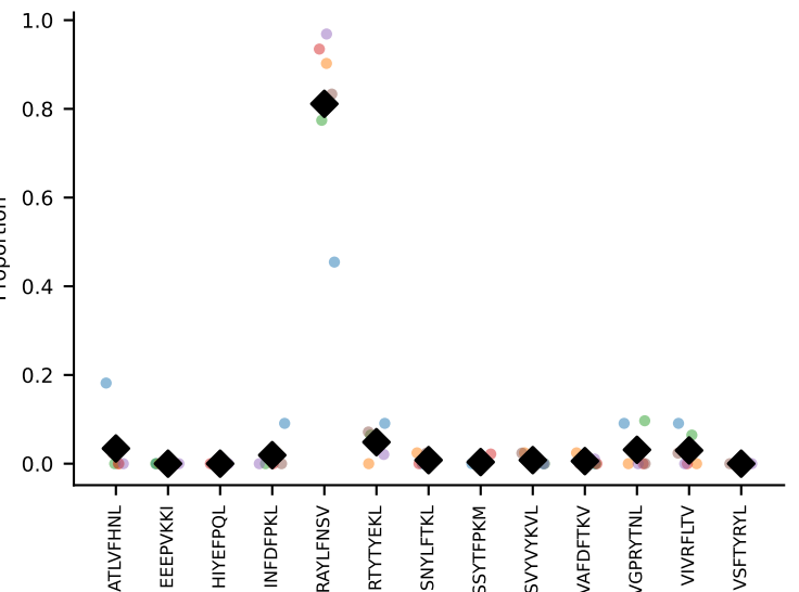
#80 AV10-CAASMTNSAGNKLTf-AJ17_BV26-CASRDWGQDTQYF-BJ2-5 coh=0.954, n=28
