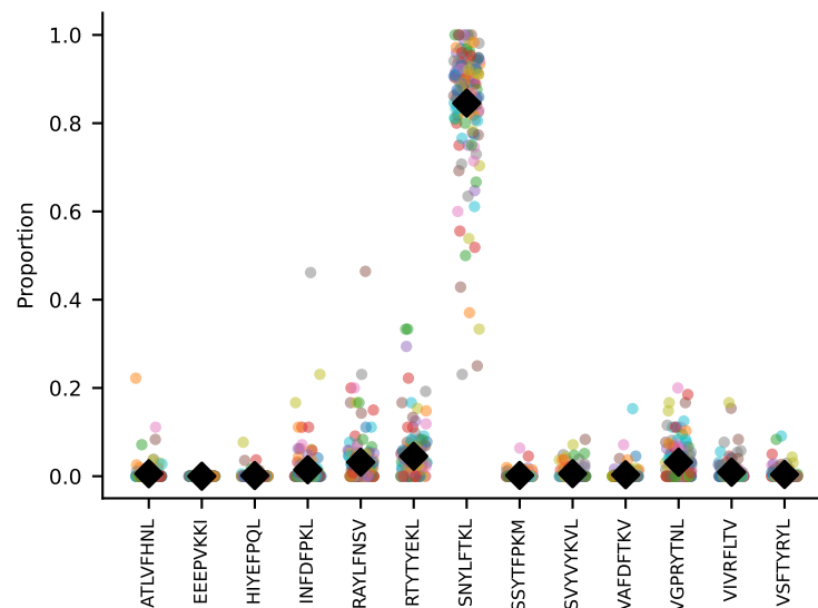
#79 AV16-CAMREDSNYQLIW-AJ33_BV3-CASSSGQISNERLFF-BJ1-4 coh=0.955, n=16
