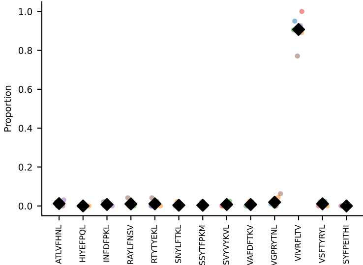
#95 AV16/DV11-CAMREDTGYNFYF-AJ49_BV13-1-CASGGVYEYF-BJ2-1 coh=0.996, n=12
