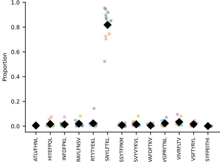
#45 AV13D-3-CAMRTNSAGNKLTF-AJ17*p02_BV13-2-CASGTTYEQYF-BJ2-7 coh=0.984, n=11
