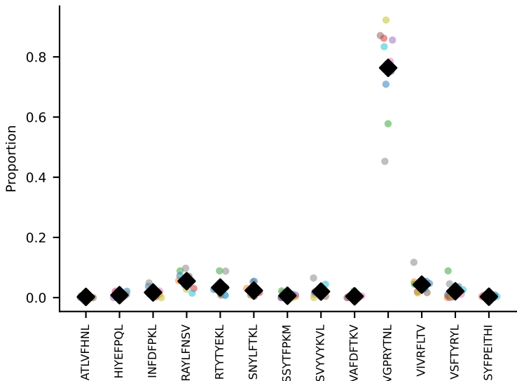
#49 AV16D/DV11-CAMREDTNTGKLTF-AJ27_BV13-1-CASSDGANSDYTF-BJ2-7 coh=0.981, n=6
