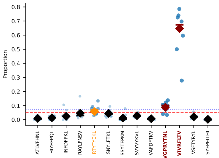
#109 AV3-3-CAVMPNYNVLYF-AJ21*p03_BV13-2-CASGDLGTNNQAPLF-BJ1-5 DUAL | Above BG: VGPRYTNL+VIVRFLTV n=8 [HTxB:8] thresh=0.075
