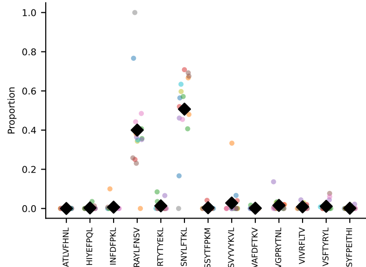
#85 AV5-1-CSASSGSWQLIF-AJ22_BV13-2-CASGEVGSNTEVFF-BJ1-1#86 AV16D/DV11-CAMREVTGANTGKLTF-AJ52_BV1-CTCSVDRIQDTQYF-BJ2-6 coh=0.829, n=25
