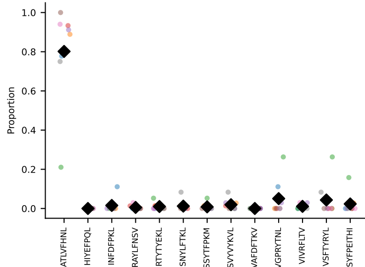
#83 AV5-1-CSASSGSWQLIF-AJ22_BV13-2-CASGEVGSNTEVFF-BJ1-1#84 AV16D/DV11-CAMREVTGANTGKLTF-AJ52_BV1-CTCSVDRIQDTQYF-BJ2-6 coh=0.830, n=6
