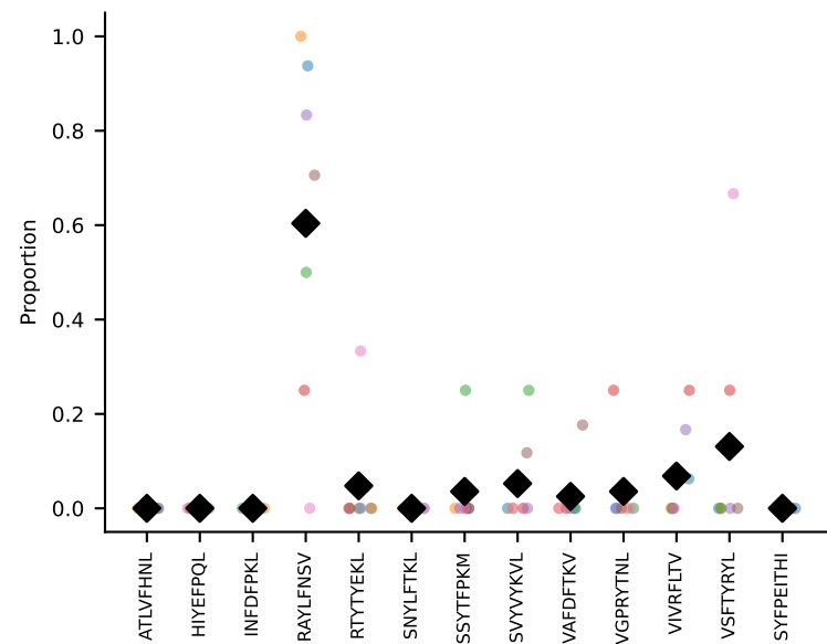
#100 AV16/DV11-CAMREAGYQNIFYF-AJ49_BV4-CEGDRNNSPLYF-BJ1-6 coh=0.574, n=7
