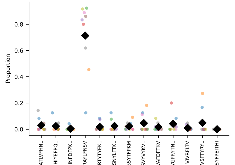
#95 AV16D/DV11-CAMREVTGANTGKLTF-AJ52_BV1-CTCSVDRIQDTQYF-BJ2-6#96 AV16D/DV11-CAMREVTGANTGKLTF-AJ52_BV1-CTCSVDRIQDTQYF-BJ2-6 coh=0.794, n=6
