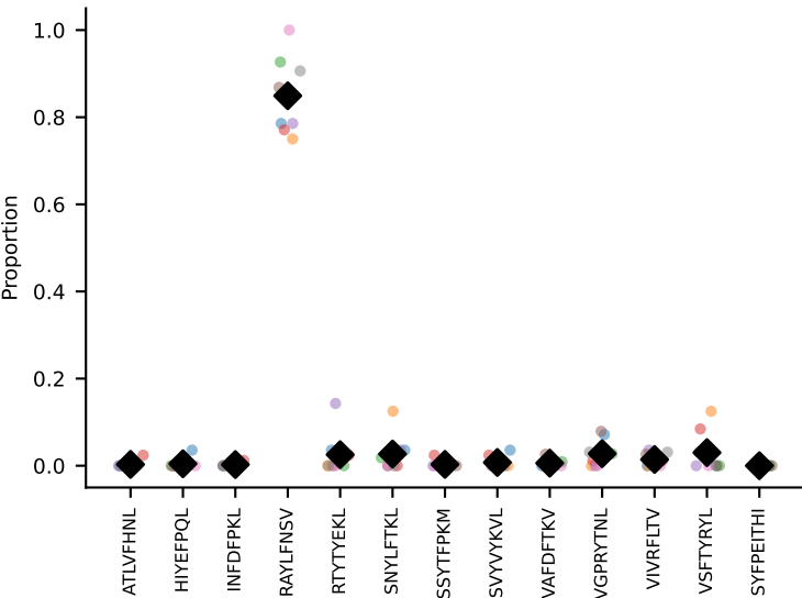
#31 AV16D/DV11-CAMREGSSGSWQLIF-AJ22_BV13-1-CASSDVGDEYQF-BJ2-7 coh=0.983, n=8
