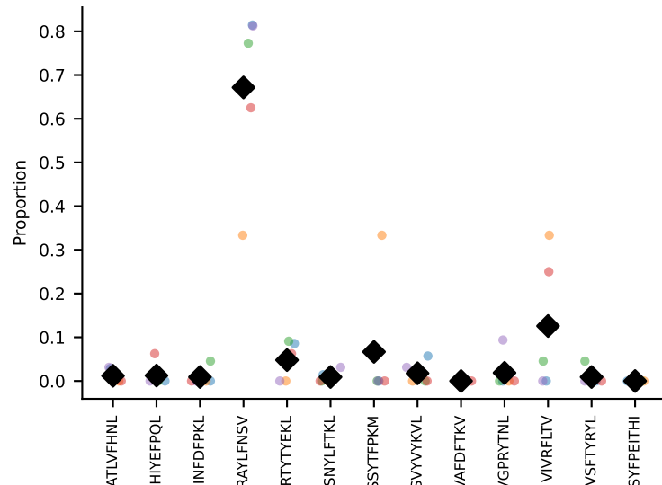
#91 AV5-1-CSASSGSWQLIF-AJ22_BV13-2-CASGEVGSNTEVFF-BJ1-1#92 AV16D/DV11-CAMREVTGANTGKLTF-AJ52_BV1-CTCSVDRIQDTQYF-BJ2-6 coh=0.823, n=5
