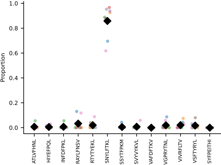
#35 AV7-3-CASPNTGYQNIFY-AJ49_BV13-2-CASGGWGSQNTLYF-BJ2-4 coh=0.977, n=15
