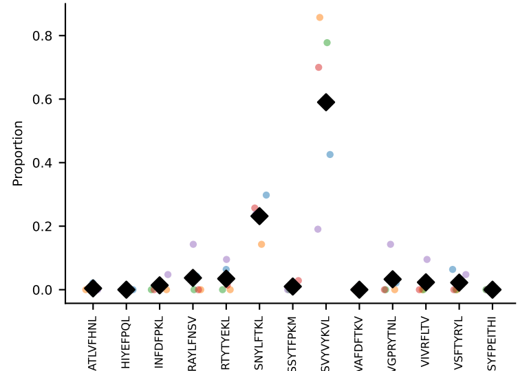
#87 AV16/DV11-CAMREVTGANTGKLTF-AJ52_BV1-CTCSVDRIQDTQYF-BJ2-6#88 AV16/DV11-CAMREVTGANTGKLTF-AJ52_BV1-CTCSVDRIQDTQYF-BJ2-6 coh=0.823, n=9
