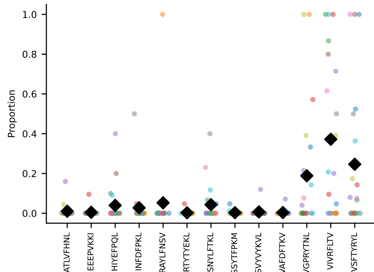
#47 AV12-1-CALRDYSNNRLTL-AJ7_BV3-CASSPGVDTQYF-BJ2-5 coh=0.354, n=13
