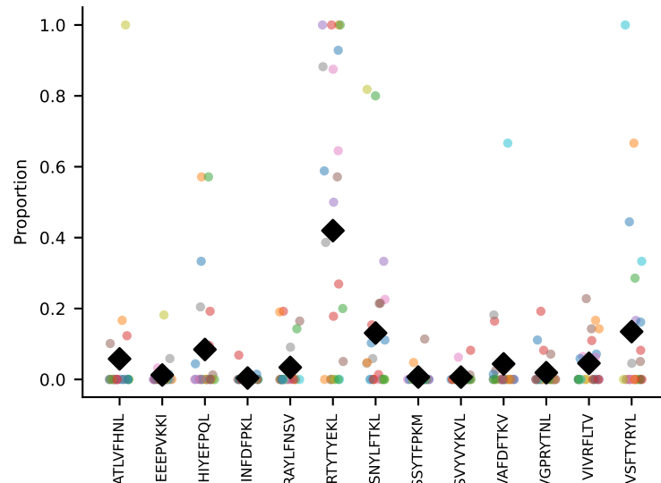
#35 AV16-CAMREGYGNKITf-AJ48_BV30-CSSREGQNTLYF-BJ2-4 coh=0.383, n=24
