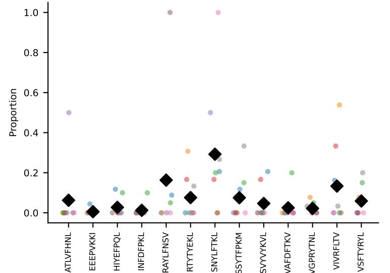
#60 AV6-6-CALGEDGSSGNKLIF-AJ32_BV13-3-CASRQGARTVEVFF-BJ1-1 coh=0.328, n=8
