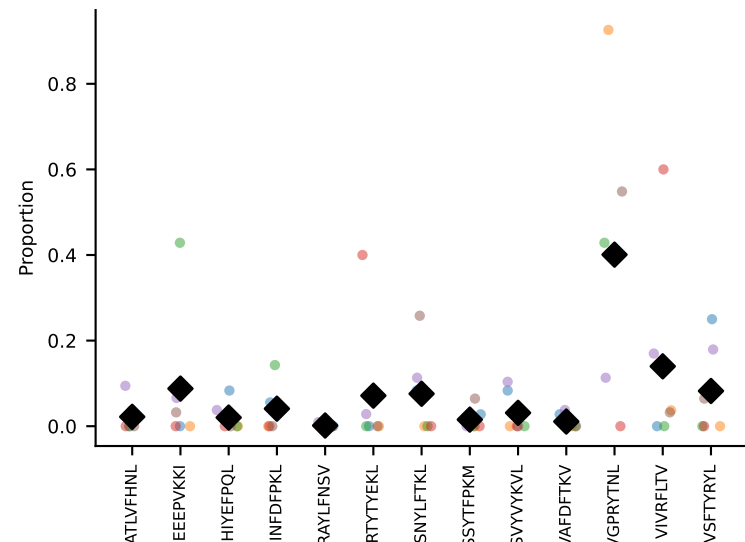
#21 AV19-CAAGADYANKMIF-AJ47_BV3-CASSPGPQNTLYF-BJ2-4 coh=0.462, n=6
