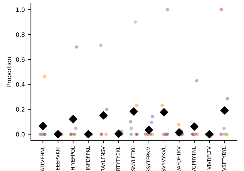
#156 AV14D-1-CAARNTGADRLTF-AJ45_BV29-CASSWGN YAEQFF-BJ2-2 coh=0.031, n=6
