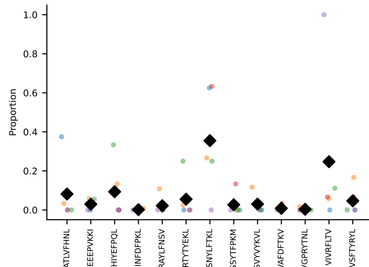
#24 AV12-1-CALSETGNTGKLIF-AJ37_BV13-2-CASGDAGTNTTEVFF-BJ1-1 coh=0.427, n=5
