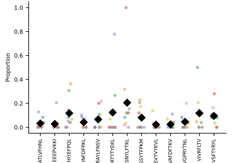
#56 AV13-2-CAIDTNTGKLTf-AJ27_BV13-2-CASGDVNTVEVFF-BJ1-1 coh=0.333, n=8
