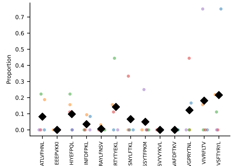
#104 AV14-2-CAASASSGSWQLIF-AJ22_BV31-CAWSLQGSQNTLYF-BJ1-3 coh=0.234, n=17
