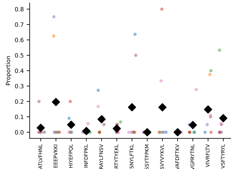
#137 AV8D-2-CATDTGGLSGKLTf-AJ2_BV13-1-CASSPGQYAEQFF-BJ2-1 coh=0.175, n=36
