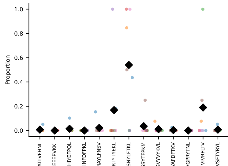
#22 AV19-CAAGGSGGKLT-AJ44_BV13-1-CASSDLTGAPNERLFF-BJ1-4 coh=0.455, n=7
