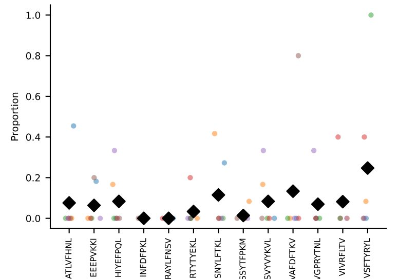
#152 AV9-1-CAVSADGSSGNKLIF-AJ32_BV1-CTCSAVRINTEVFF-BJ1-1 coh=0.120, n=7
