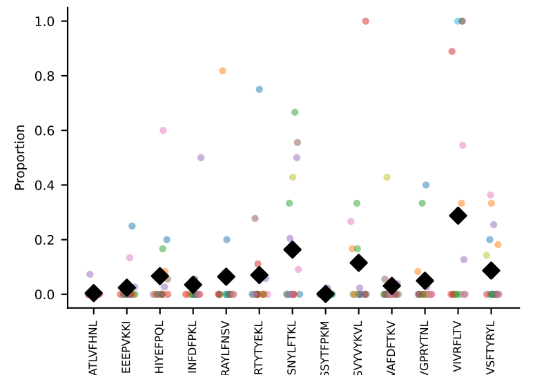
#108 AV14-3-CAATNSAGNKLTf-AJ17_BV26-CASSLTLSGNTLYF-BJ1-3 coh=0.226, n=5
