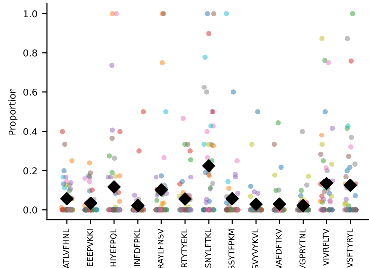
#70 AV7-5-CAVGGSGGKLTL-AJ44_BV4-CASSLGRHTEVFF-BJ1-1 coh=0.298, n=48
