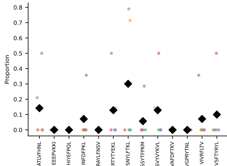
#151 AV13-1-CAFNNAGAKLTF-AJ39_BV3-CASSYRDWGV EYQF-BJ2-7 coh=0.121, n=6
