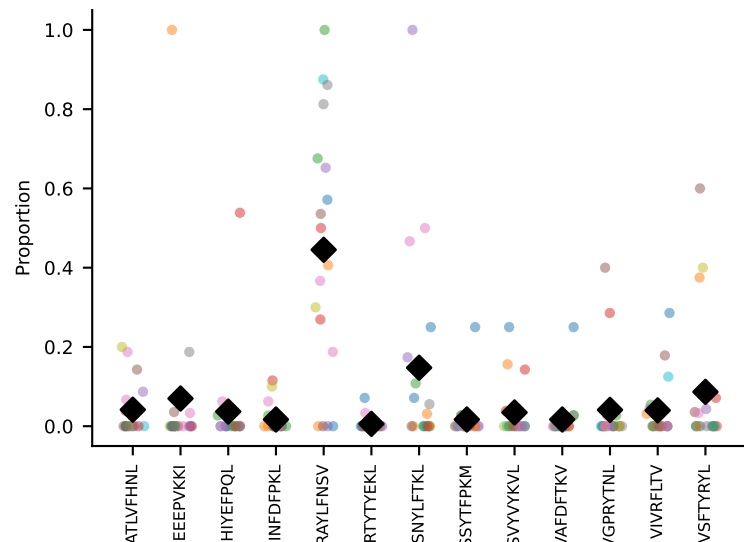
#23 AV16N-CAMREGNSGT YQRF-AJ13_BV3-CASSLGQAPNSDYTF-BJ1-2 coh=0.446, n=18
