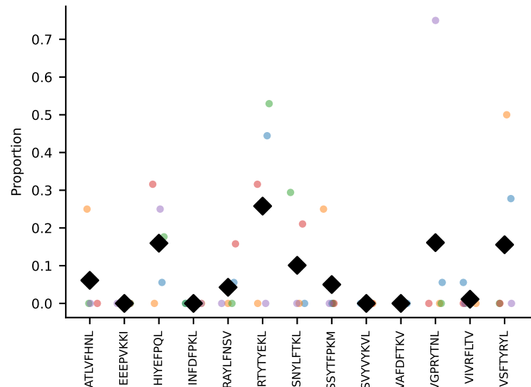
#71 AV3-1-CAVSAGDYAQLTF-AJ26_BV26-CASSLSRGDGTVEFF-BJ1-1 coh=0.298, n=6
