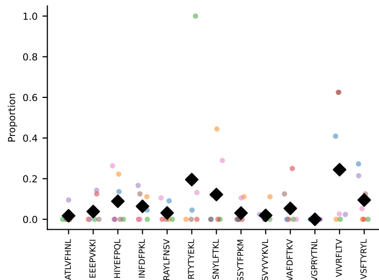
#67 AV6N-6-CALSATSSGQKLVF-AJ16_BV23-CSSSQSQTNTNEVFF-BJ1-1 coh=0.296, n=39
