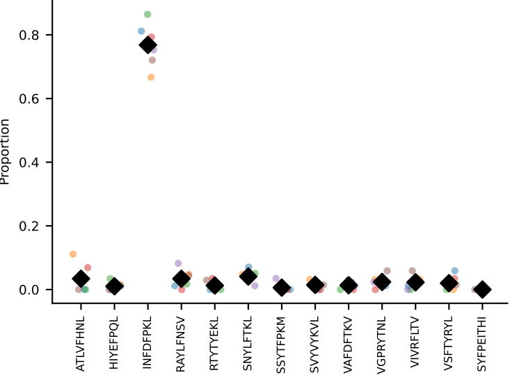
#71 AV16/DV11-CAMREHNTNTGKLTF-AJ27_BV1-CTCSADRVGNTLYF-BJ1-1 coh=0.988, n=10
