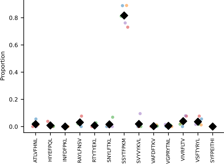
#69 AV6-6-CALGDHTGYQNIFYF-AJ49_BV13-3-CASSENRVNTEVFF-BJ1-1 coh=0.989, n=5
