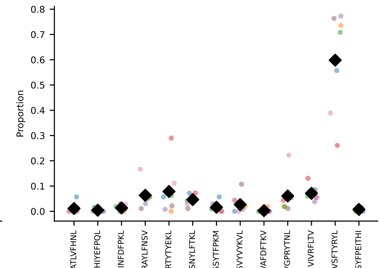
#192 AV8D-2-CATEANSPTYQRF-AJ13_BV3-CASSPPGGGDTQYF-BJ2-5 coh=0.860, n=14
