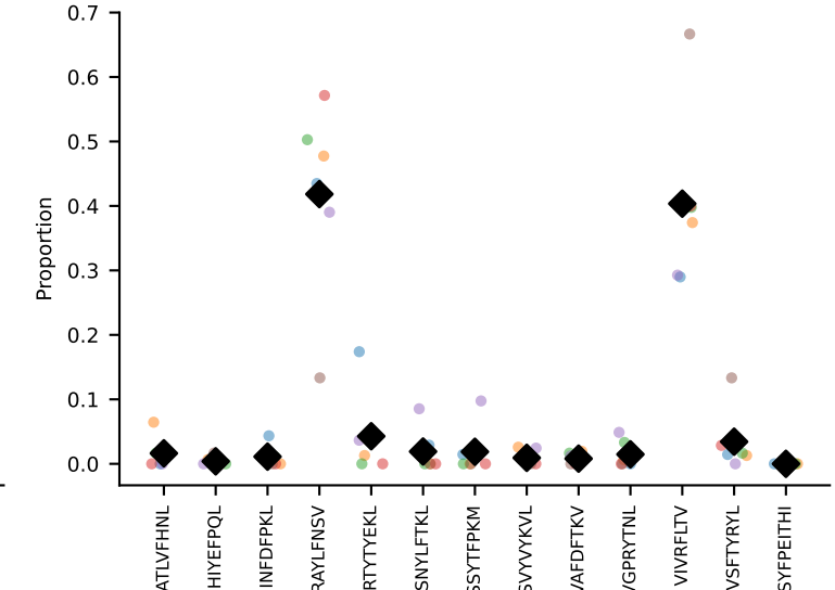
#188 AV8-1-CATDGGSAALGRLHF-AJ18_BV1-CTCSADPETETLYF-BJ2-3 coh=0.868, n=7
