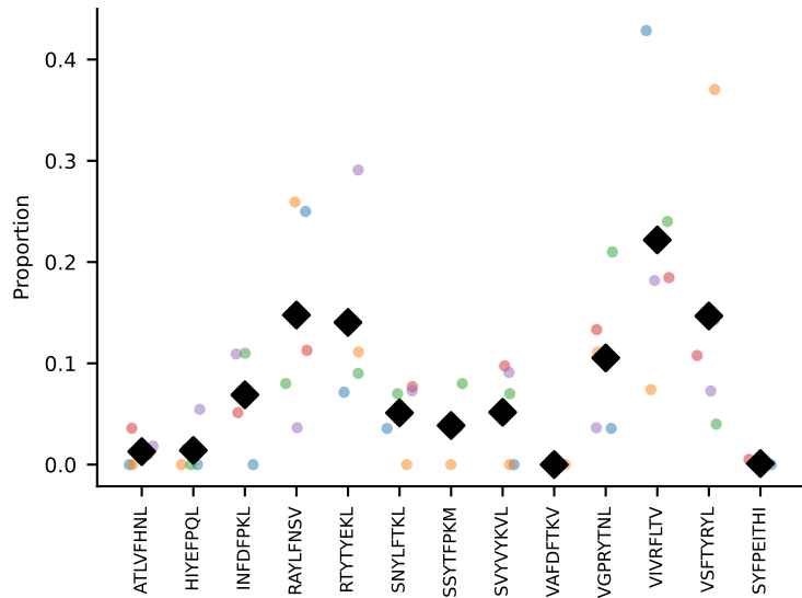
#240 AV6-5-CALSDGGTGSKLSF-AJ58_BV17-CASSPGLGGRFNEQYF-BJ2-1 coh=0.693, n=5
