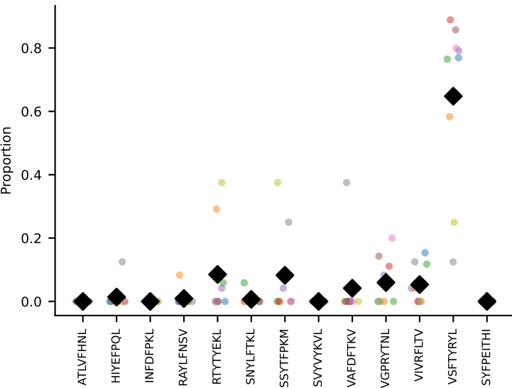
#237 AV4-3-CAADQGGRALIF-AJ15_BV13-2-CASGWAPLGDYEQYF-BJ2-7 coh=0.713, n=9
